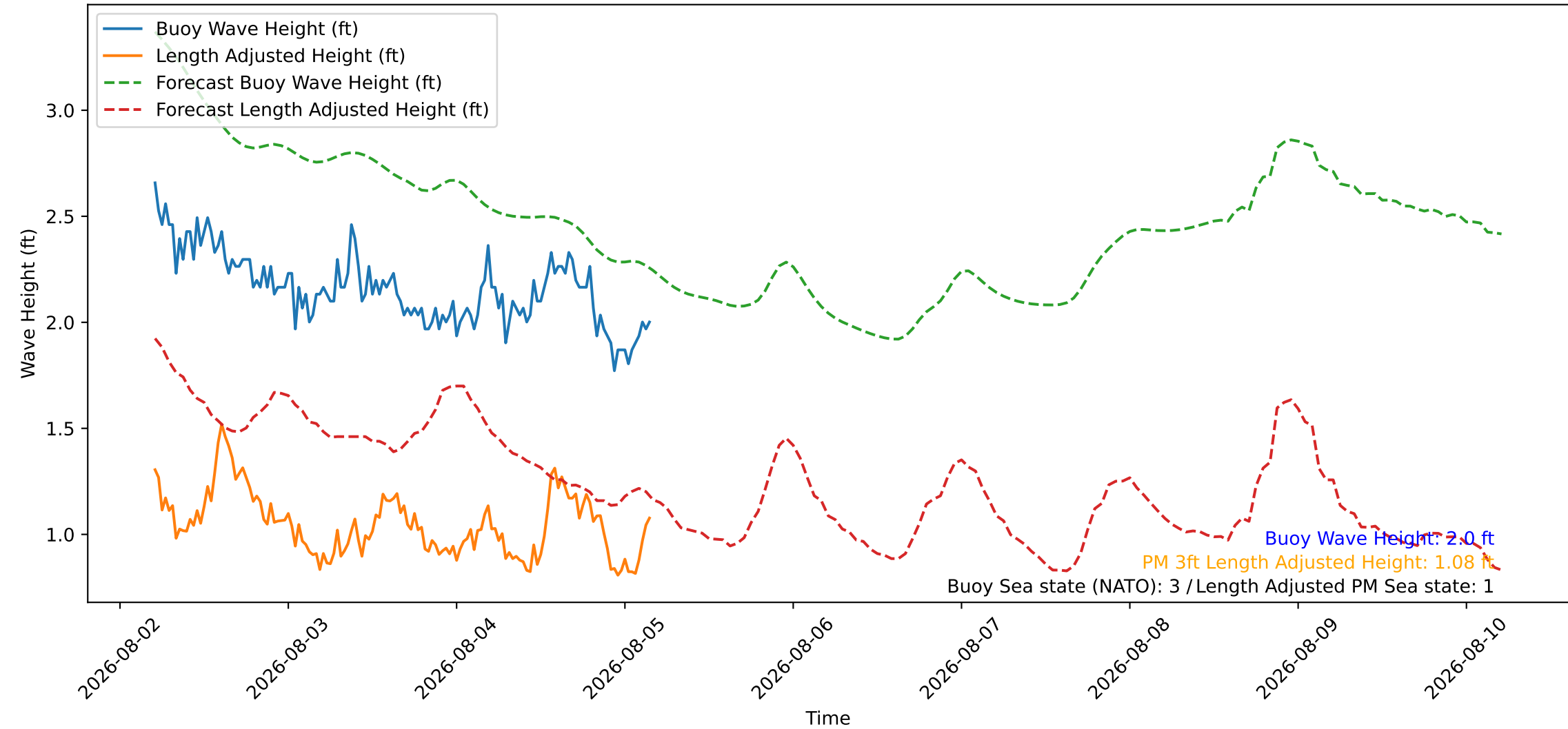
Wave Heights over Time for Red Beach at 2026-08-05 04:40:47
