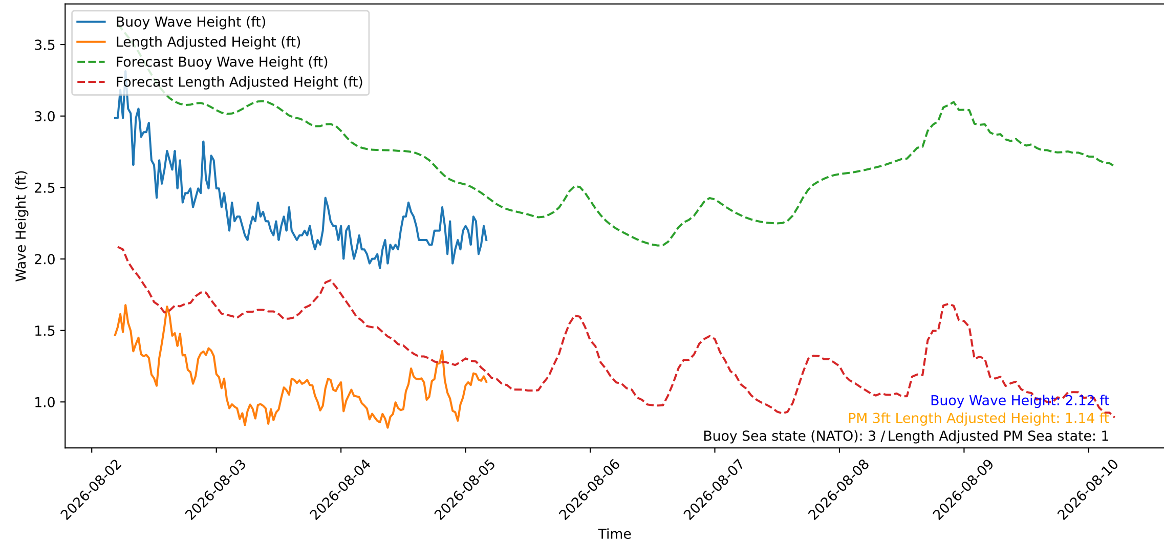
Wave Heights over Time for Green Beach at 2026-08-05 04:41:09
