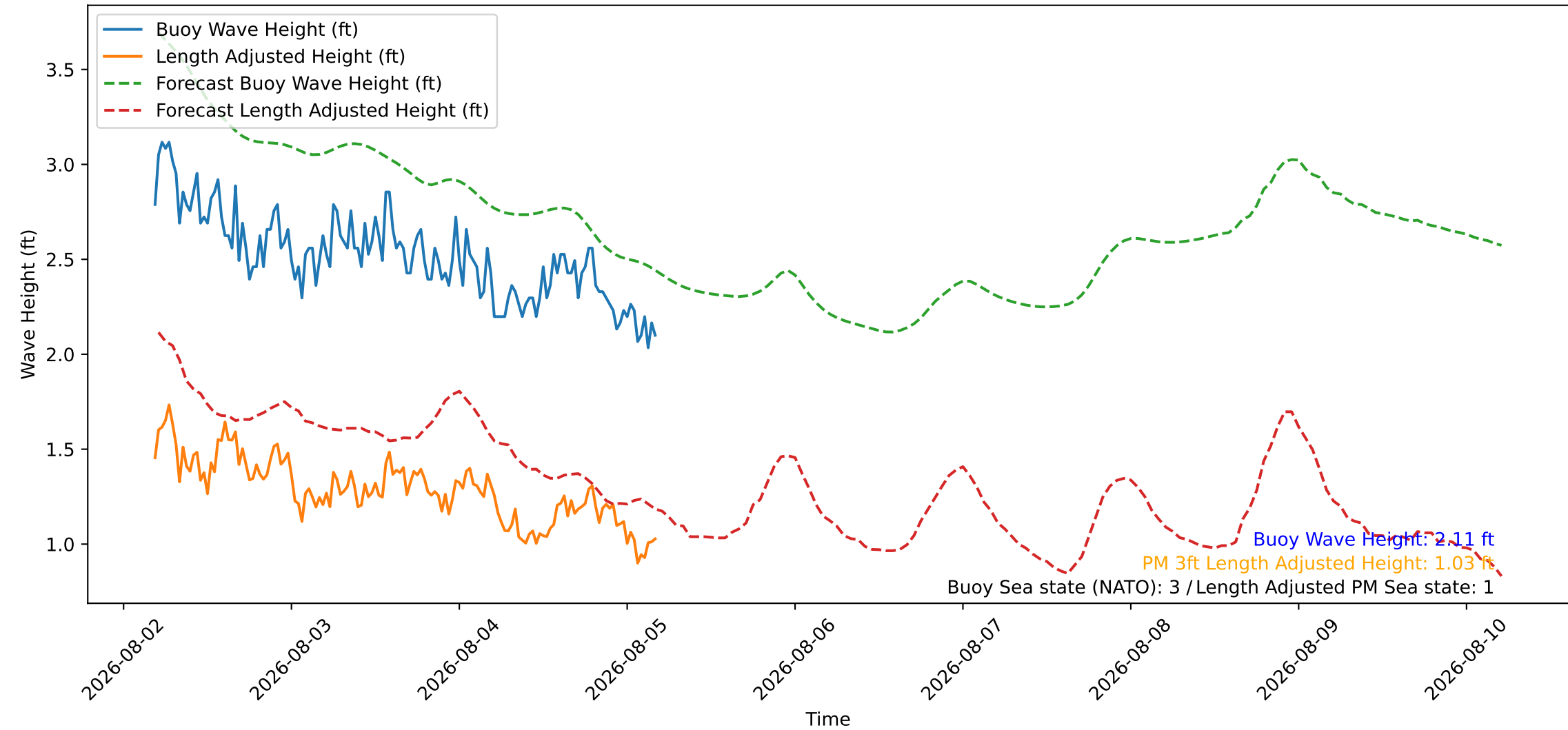
Wave Heights over Time for Oceanside Harbor at 2026-08-05 04:40:26
