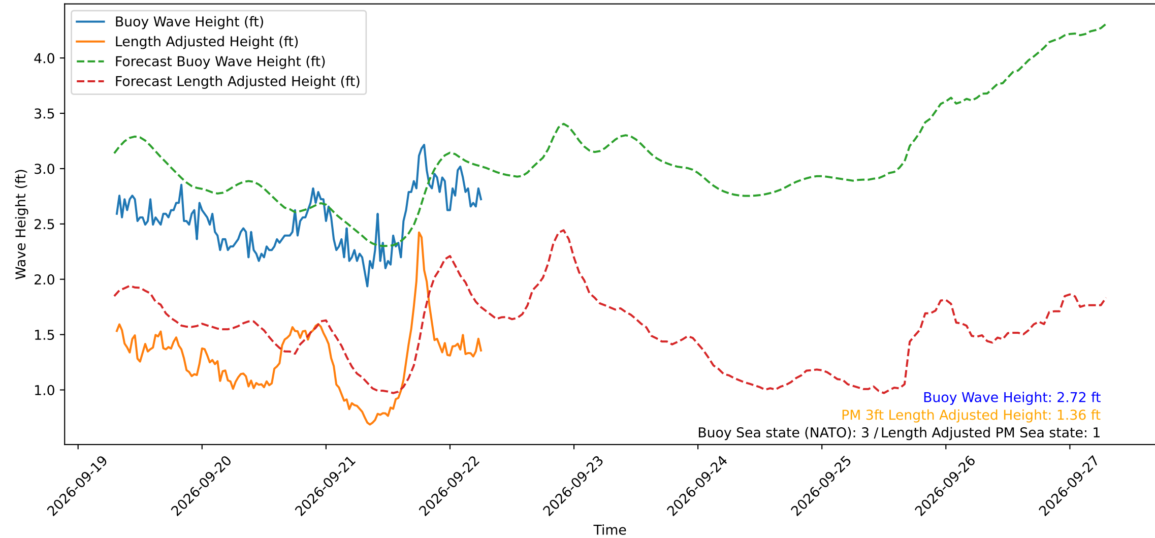
Wave Heights over Time for Green Beach at 2026-09-22 07:01:12
