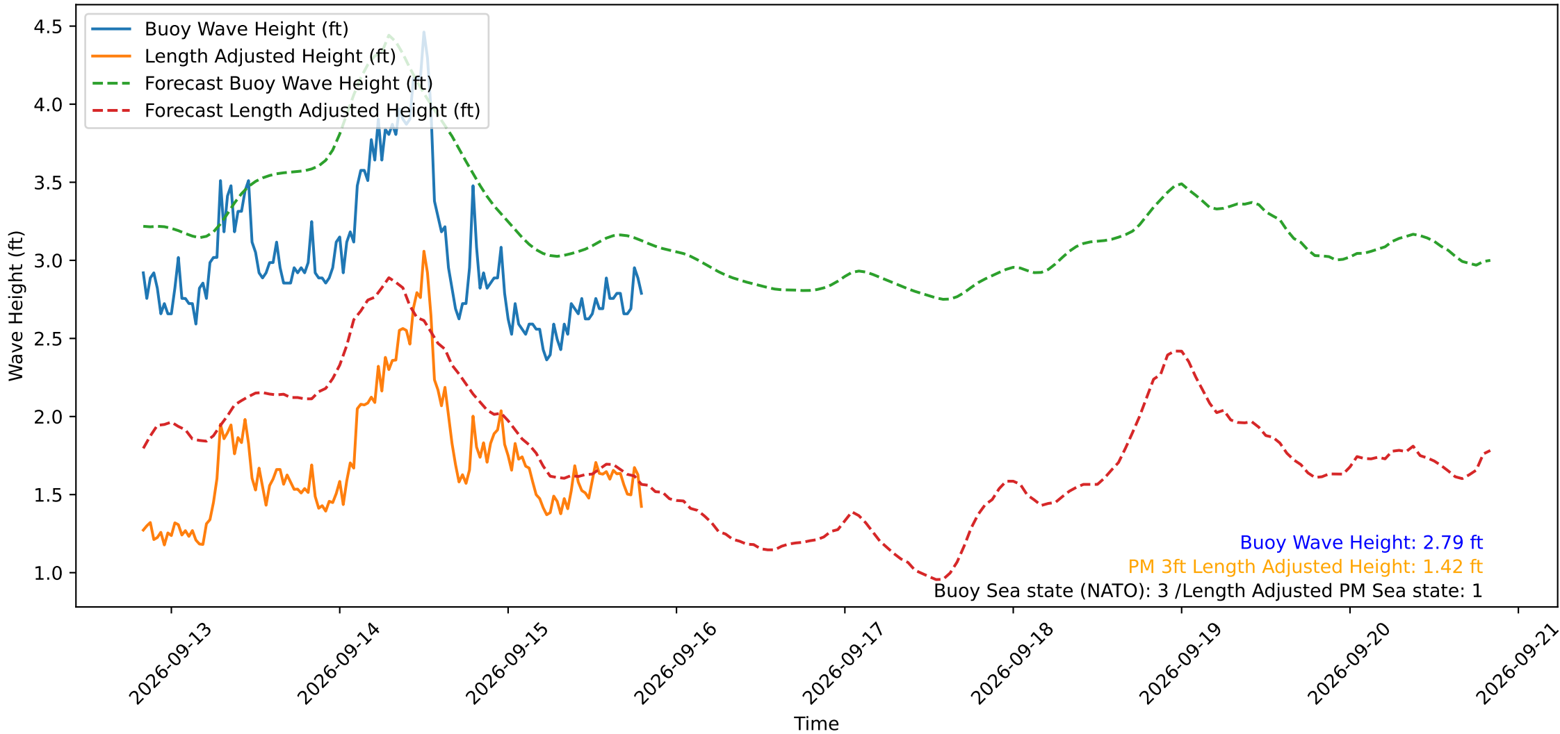
Wave Heights over Time for Oceanside Harbor at 2026-09-15 19:50:30
