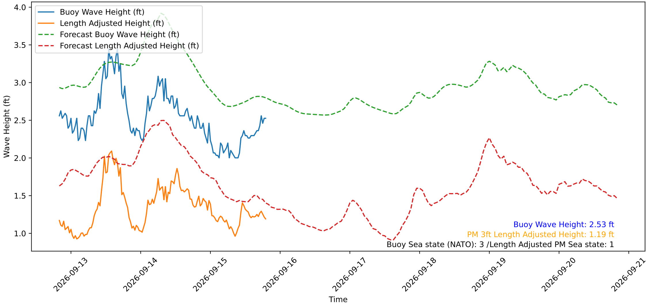
Wave Heights over Time for Red Beach at 2026-09-15 19:50:51
