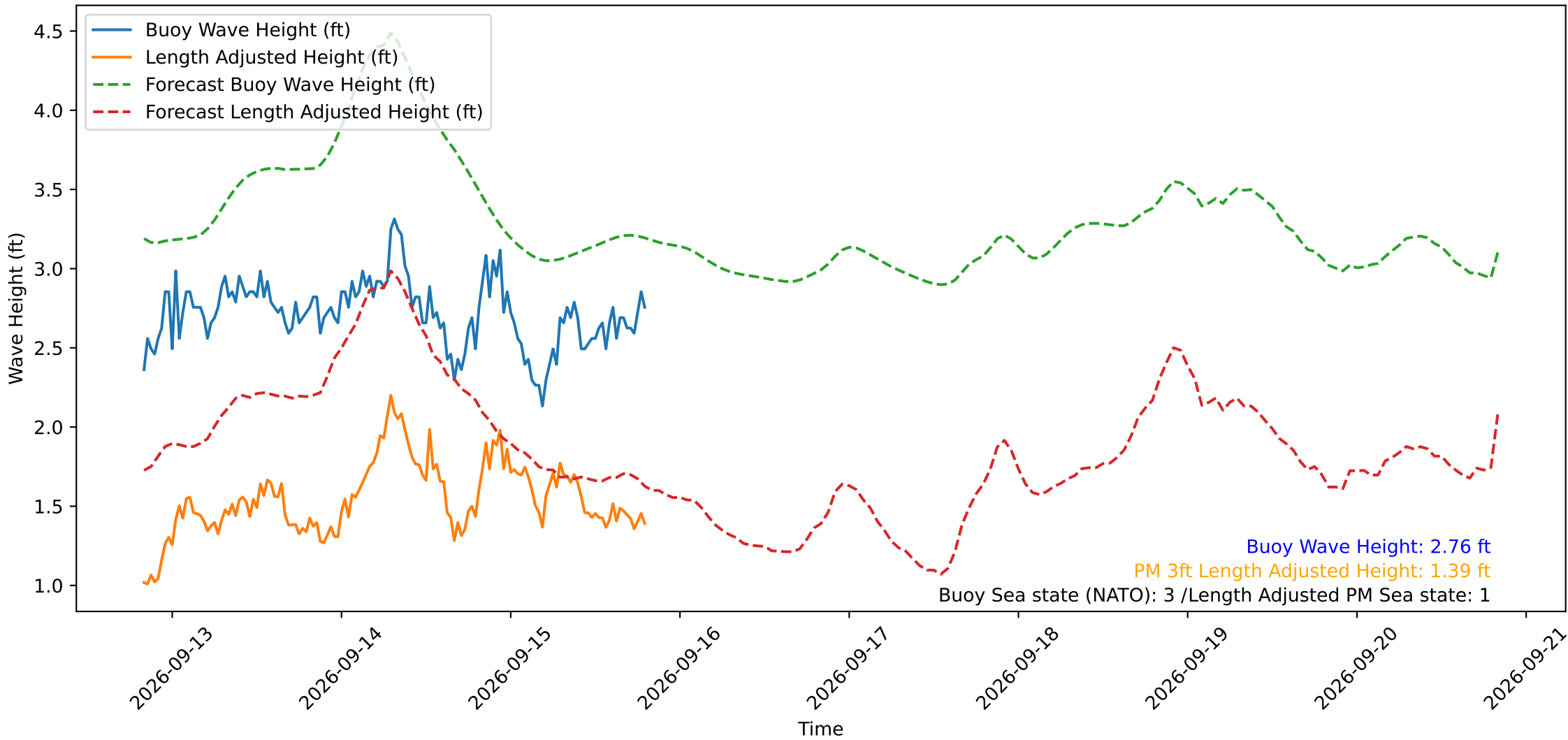
Wave Heights over Time for Green Beach at 2026-09-15 19:51:15
