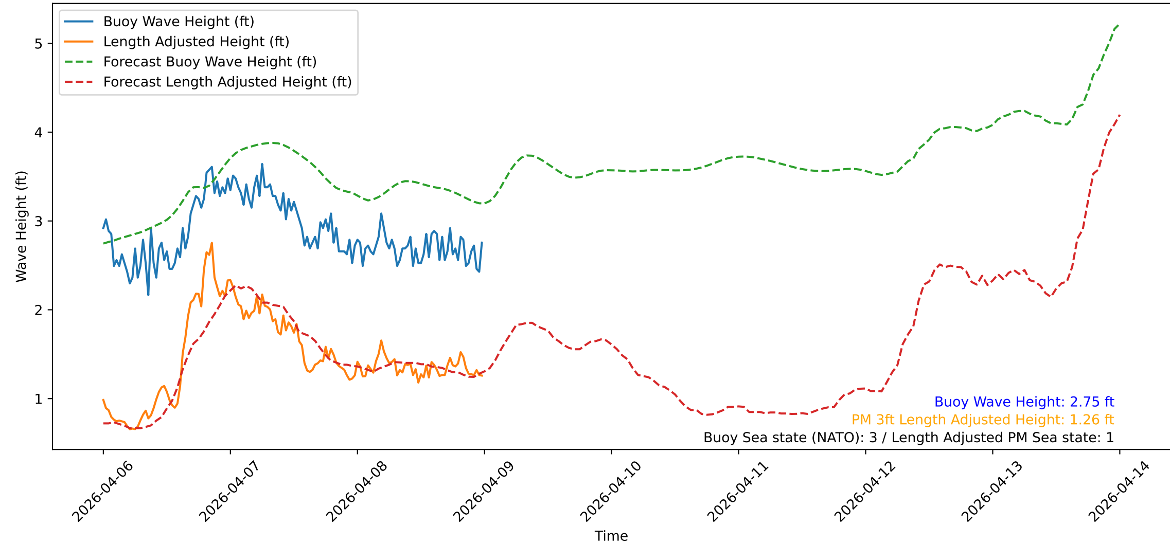
Wave Heights over Time for Oceanside Harbor at 2026-04-09 00:10:31
