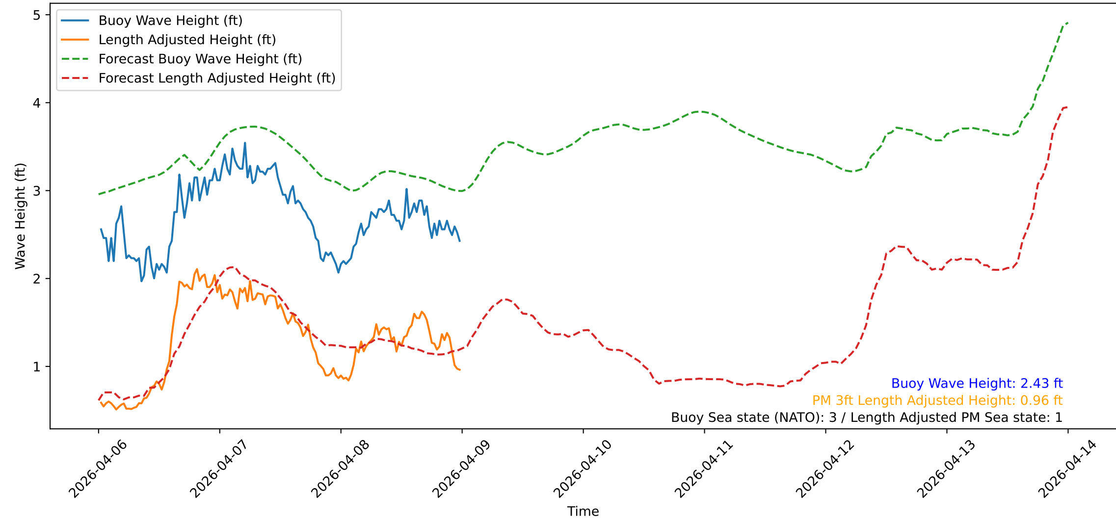
Wave Heights over Time for Red Beach at 2026-04-09 00:10:47
