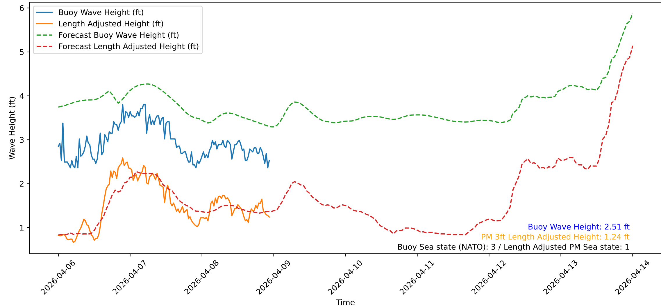
Wave Heights over Time for Green Beach at 2026-04-09 00:11:09
