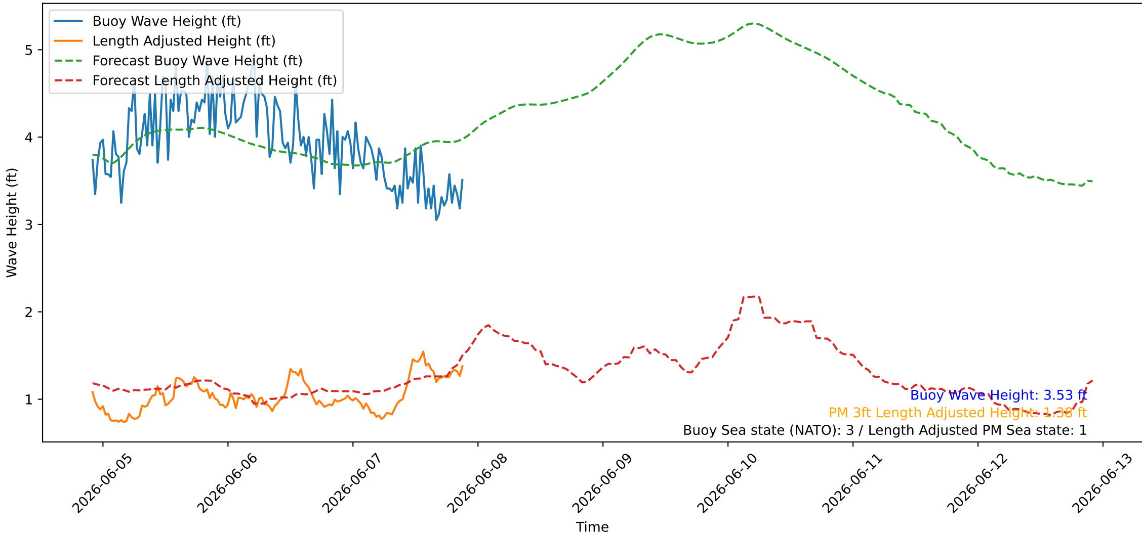
Wave Heights over Time for Red Beach at 2026-06-07 21:50:47
