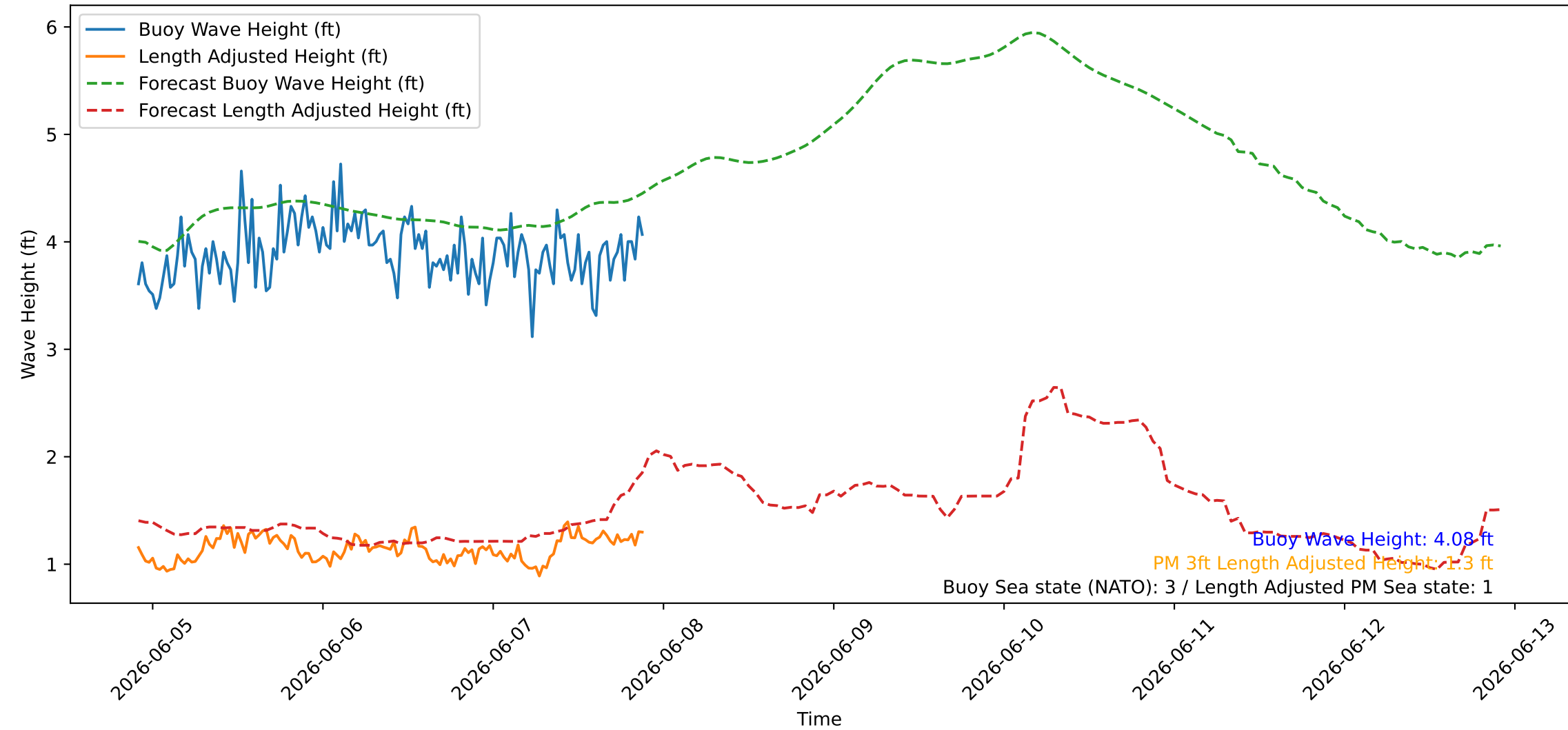
Wave Heights over Time for Green Beach at 2026-06-07 21:51:09
