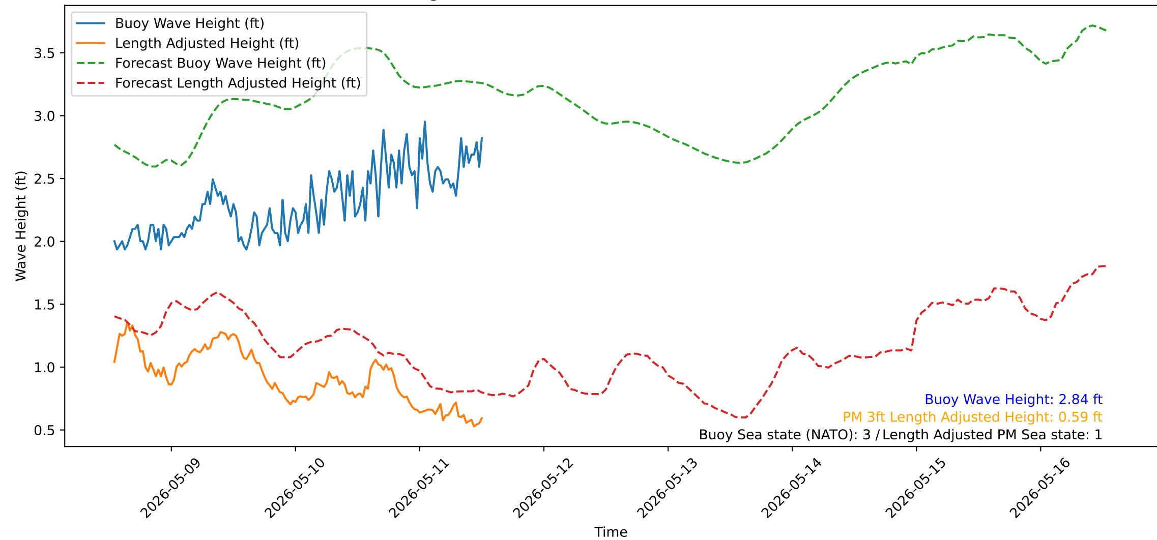
Wave Heights over Time for Red Beach at 2026-05-11 12:40:50
