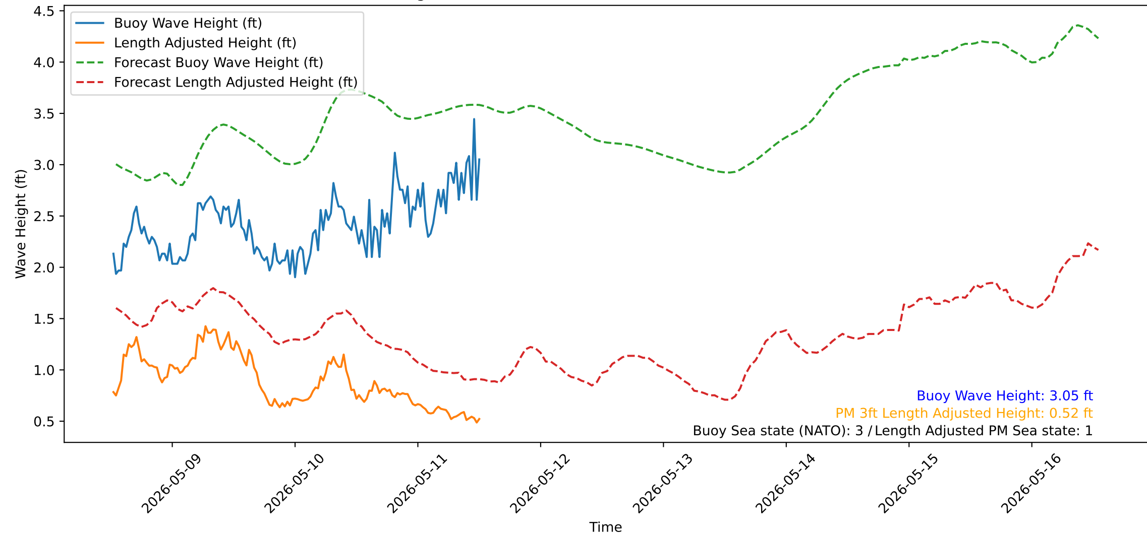
Wave Heights over Time for Green Beach at 2026-05-11 12:41:13
