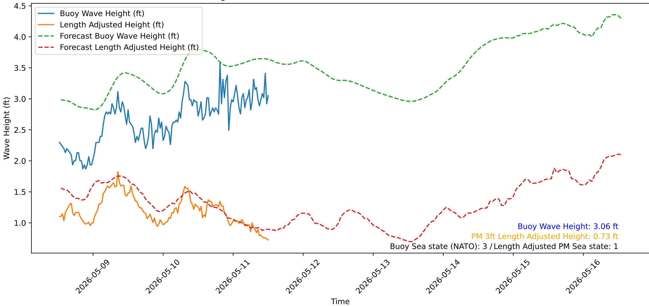
Wave Heights over Time for Oceanside Harbor at 2026-05-11 12:40:31
