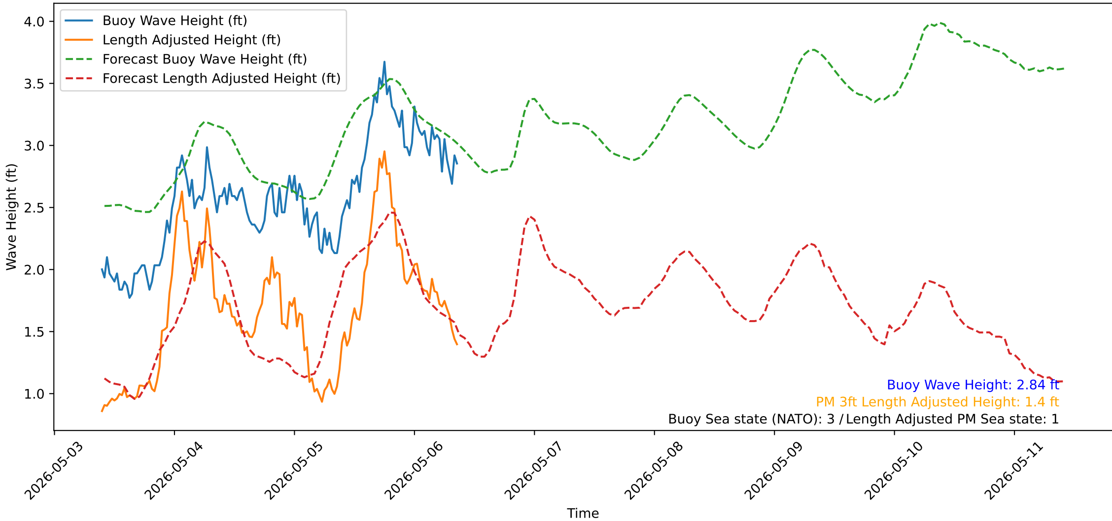
Wave Heights over Time for Green Beach at 2026-05-06 09:31:13
