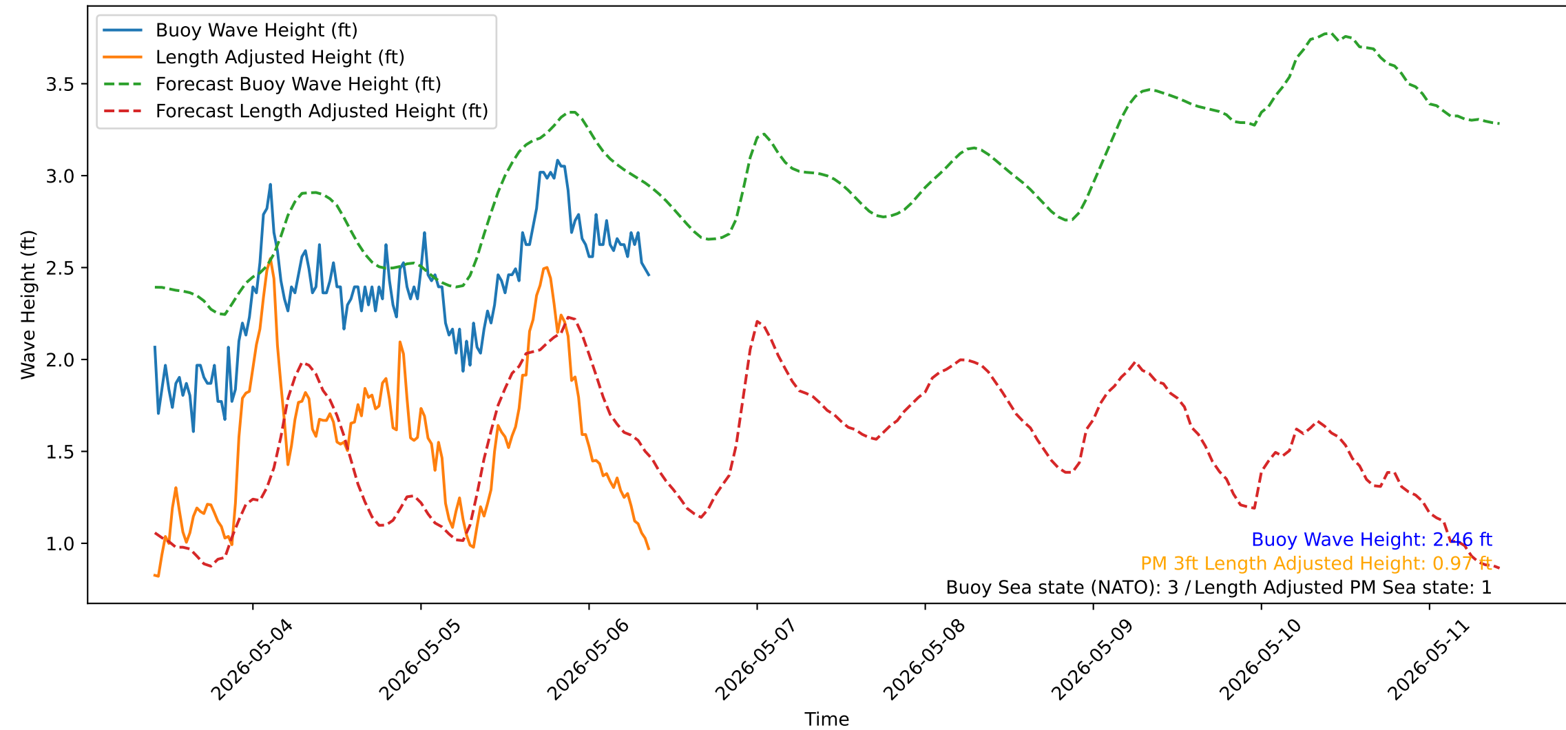
Wave Heights over Time for Red Beach at 2026-05-06 09:30:50
