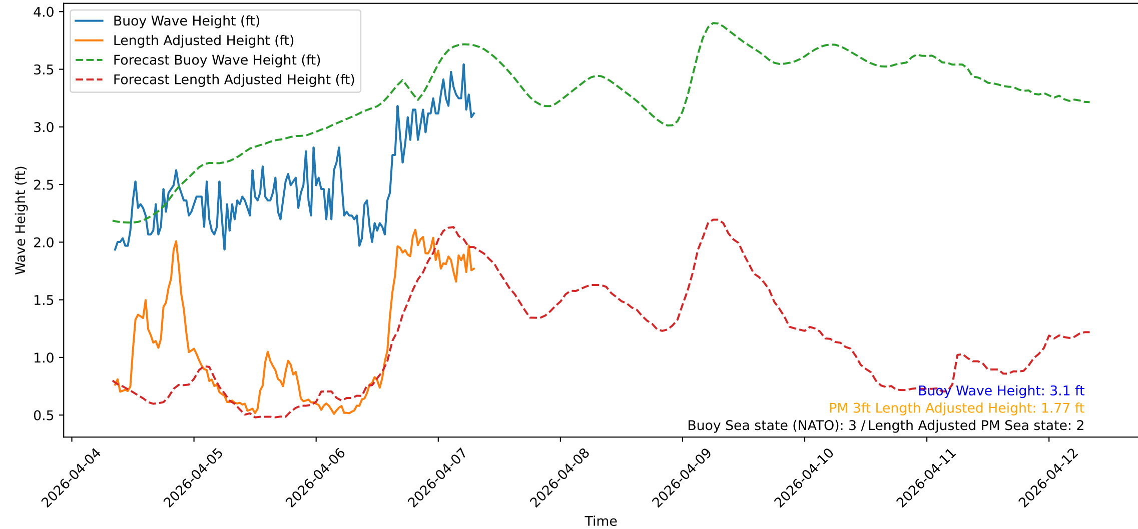
Wave Heights over Time for Red Beach at 2026-04-07 08:00:48
