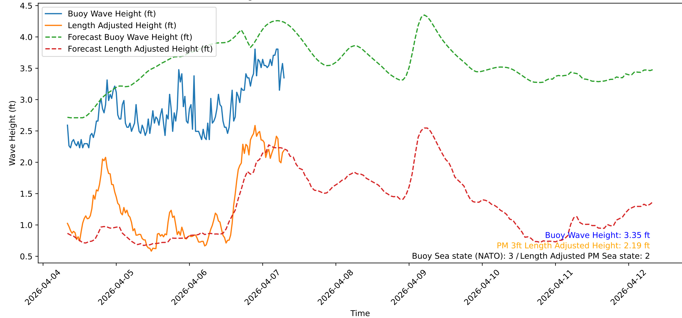
Wave Heights over Time for Green Beach at 2026-04-07 08:01:10
