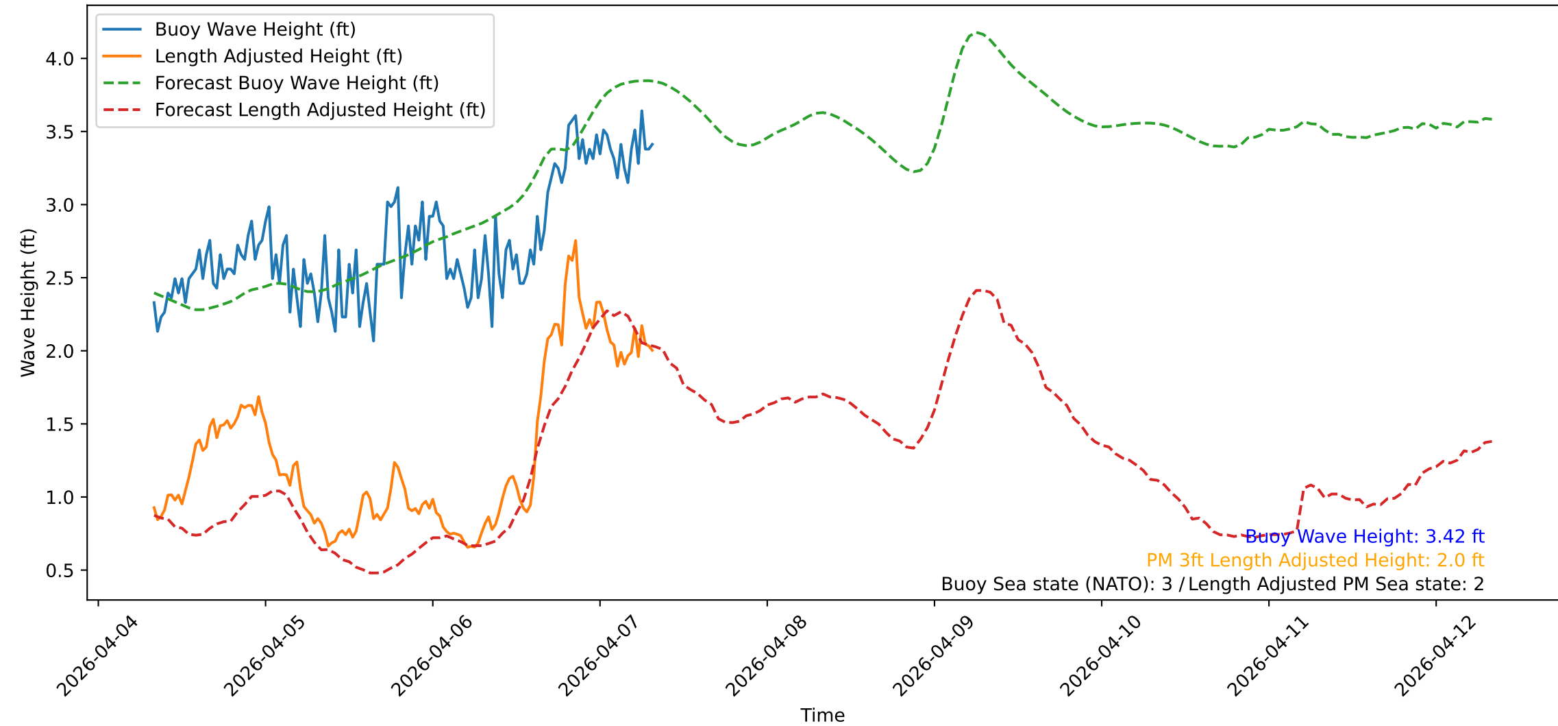
Wave Heights over Time for Oceanside Harbor at 2026-04-07 08:00:32
