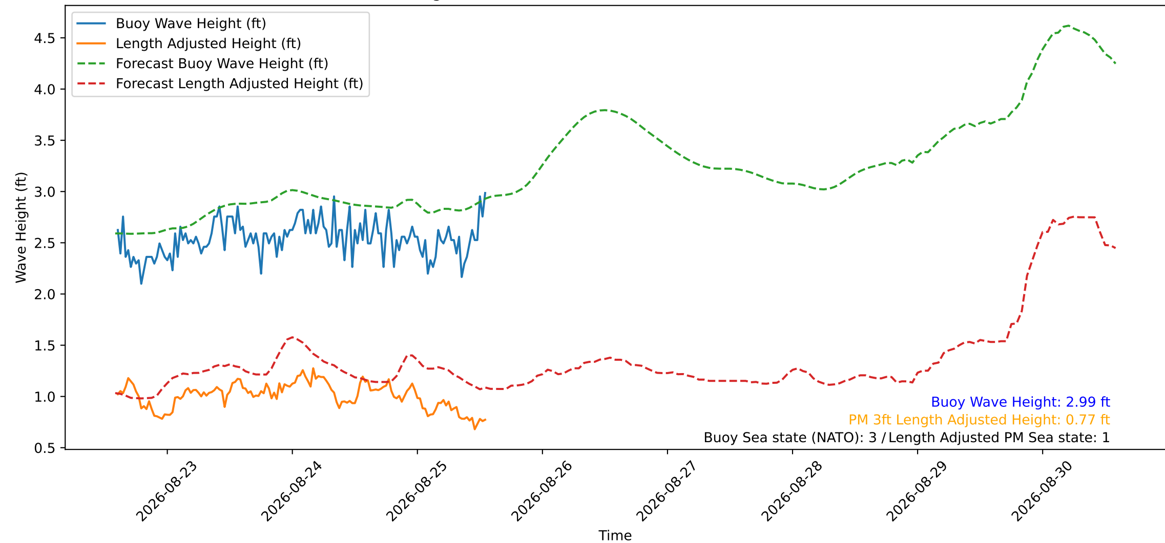
Wave Heights over Time for Red Beach at 2026-08-25 14:00:49
