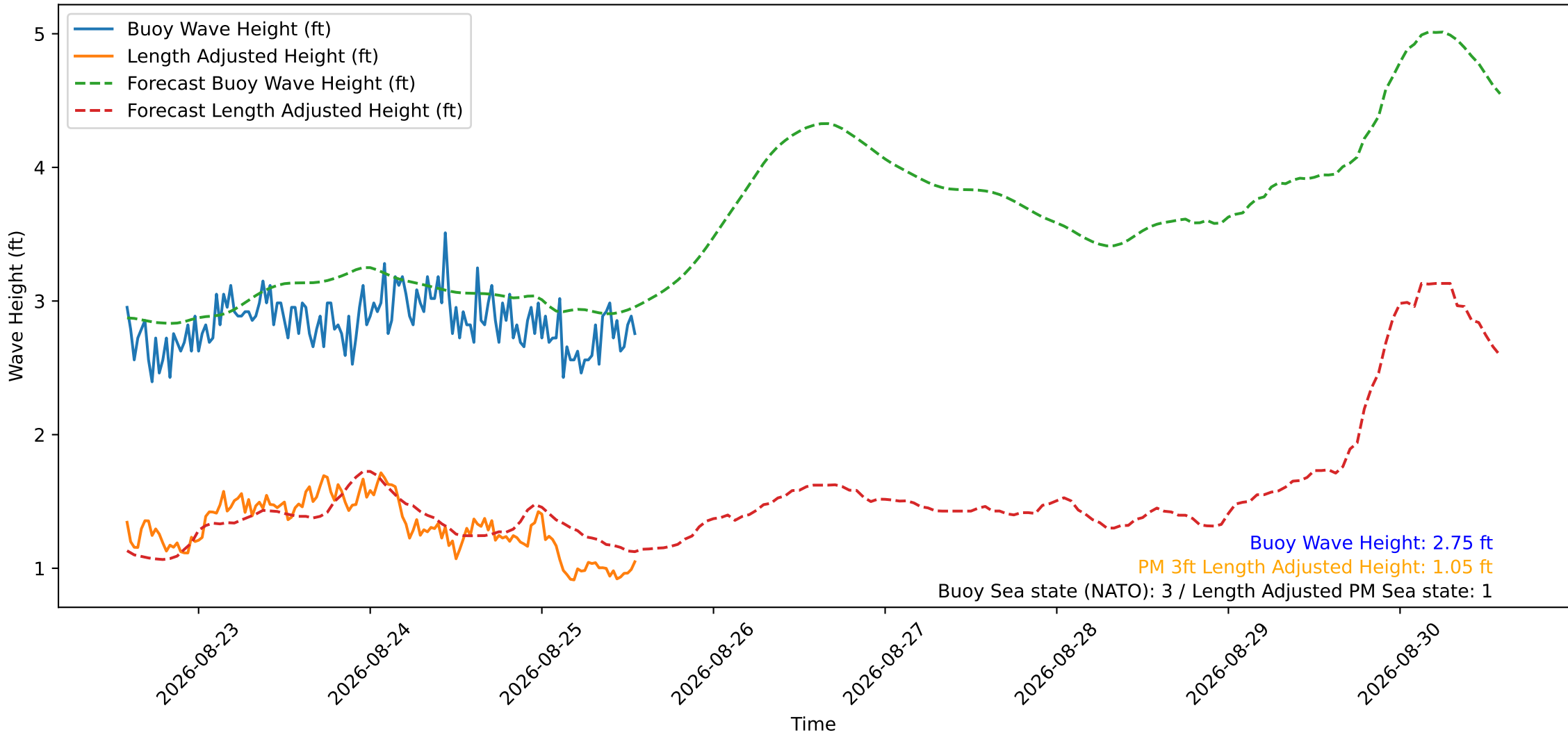
Wave Heights over Time for Oceanside Harbor at 2026-08-25 14:00:29
