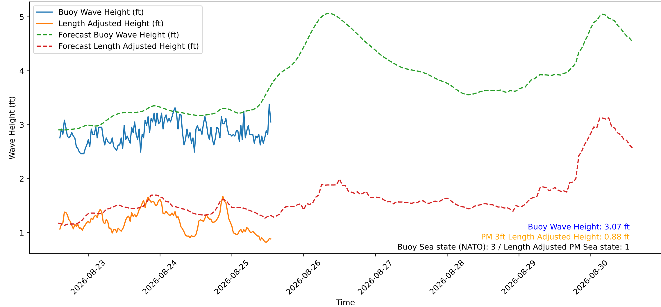
Wave Heights over Time for Green Beach at 2026-08-25 14:01:12
