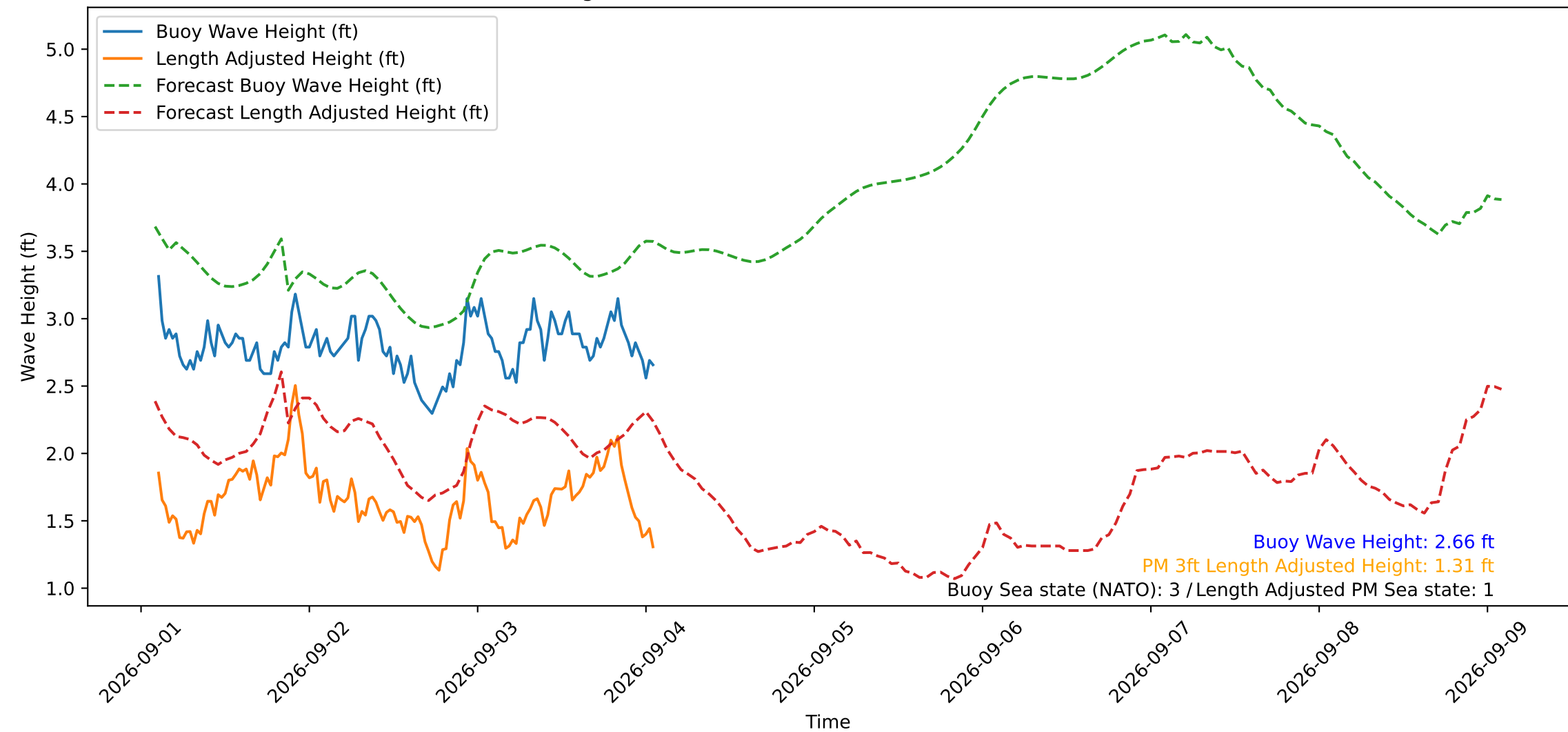
Wave Heights over Time for Red Beach at 2026-09-04 02:00:49
