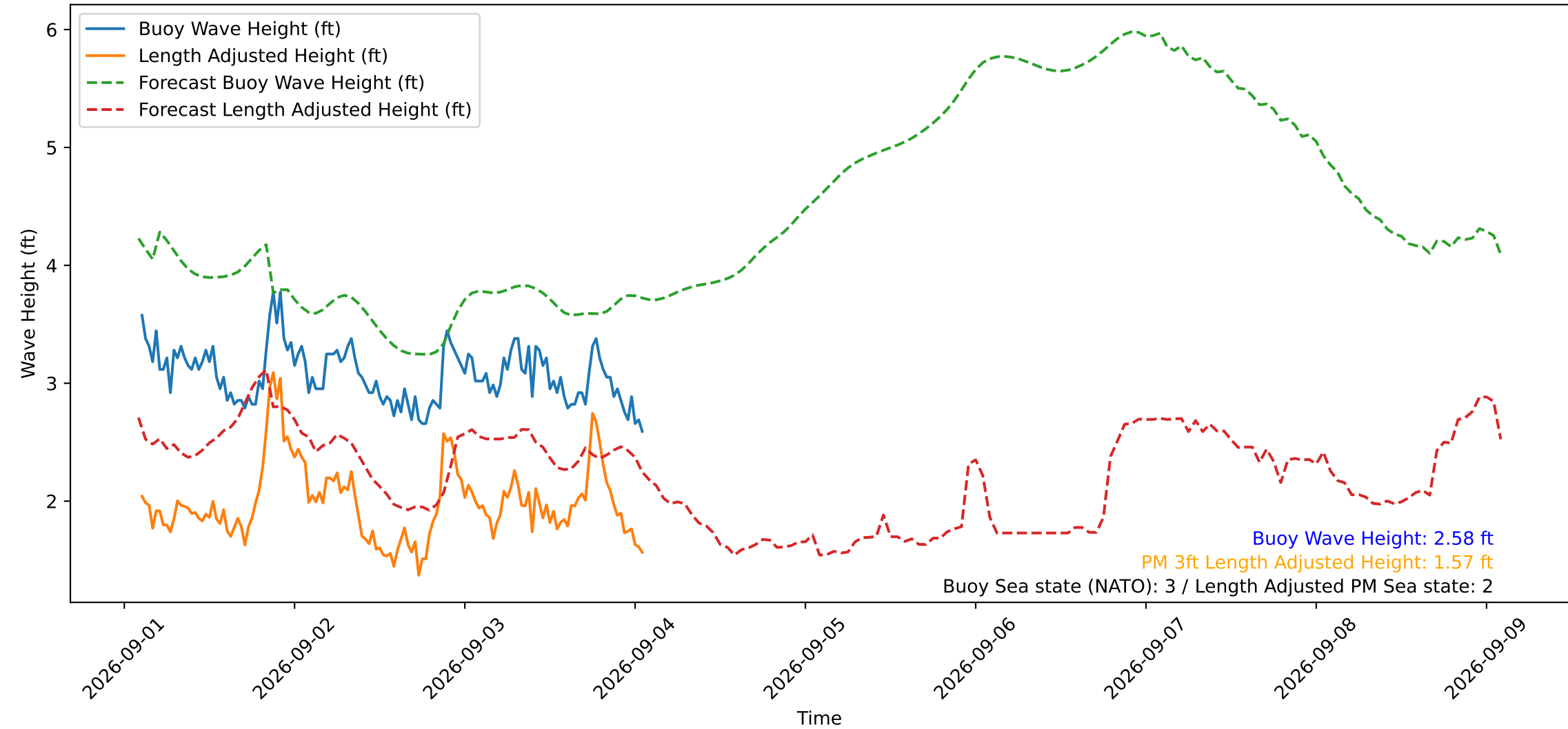
Wave Heights over Time for Green Beach at 2026-09-04 02:01:12
