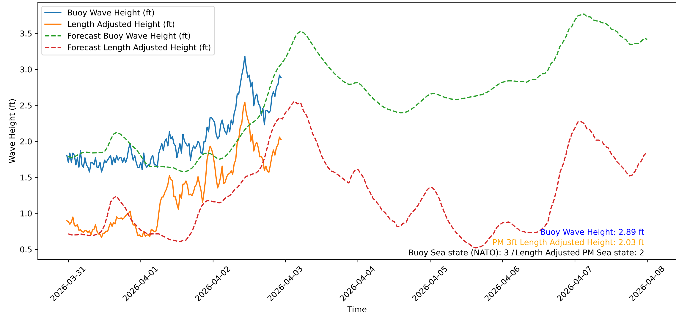
Wave Heights over Time for Oceanside Harbor at 2026-04-02 23:40:31
