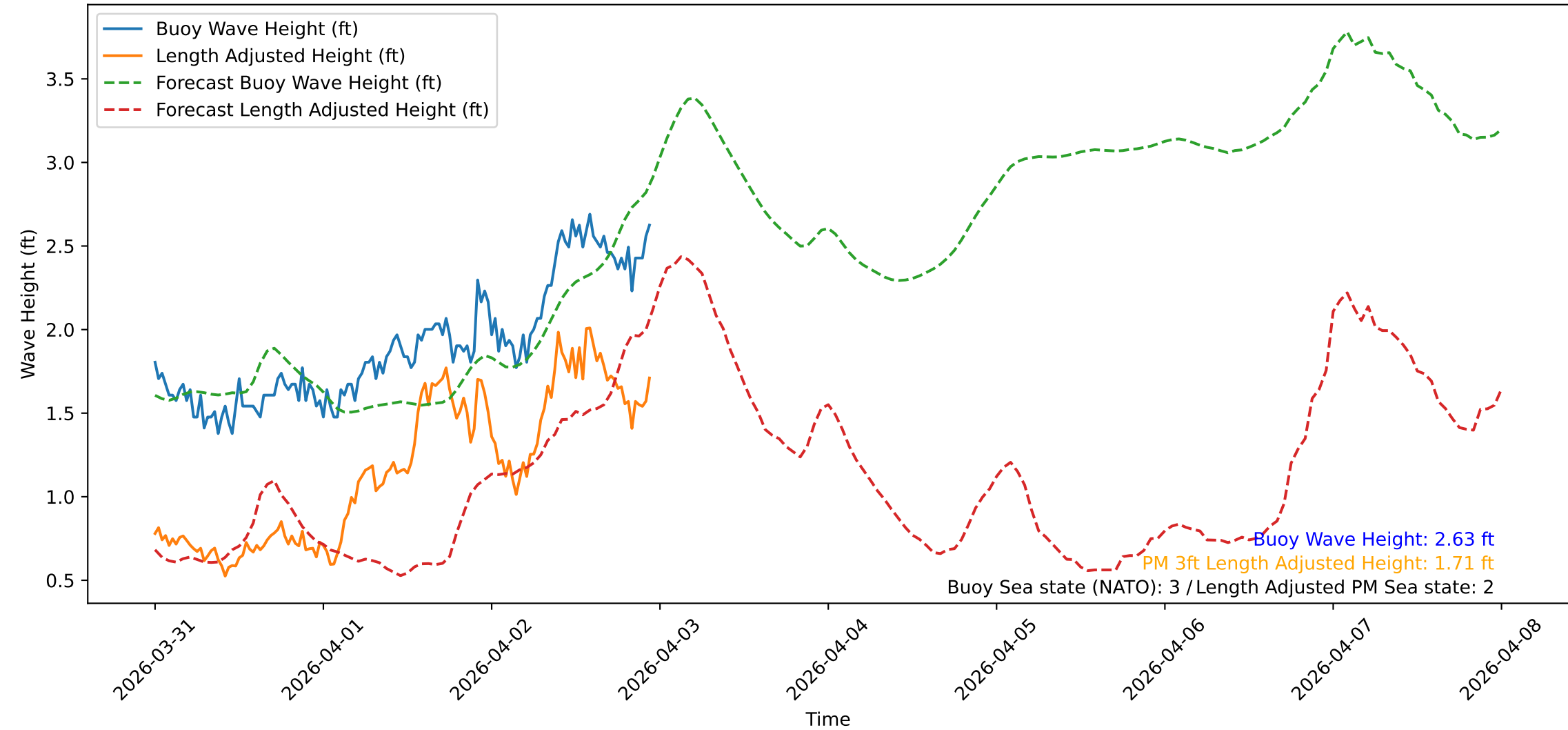
Wave Heights over Time for Red Beach at 2026-04-02 23:40:47
