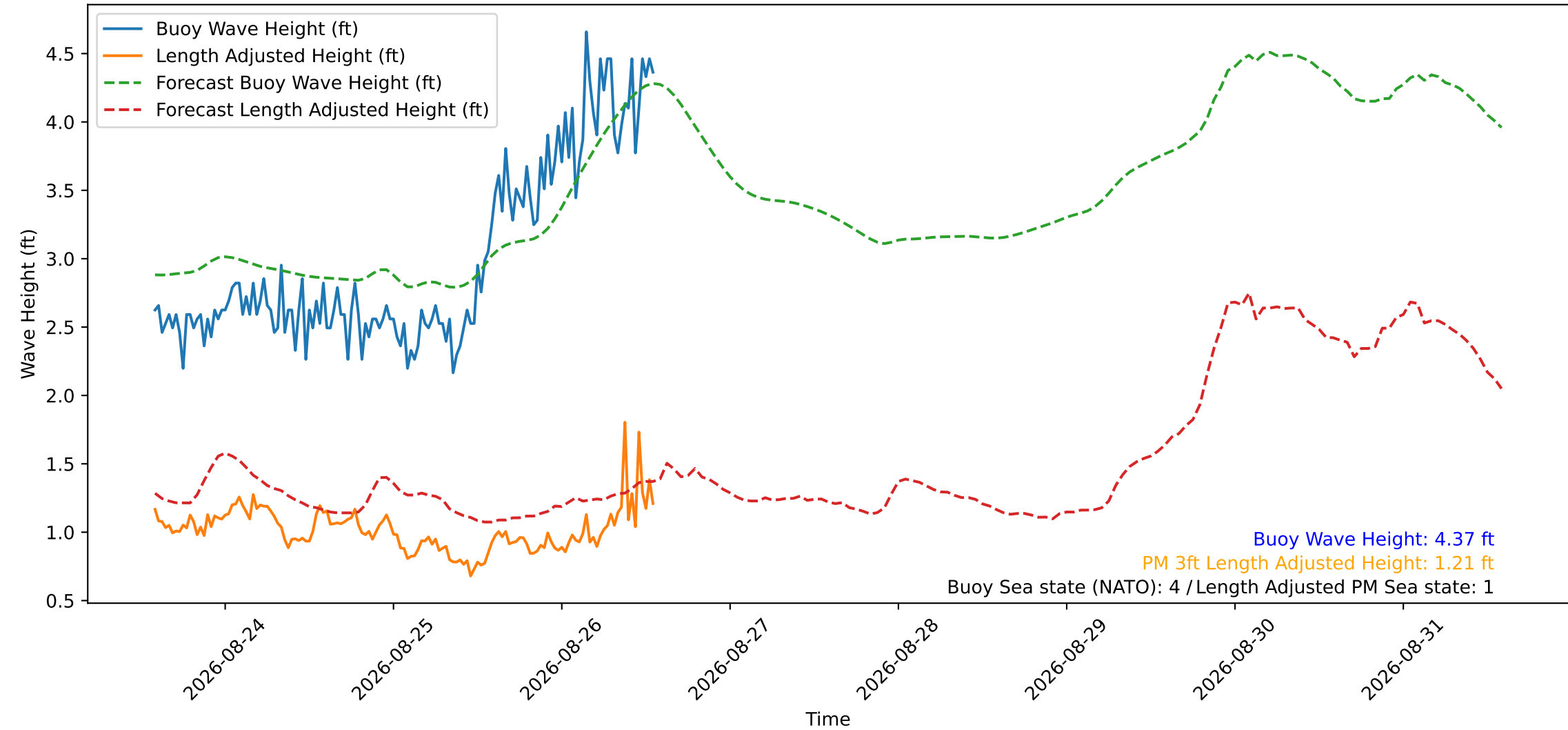
Wave Heights over Time for Red Beach at 2026-08-26 13:50:52
