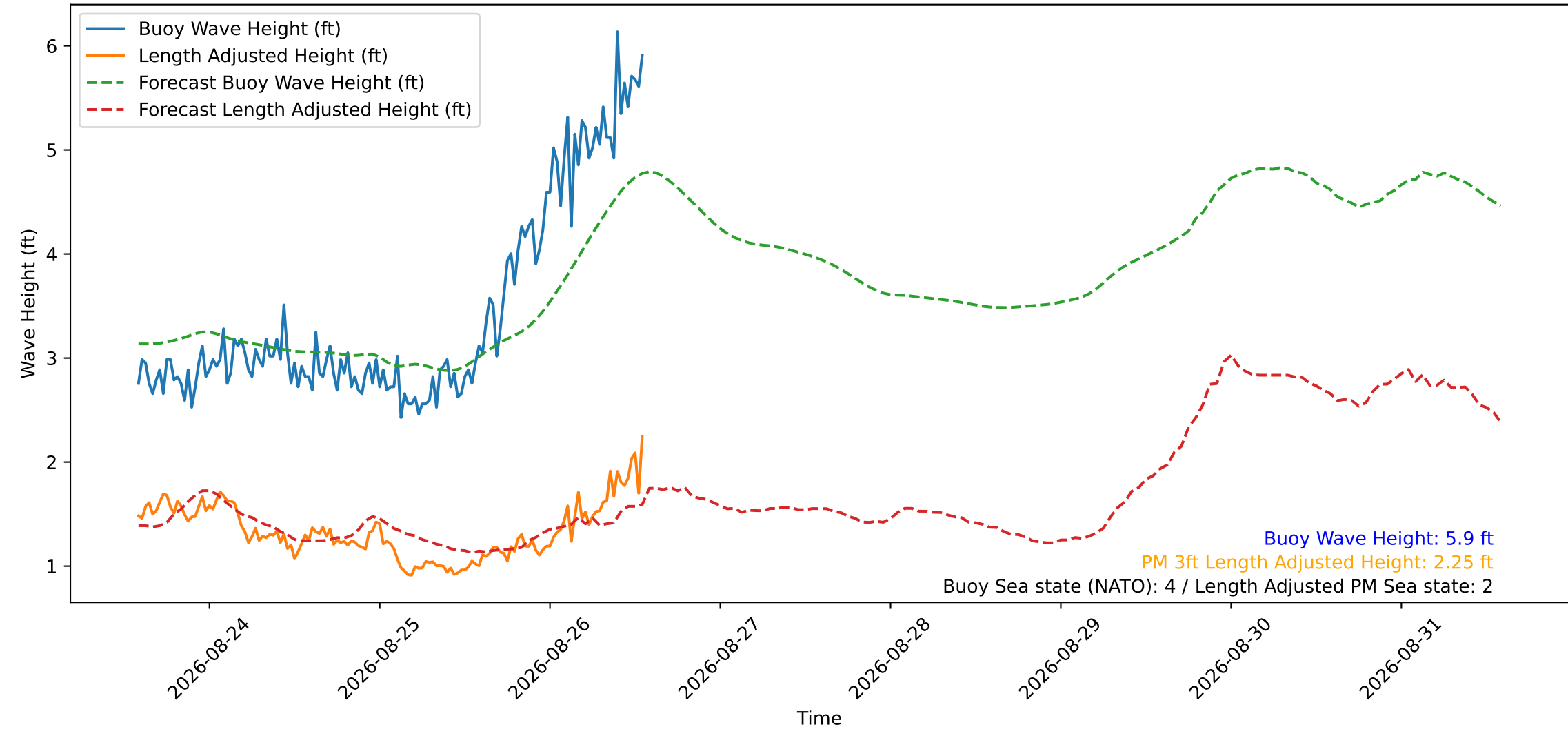
Wave Heights over Time for Oceanside Harbor at 2026-08-26 13:50:30
