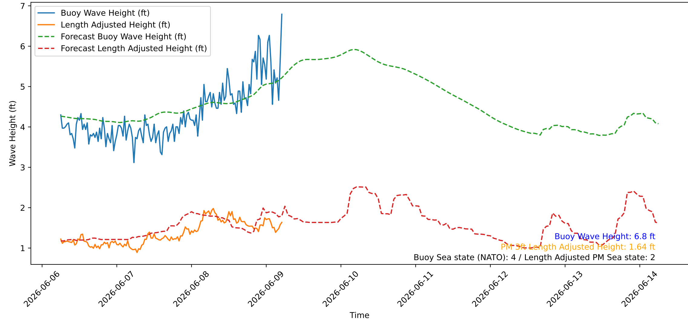
Wave Heights over Time for Green Beach at 2026-06-09 05:51:10
