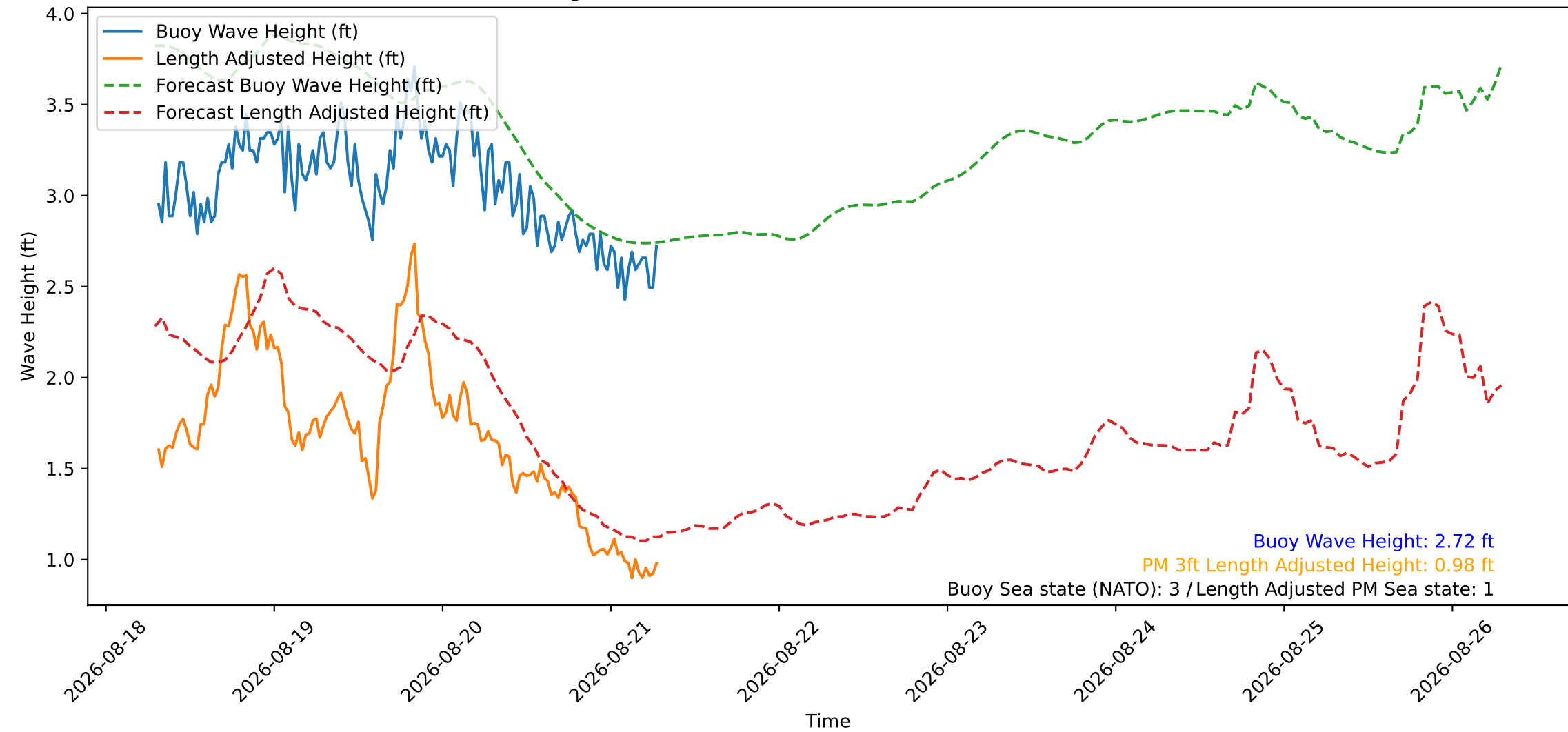
Wave Heights over Time for Green Beach at 2026-08-21 07:21:11
