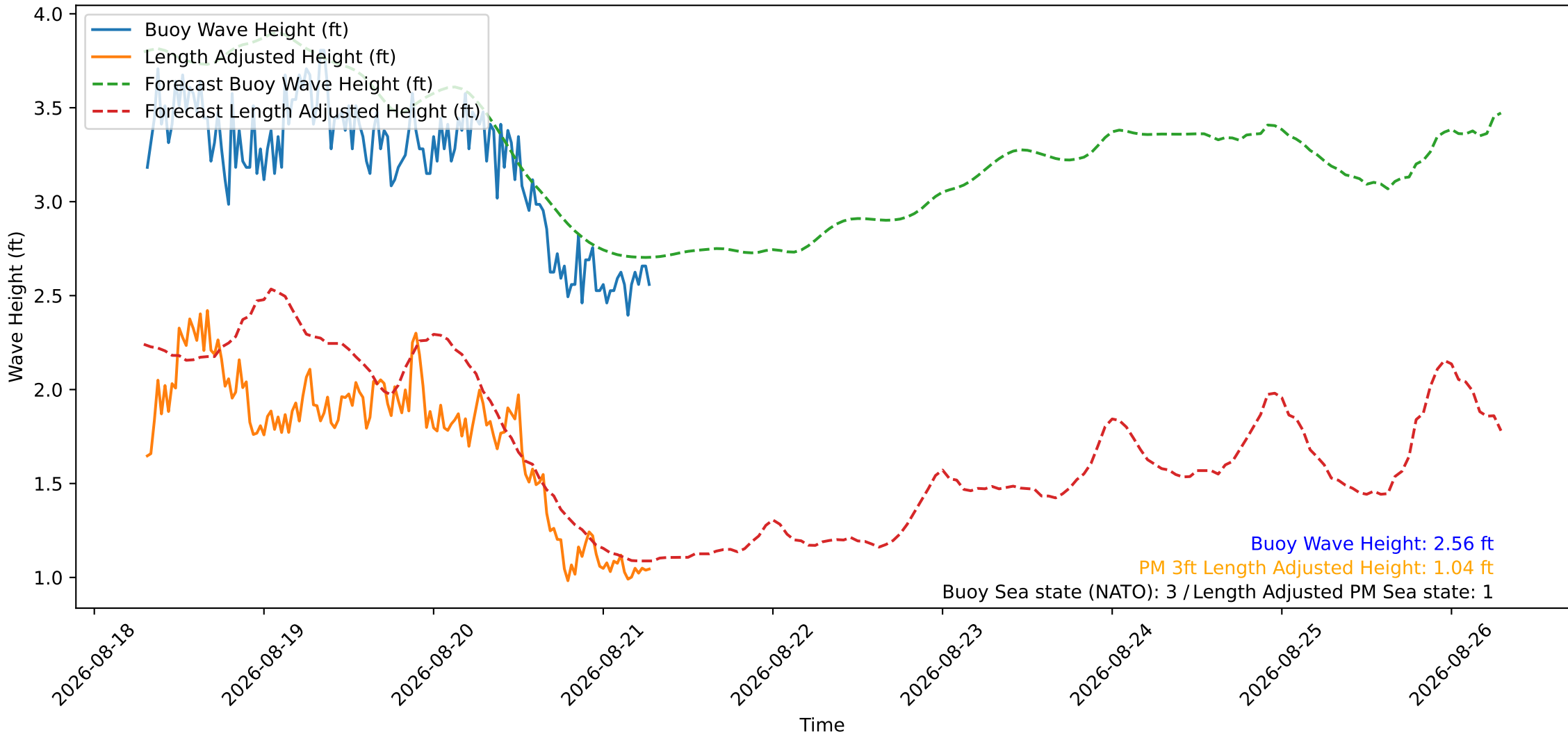
Wave Heights over Time for Oceanside Harbor at 2026-08-21 07:20:26
