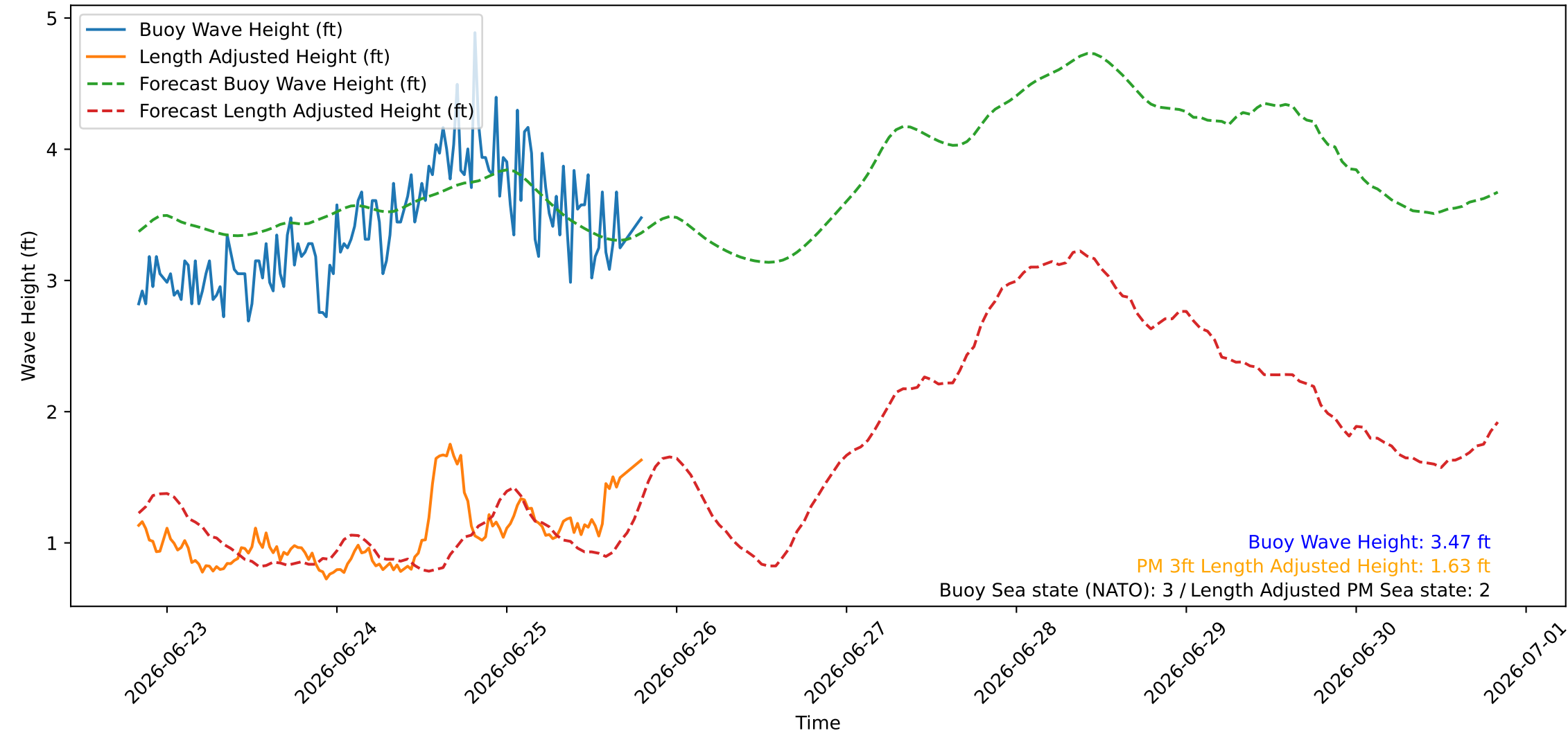
Wave Heights over Time for Oceanside Harbor at 2026-06-25 20:10:26
