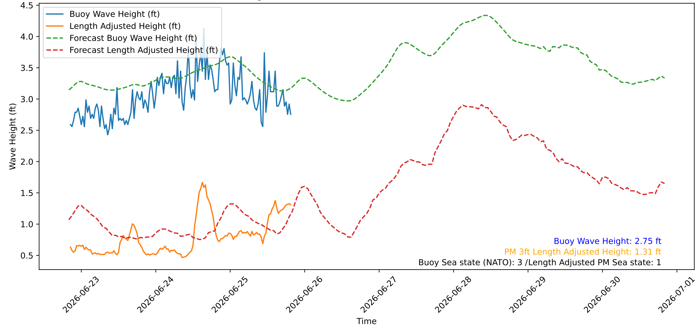
Wave Heights over Time for Red Beach at 2026-06-25 20:10:45
