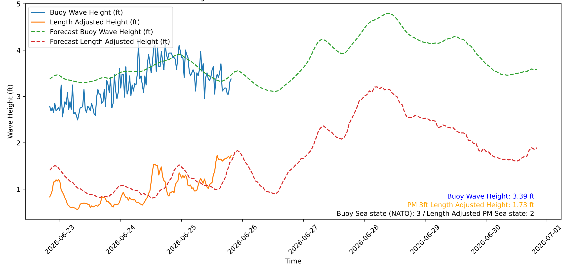
Wave Heights over Time for Green Beach at 2026-06-25 20:11:08
