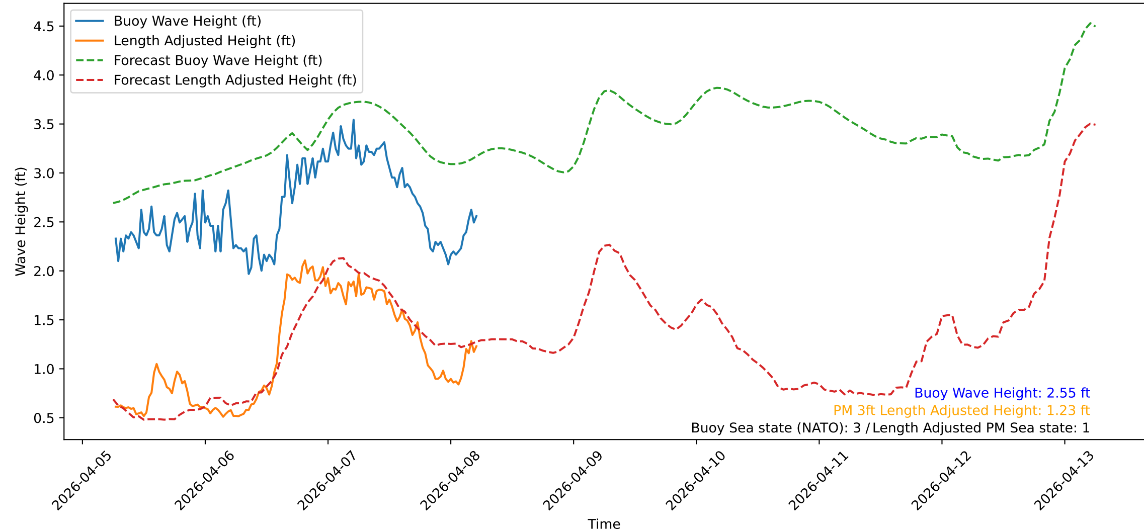
Wave Heights over Time for Red Beach at 2026-04-08 06:00:47
