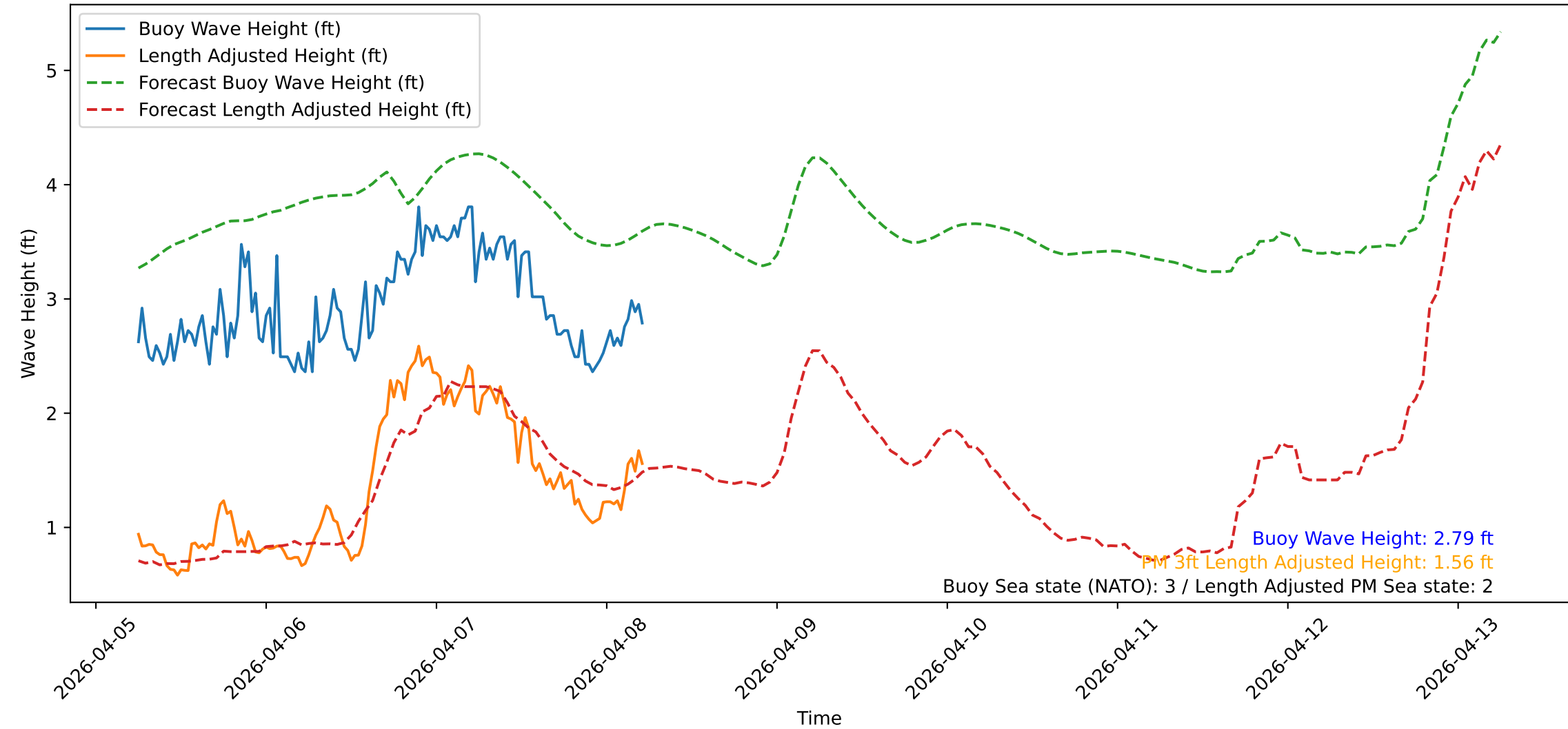
Wave Heights over Time for Green Beach at 2026-04-08 06:01:10
