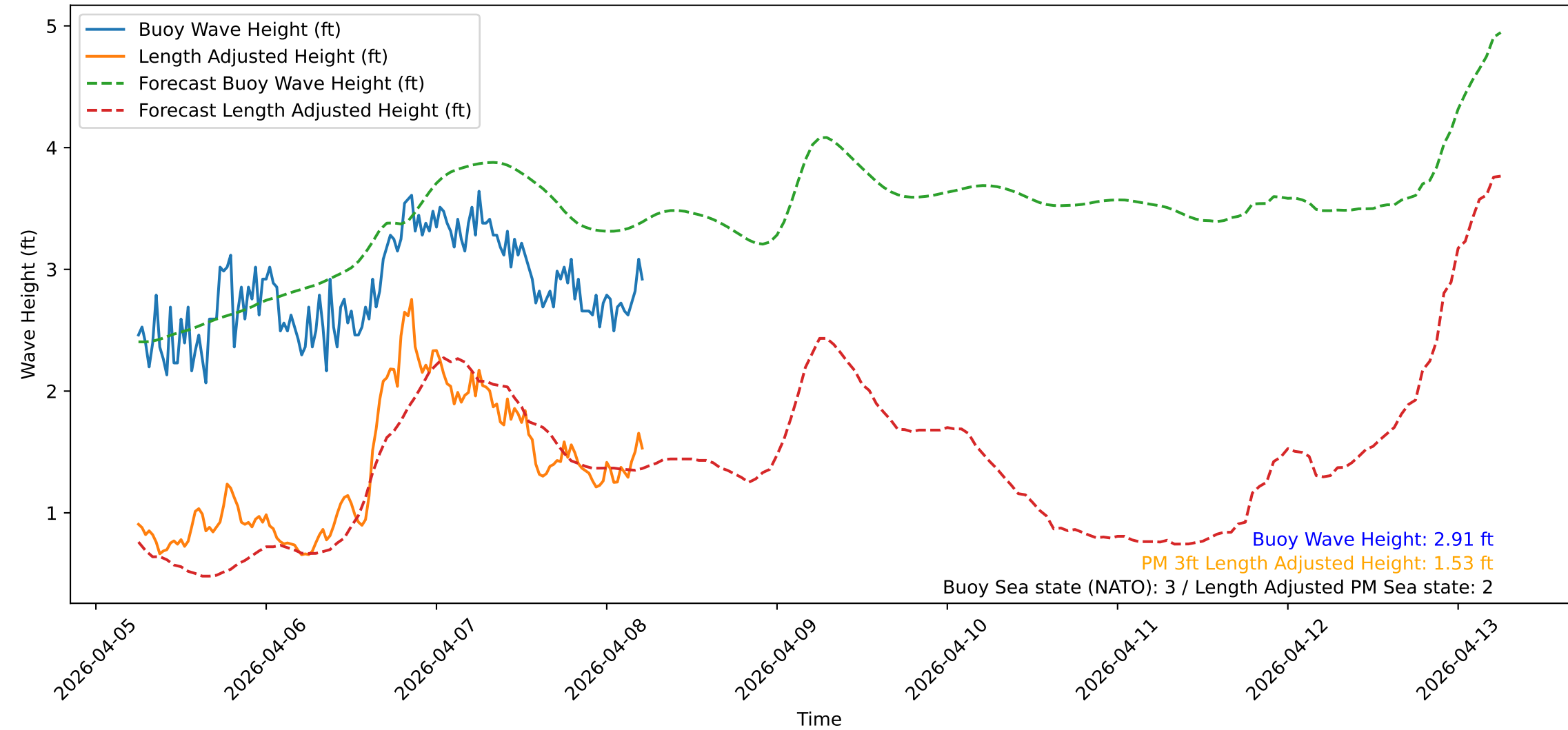
Wave Heights over Time for Oceanside Harbor at 2026-04-08 06:00:31
