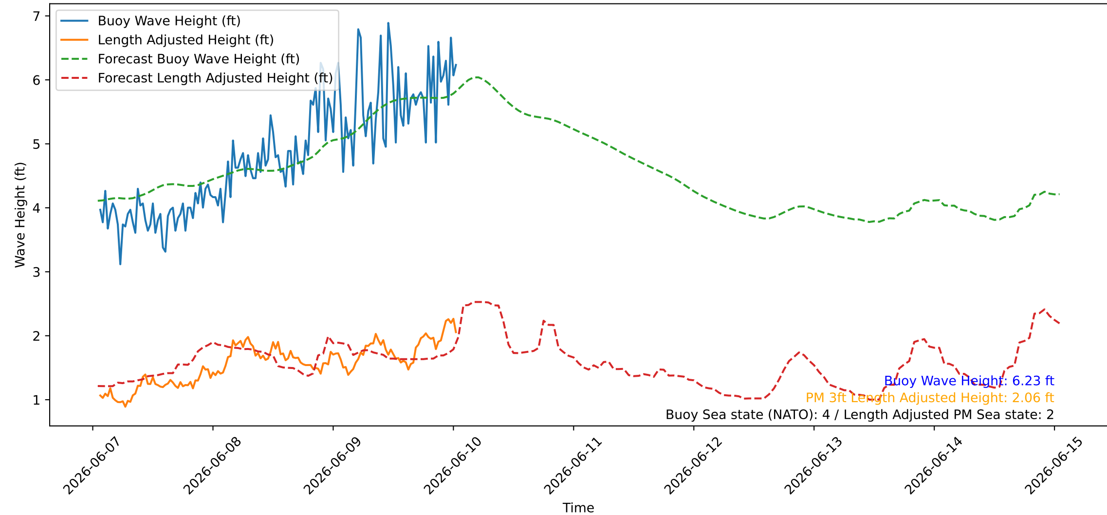
Wave Heights over Time for Green Beach at 2026-06-10 01:21:10
