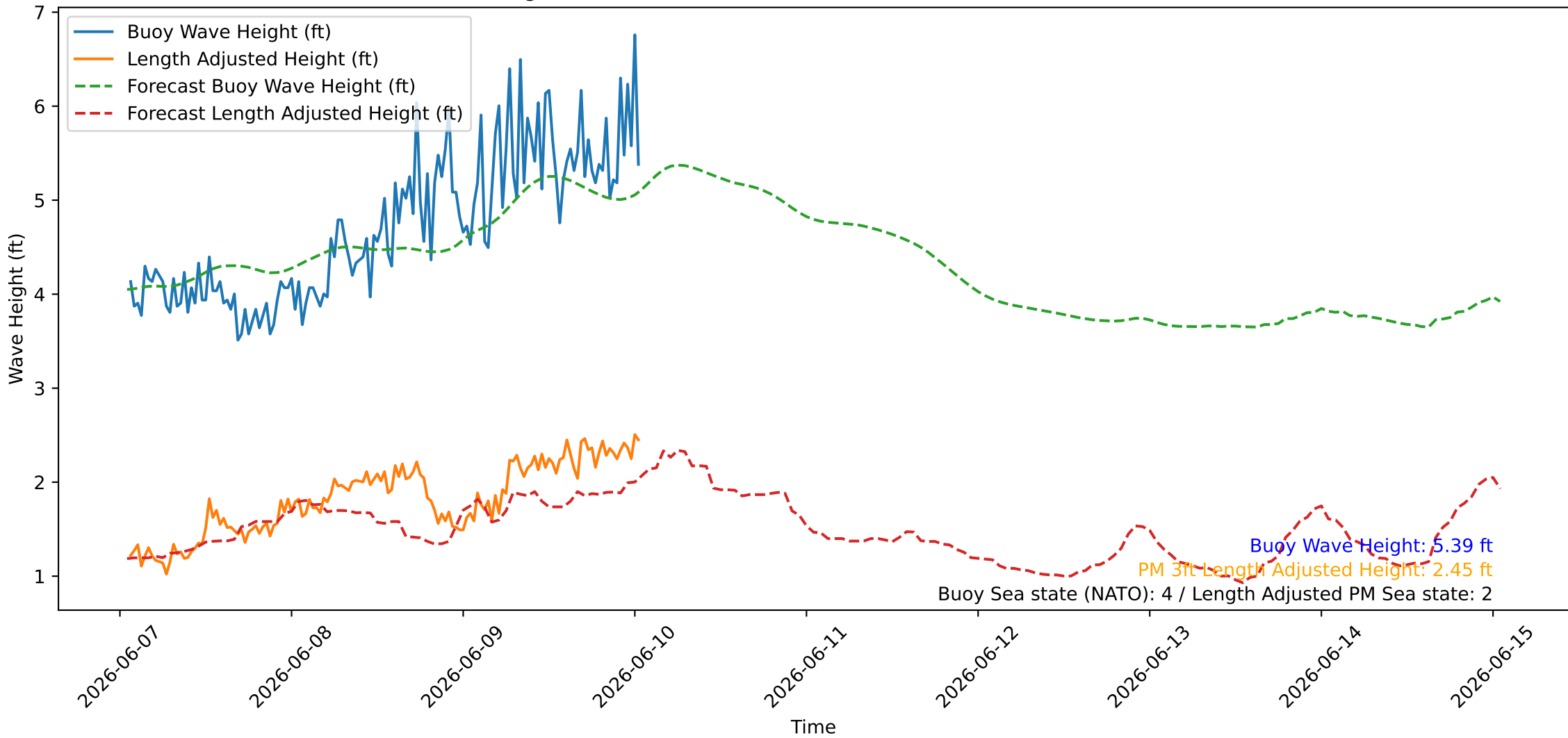
Wave Heights over Time for Oceanside Harbor at 2026-06-10 01:20:26
