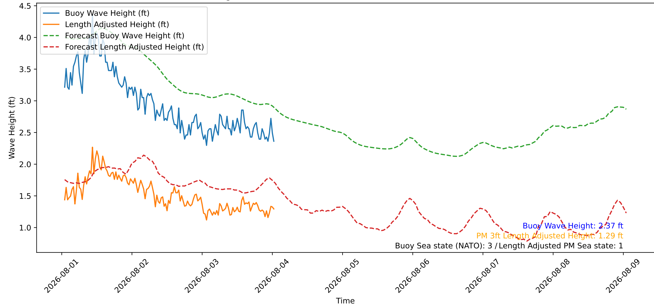
Wave Heights over Time for Oceanside Harbor at 2026-08-04 01:10:25
