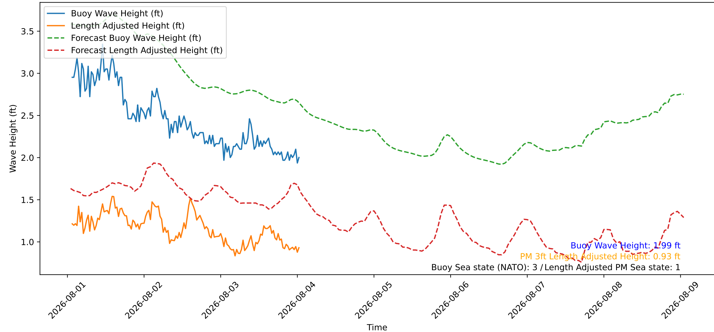
Wave Heights over Time for Red Beach at 2026-08-04 01:10:45
