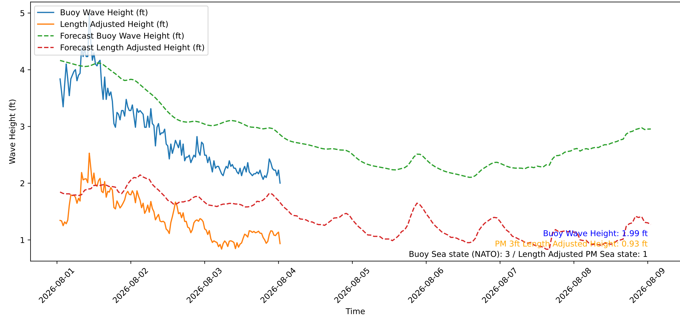
Wave Heights over Time for Green Beach at 2026-08-04 01:11:07
