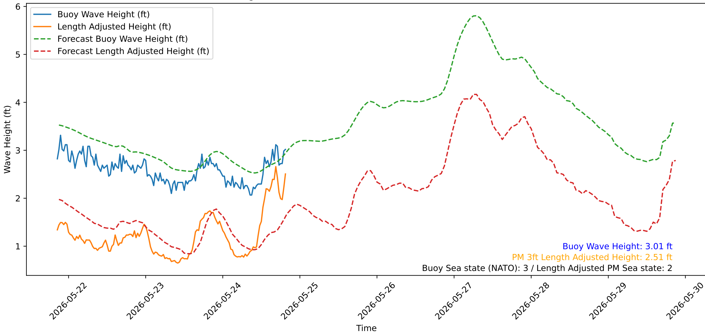
Wave Heights over Time for Green Beach at 2026-05-24 20:31:14
