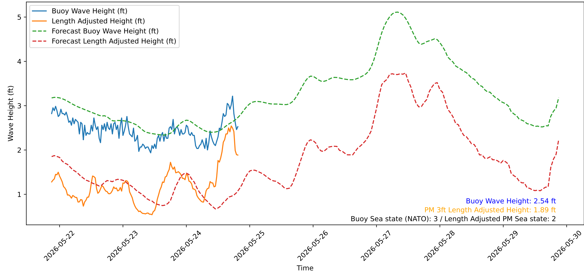
Wave Heights over Time for Red Beach at 2026-05-24 20:30:51
