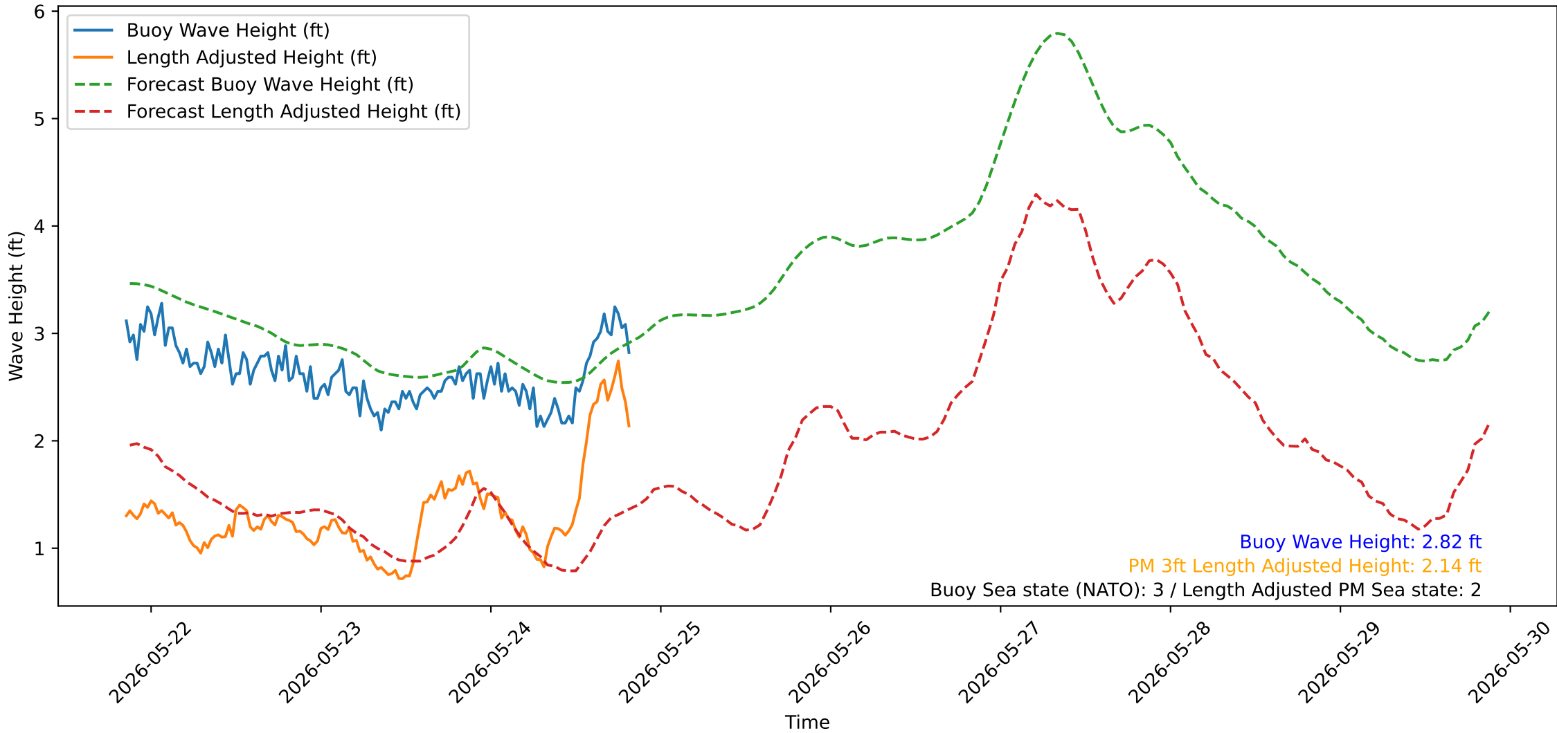
Wave Heights over Time for Oceanside Harbor at 2026-05-24 20:30:32
