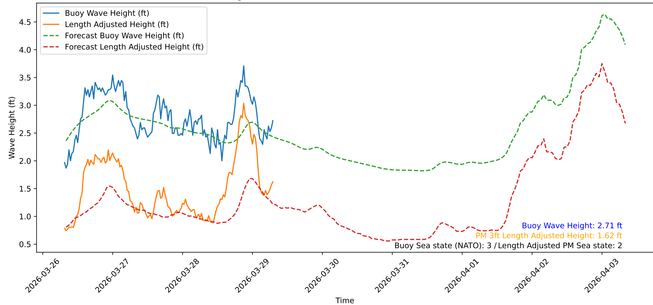
Wave Heights over Time for Green Beach at 2026-03-29 07:41:10
