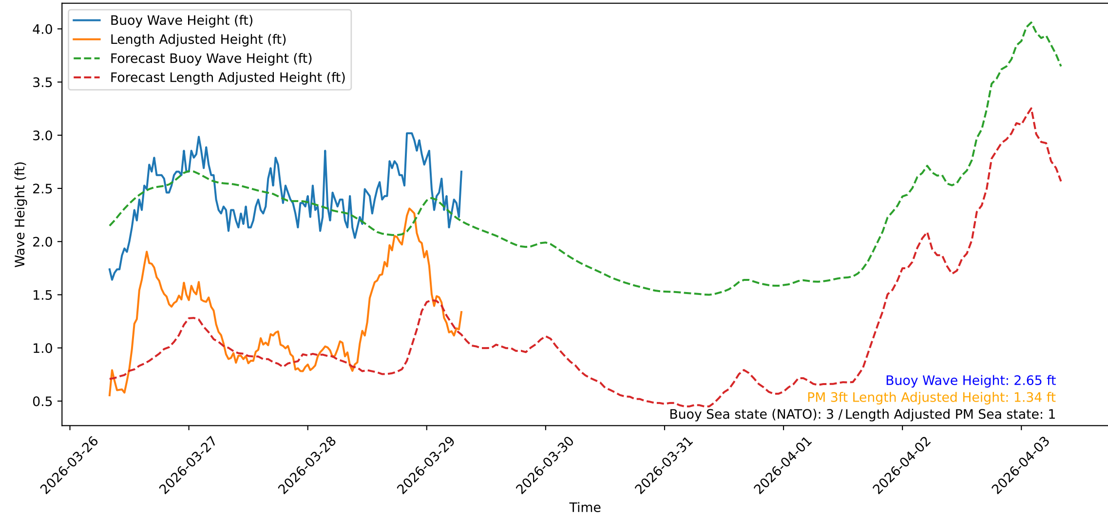
Wave Heights over Time for Red Beach at 2026-03-29 07:40:47
