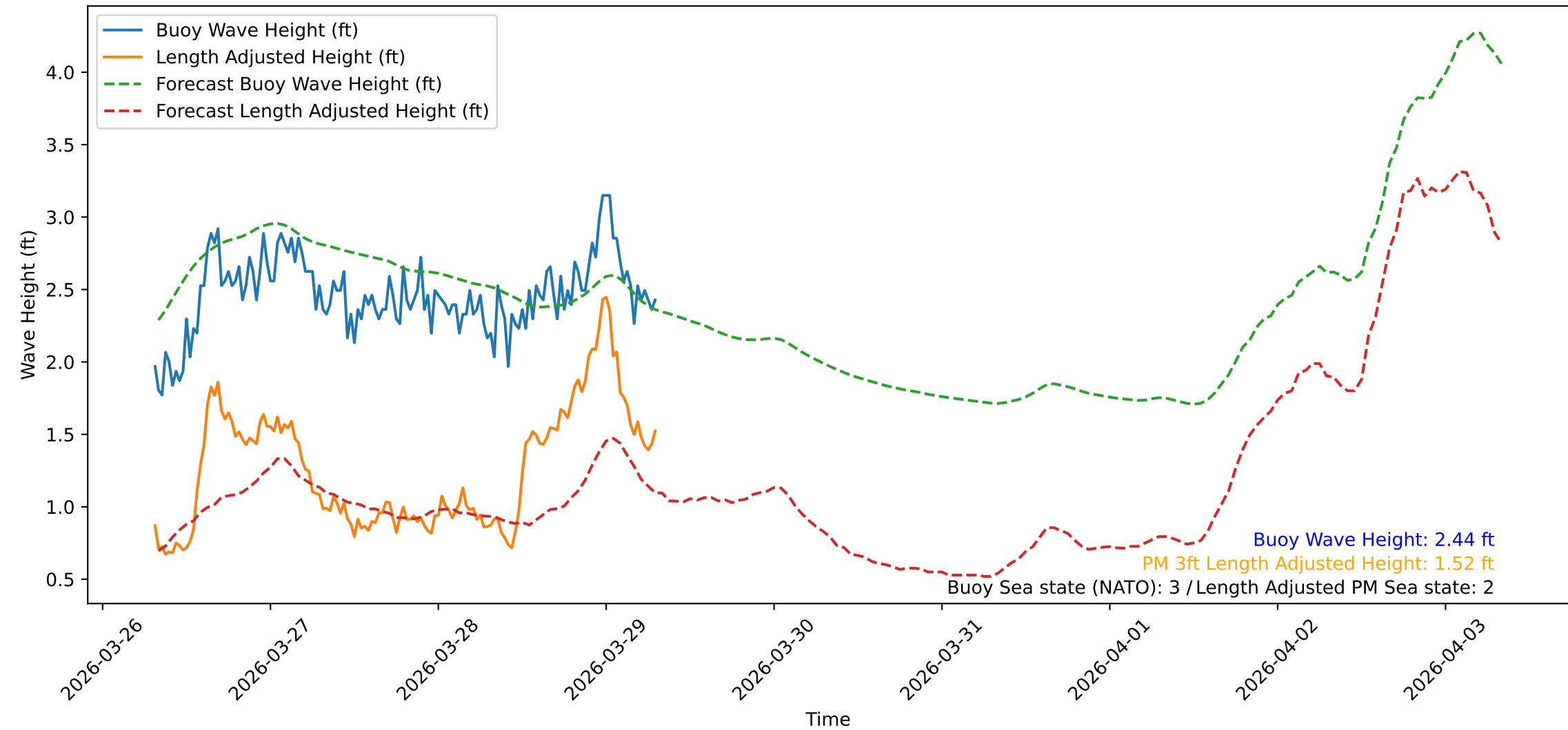
Wave Heights over Time for Oceanside Harbor at 2026-03-29 07:40:31
