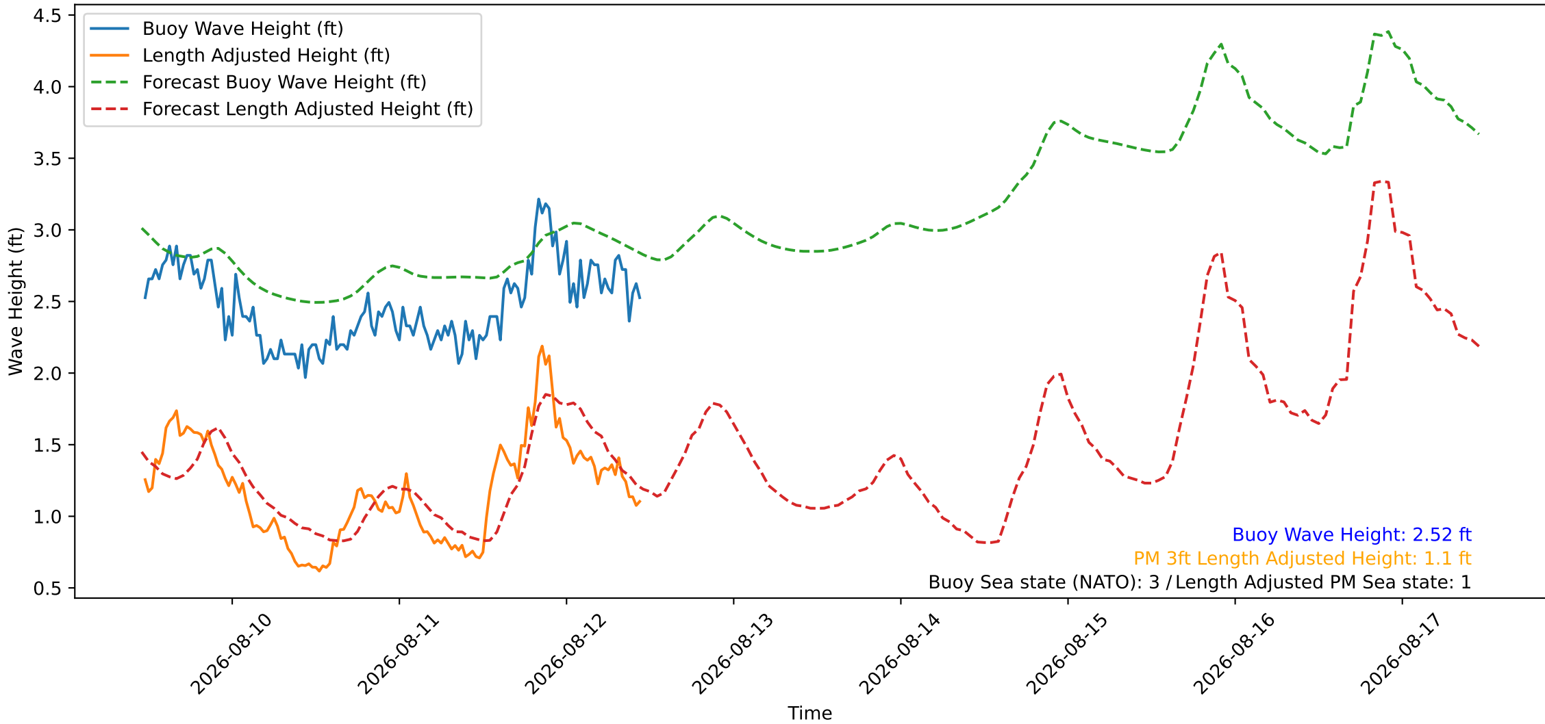
Wave Heights over Time for Green Beach at 2026-08-12 11:21:11
