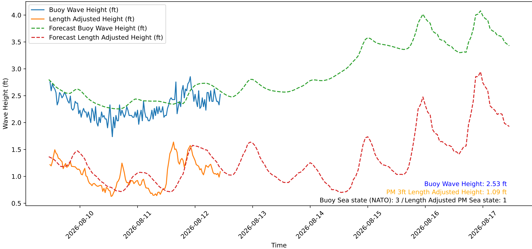
Wave Heights over Time for Red Beach at 2026-08-12 11:20:48
