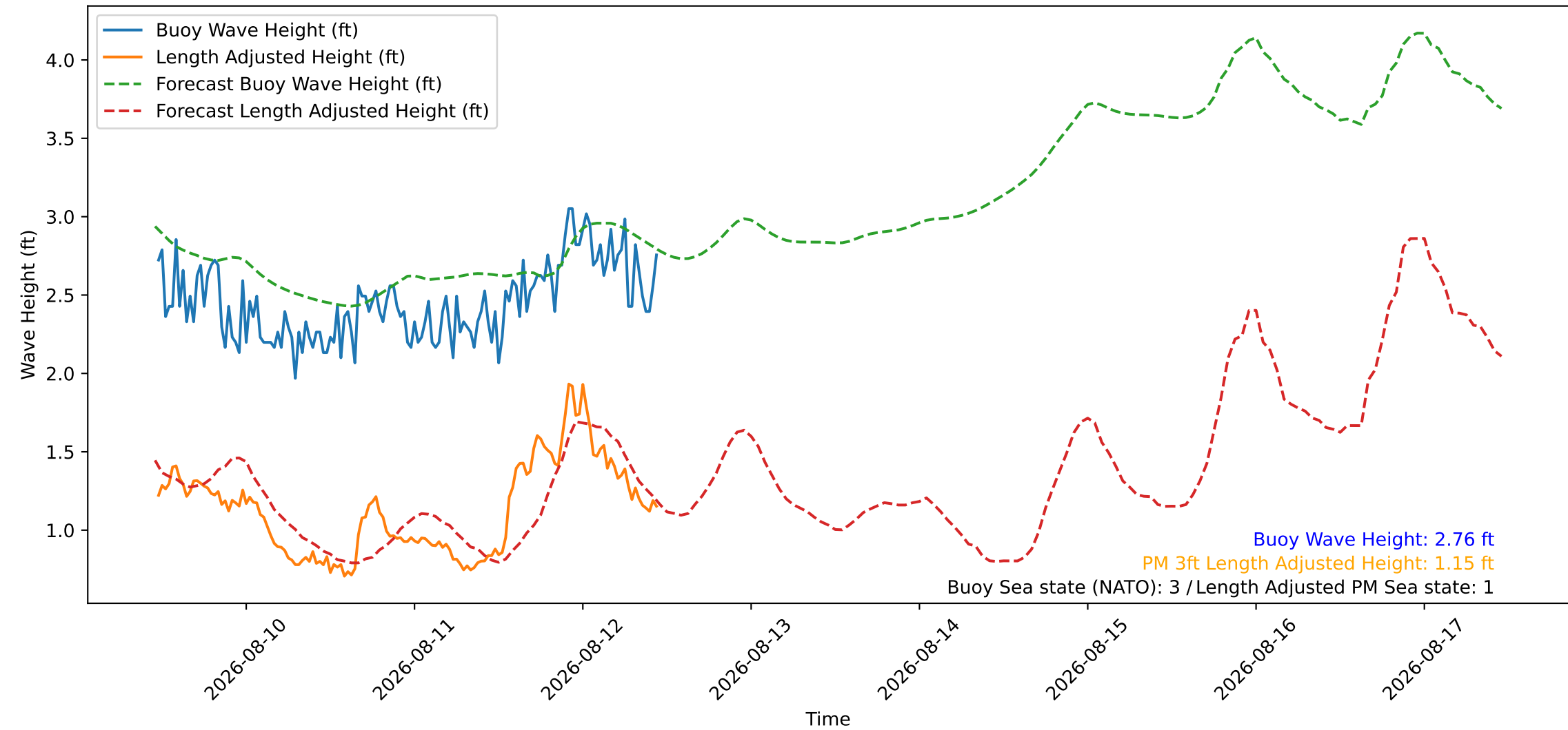
Wave Heights over Time for Oceanside Harbor at 2026-08-12 11:20:26
