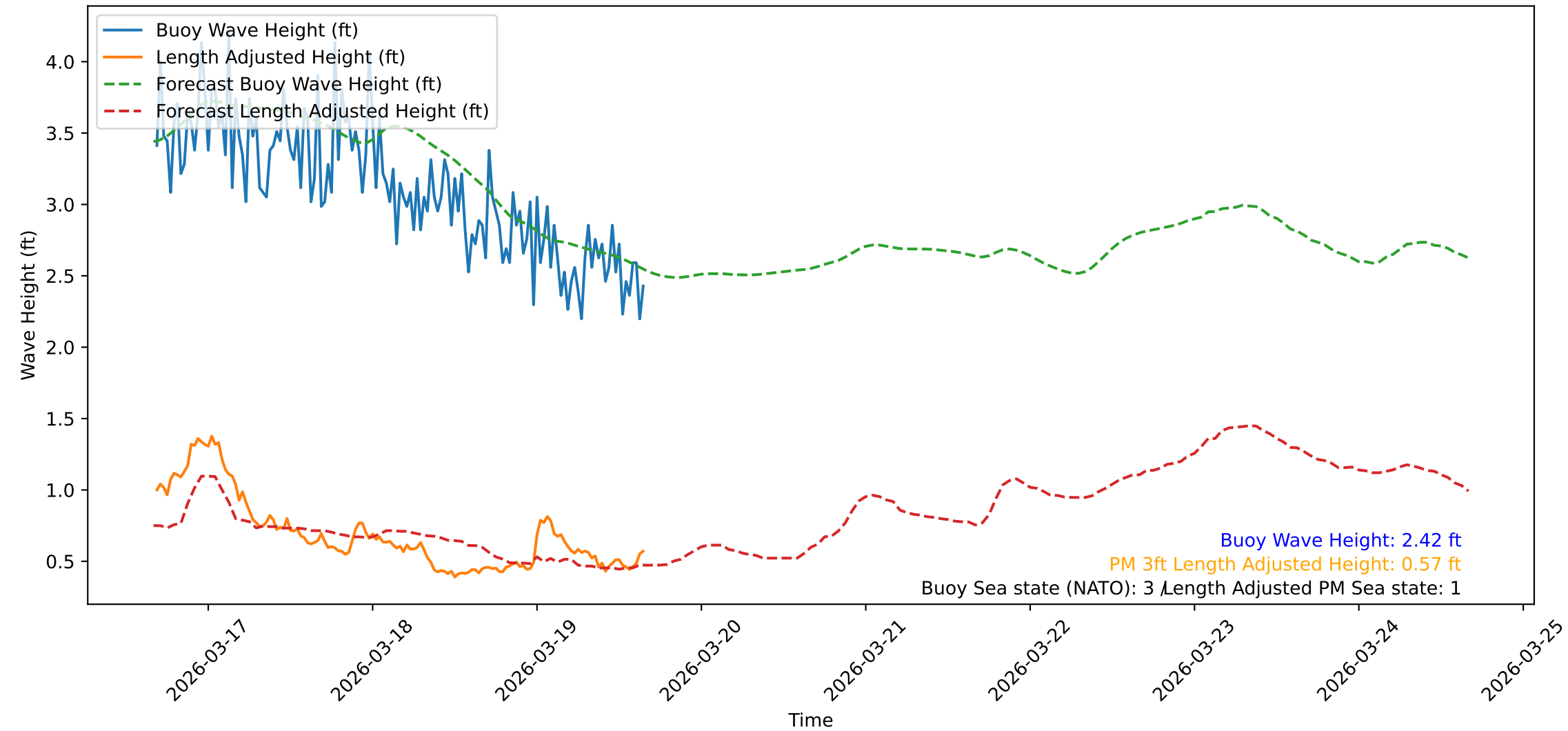
Wave Heights over Time for Green Beach at 2026-03-19 16:21:10
