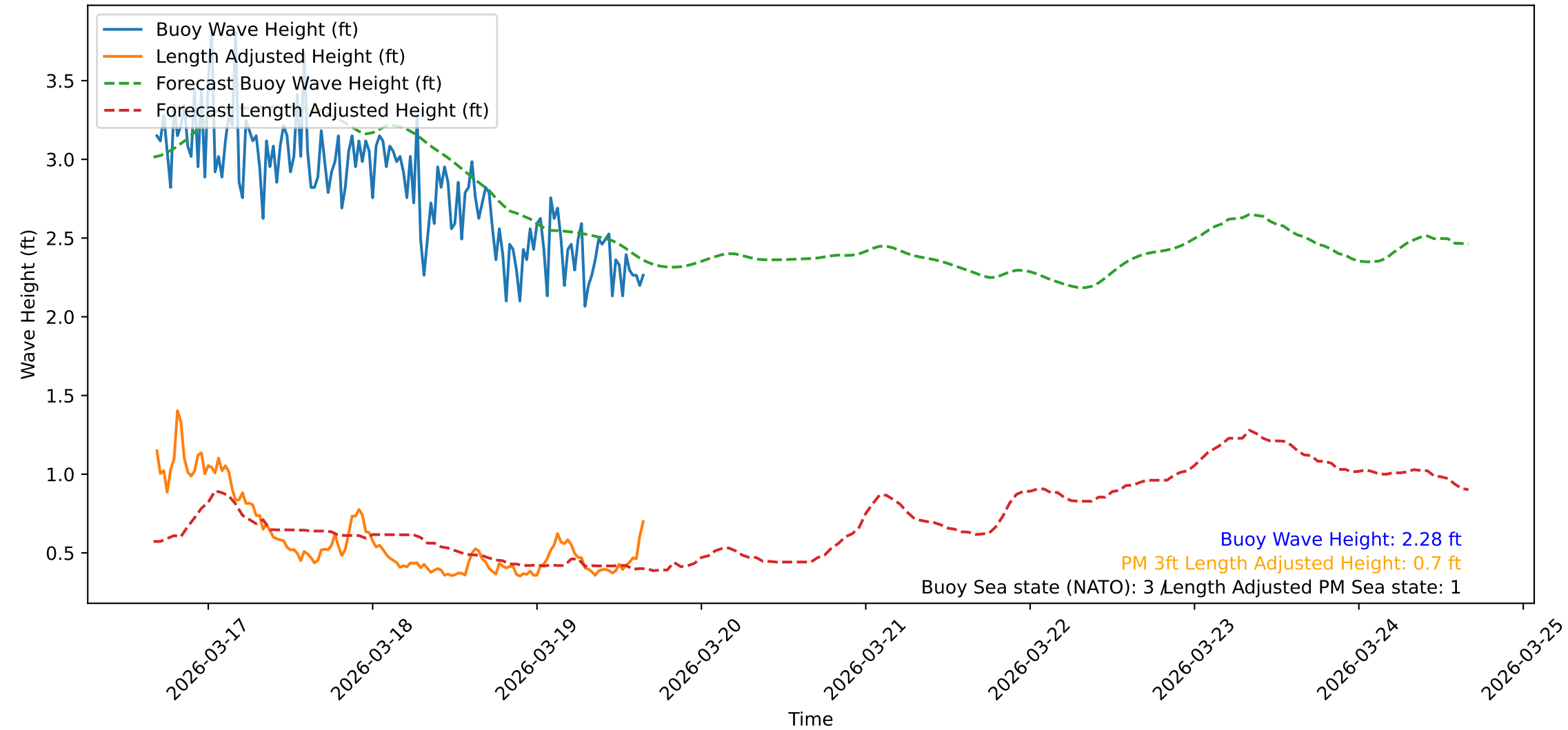
Wave Heights over Time for Red Beach at 2026-03-19 16:20:47
