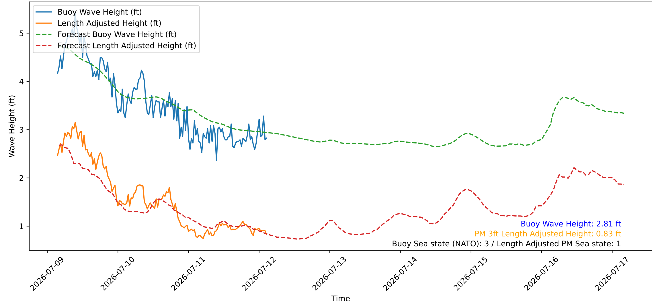
Wave Heights over Time for Oceanside Harbor at 2026-07-12 03:30:26
