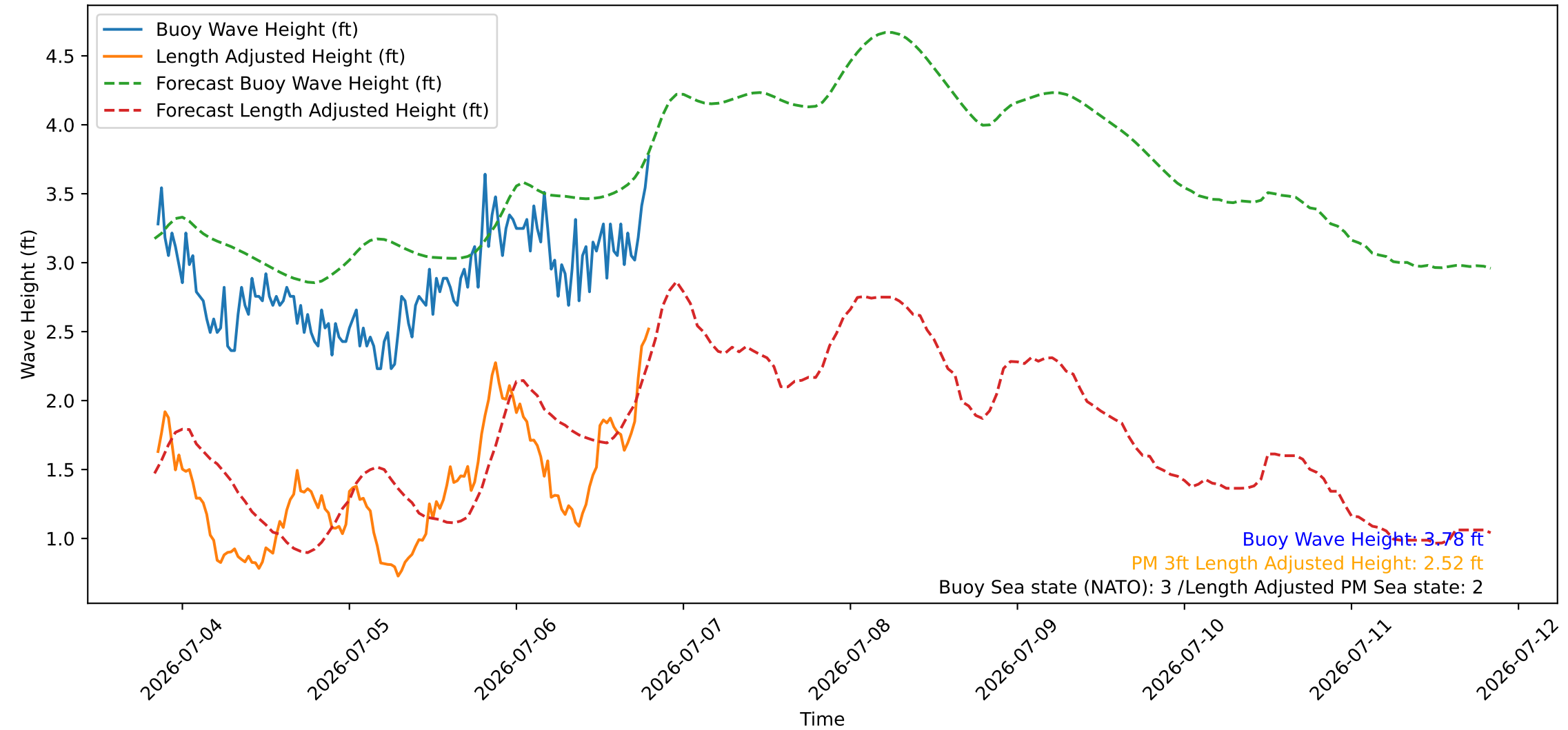
Wave Heights over Time for Red Beach at 2026-07-06 20:20:47
