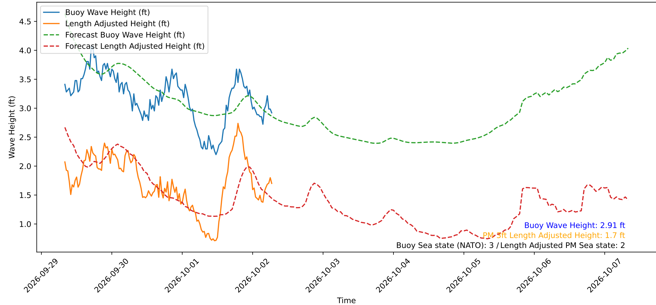
Wave Heights over Time for Green Beach at 2026-10-02 07:31:11
