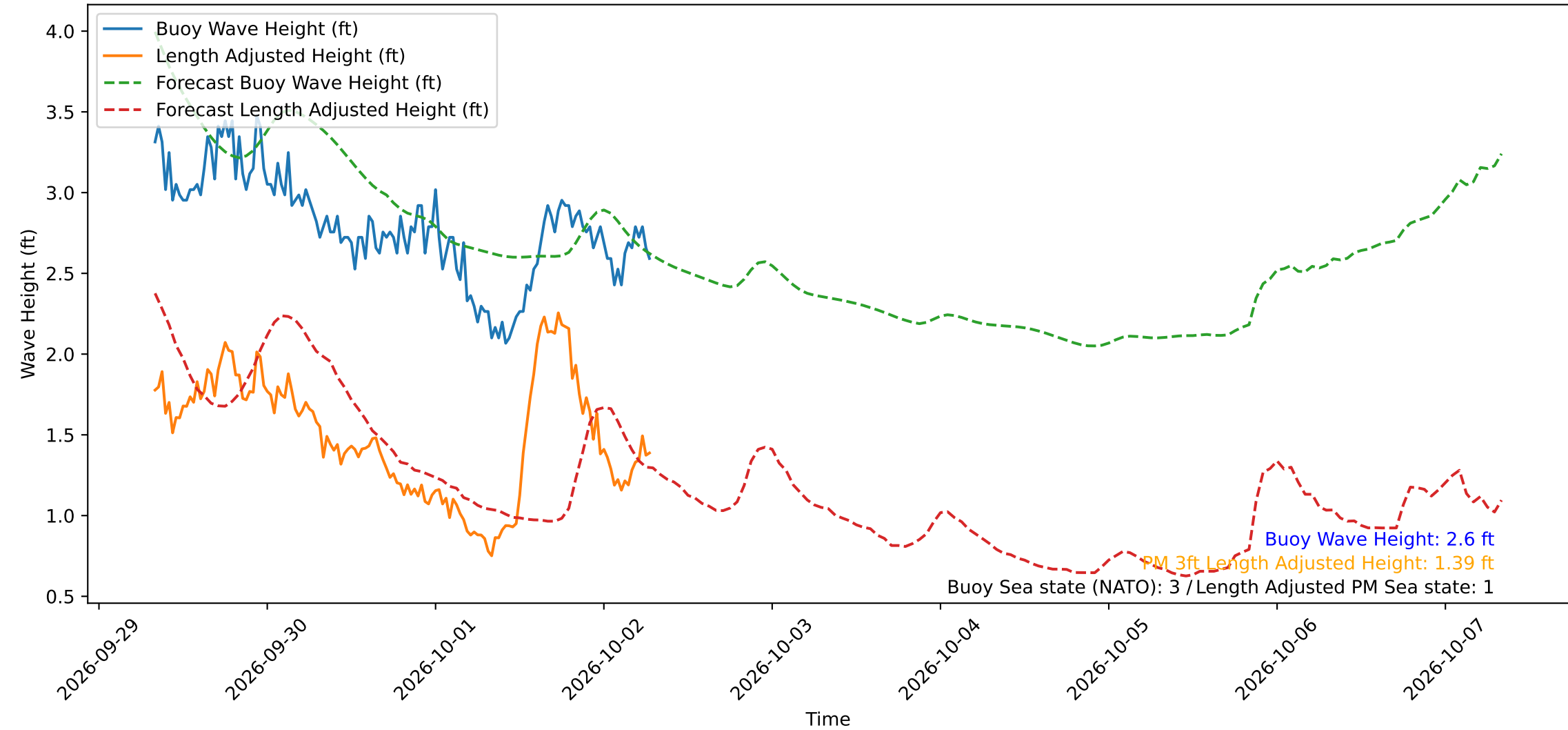
Wave Heights over Time for Red Beach at 2026-10-02 07:30:49
