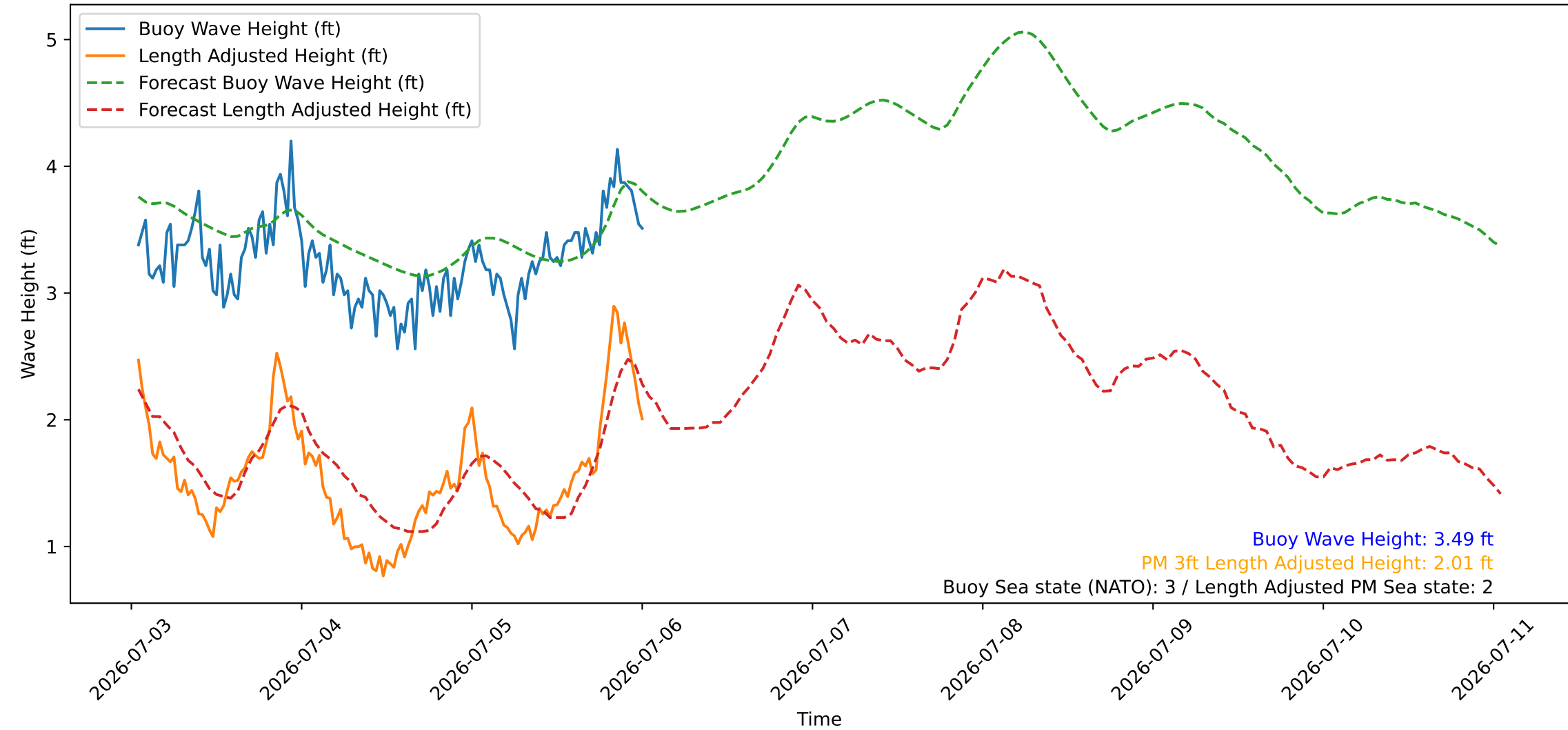
Wave Heights over Time for Green Beach at 2026-07-06 01:01:08
