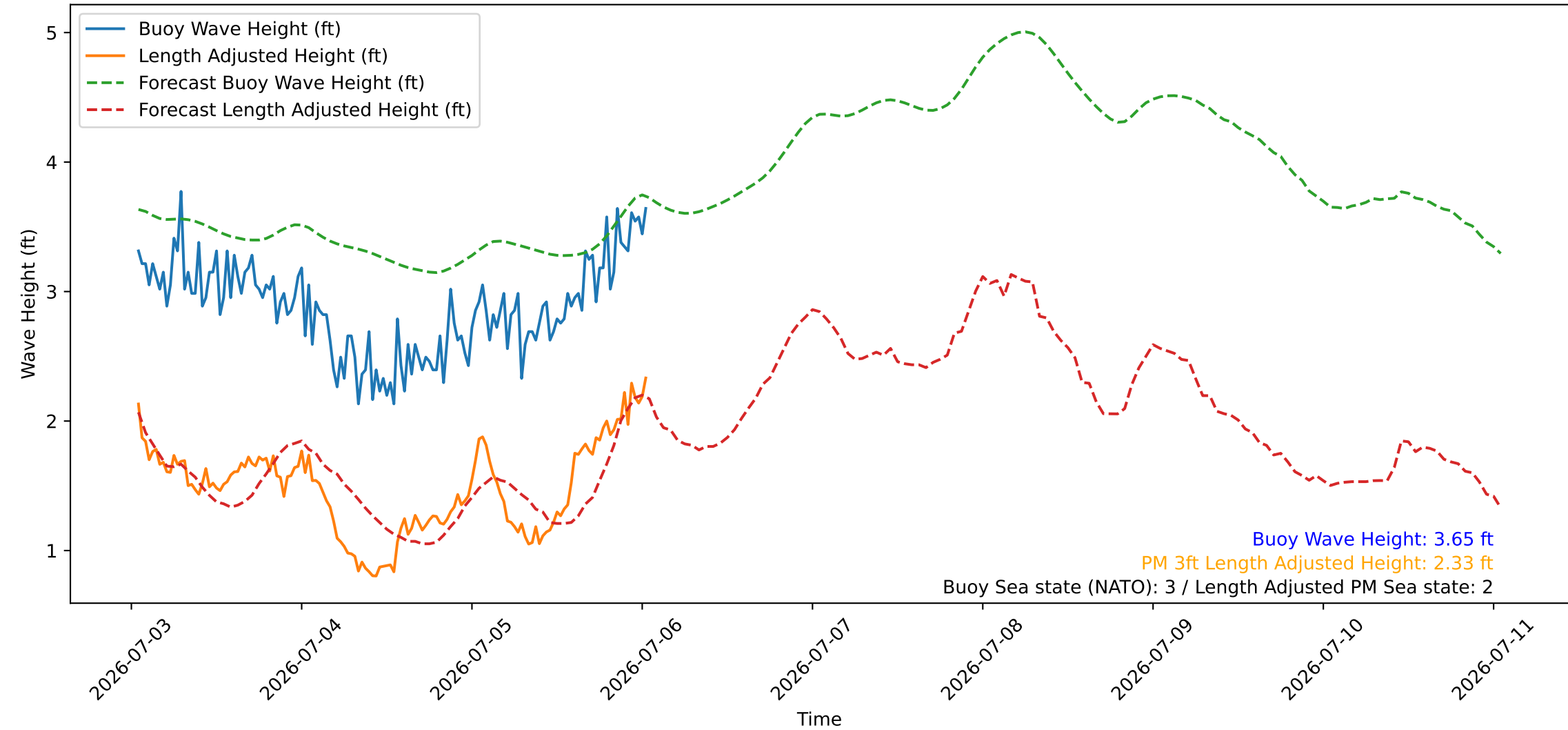
Wave Heights over Time for Oceanside Harbor at 2026-07-06 01:00:26
