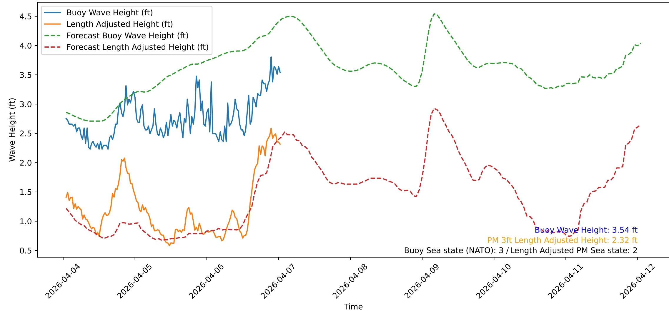
Wave Heights over Time for Green Beach at 2026-04-07 01:11:10
