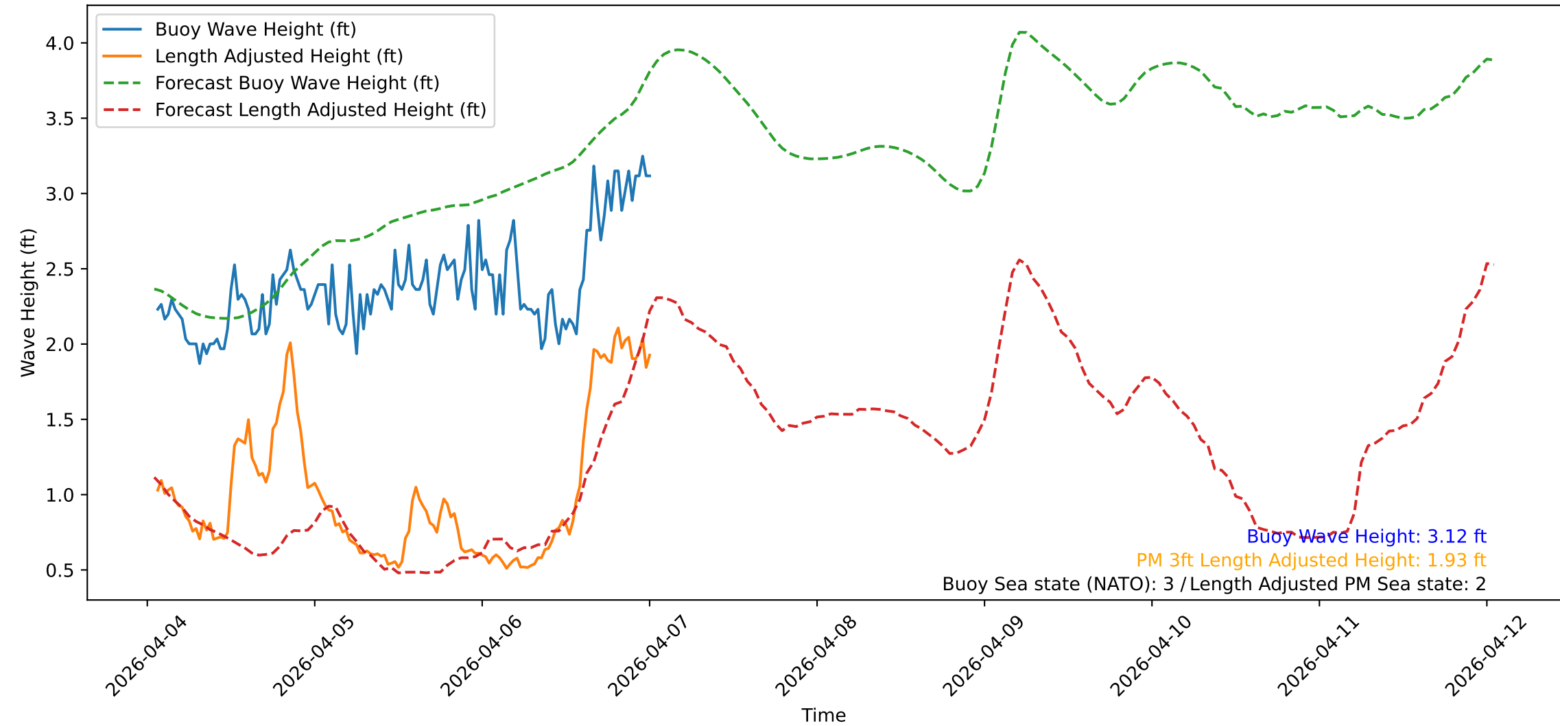
Wave Heights over Time for Red Beach at 2026-04-07 01:10:48
