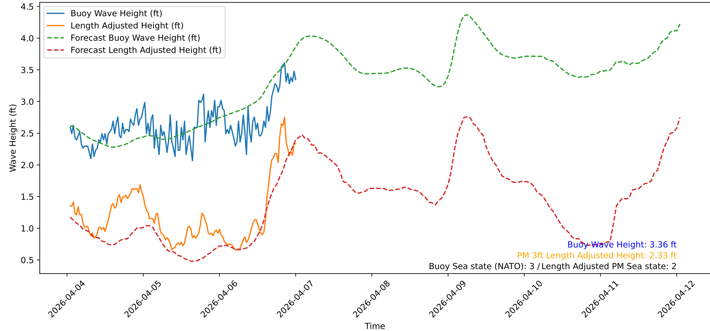
Wave Heights over Time for Oceanside Harbor at 2026-04-07 01:10:31
