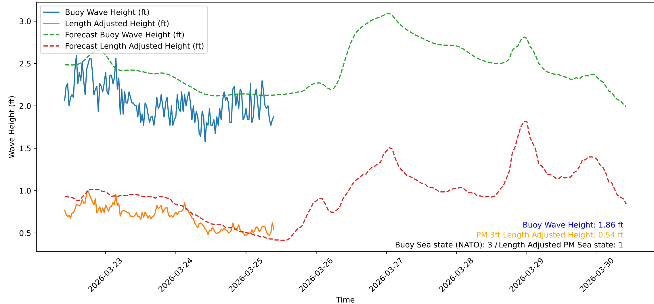
Wave Heights over Time for Oceanside Harbor at 2026-03-25 10:10:31
