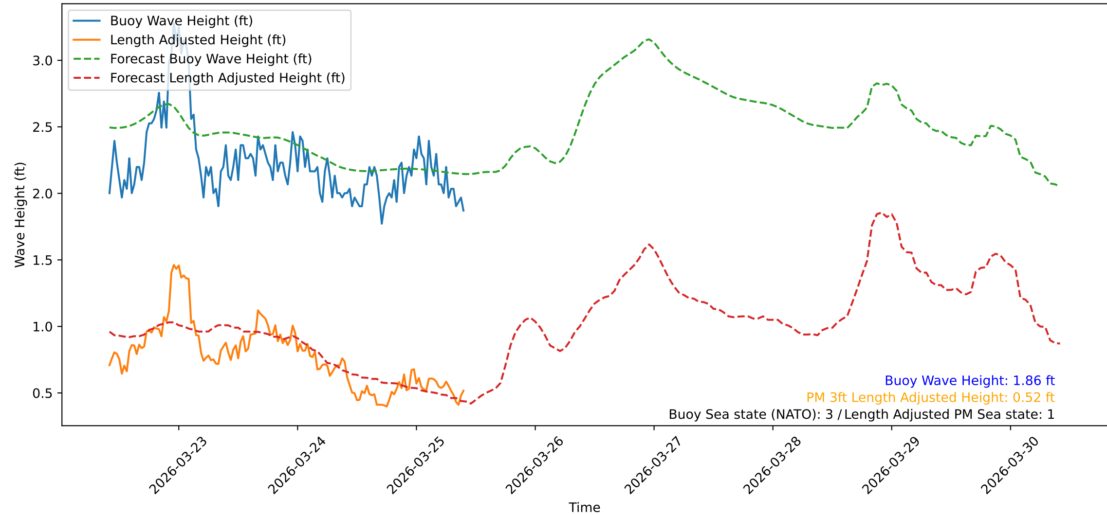
Wave Heights over Time for Green Beach at 2026-03-25 10:11:09
