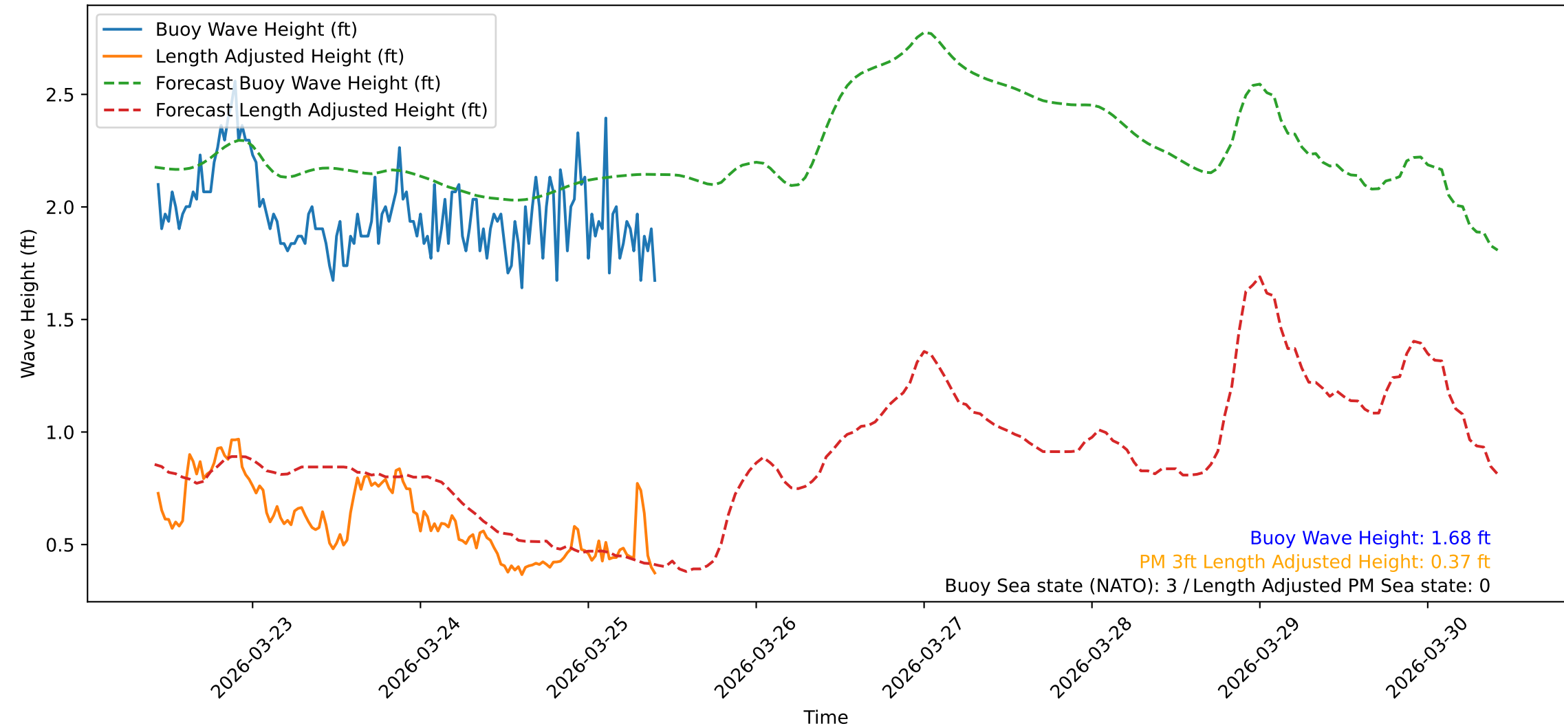
Wave Heights over Time for Red Beach at 2026-03-25 10:10:47
