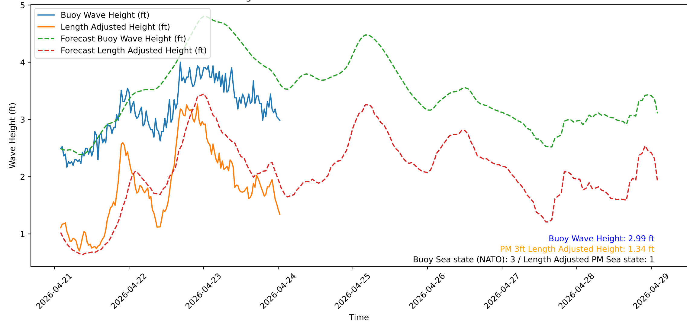
Wave Heights over Time for Green Beach at 2026-04-24 02:01:12
