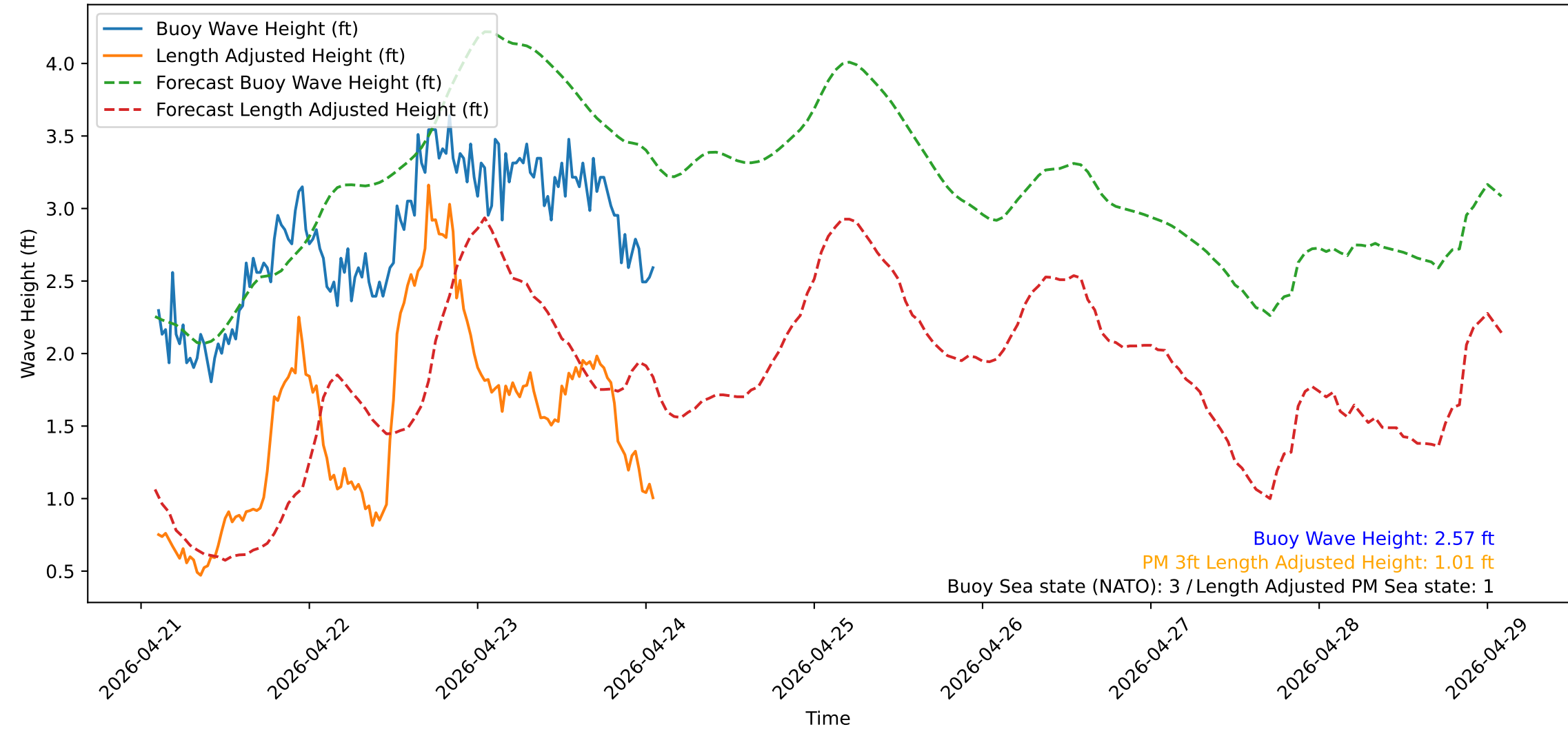
Wave Heights over Time for Red Beach at 2026-04-24 02:00:50
