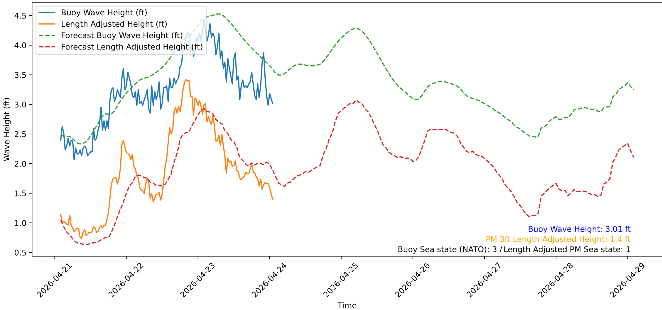
Wave Heights over Time for Oceanside Harbor at 2026-04-24 02:00:31
