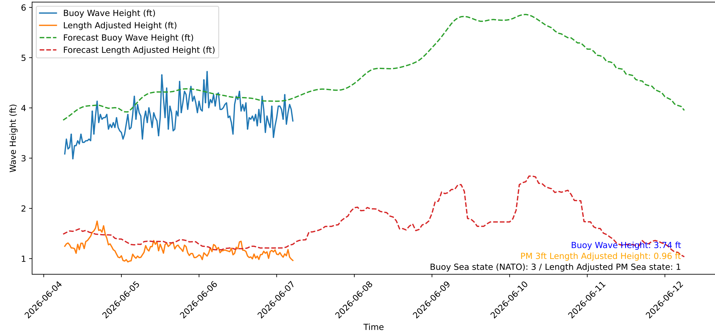
Wave Heights over Time for Green Beach at 2026-06-07 06:21:09
