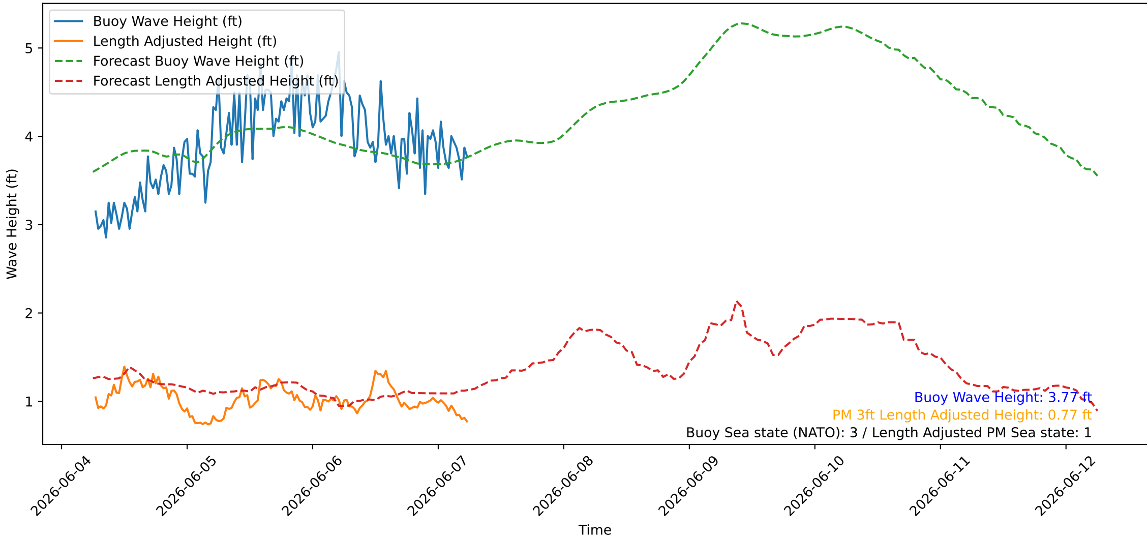
Wave Heights over Time for Red Beach at 2026-06-07 06:20:47
