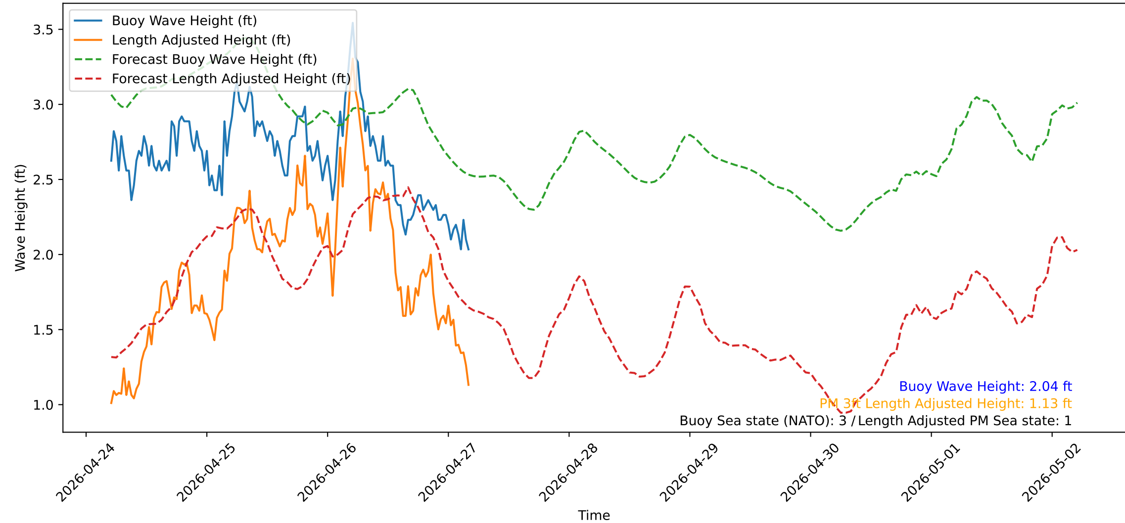
Wave Heights over Time for Red Beach at 2026-04-27 04:50:51
