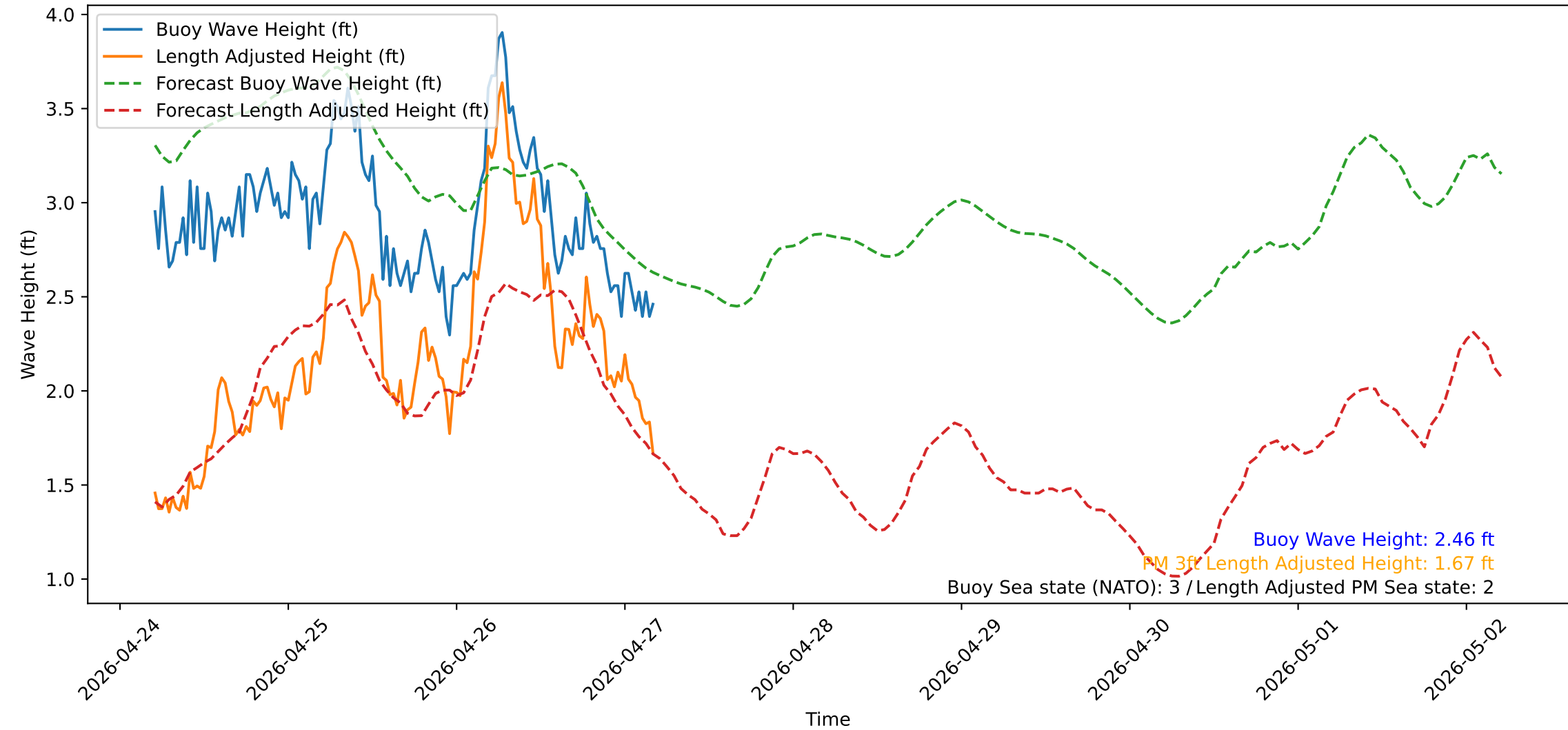
Wave Heights over Time for Oceanside Harbor at 2026-04-27 04:50:31
