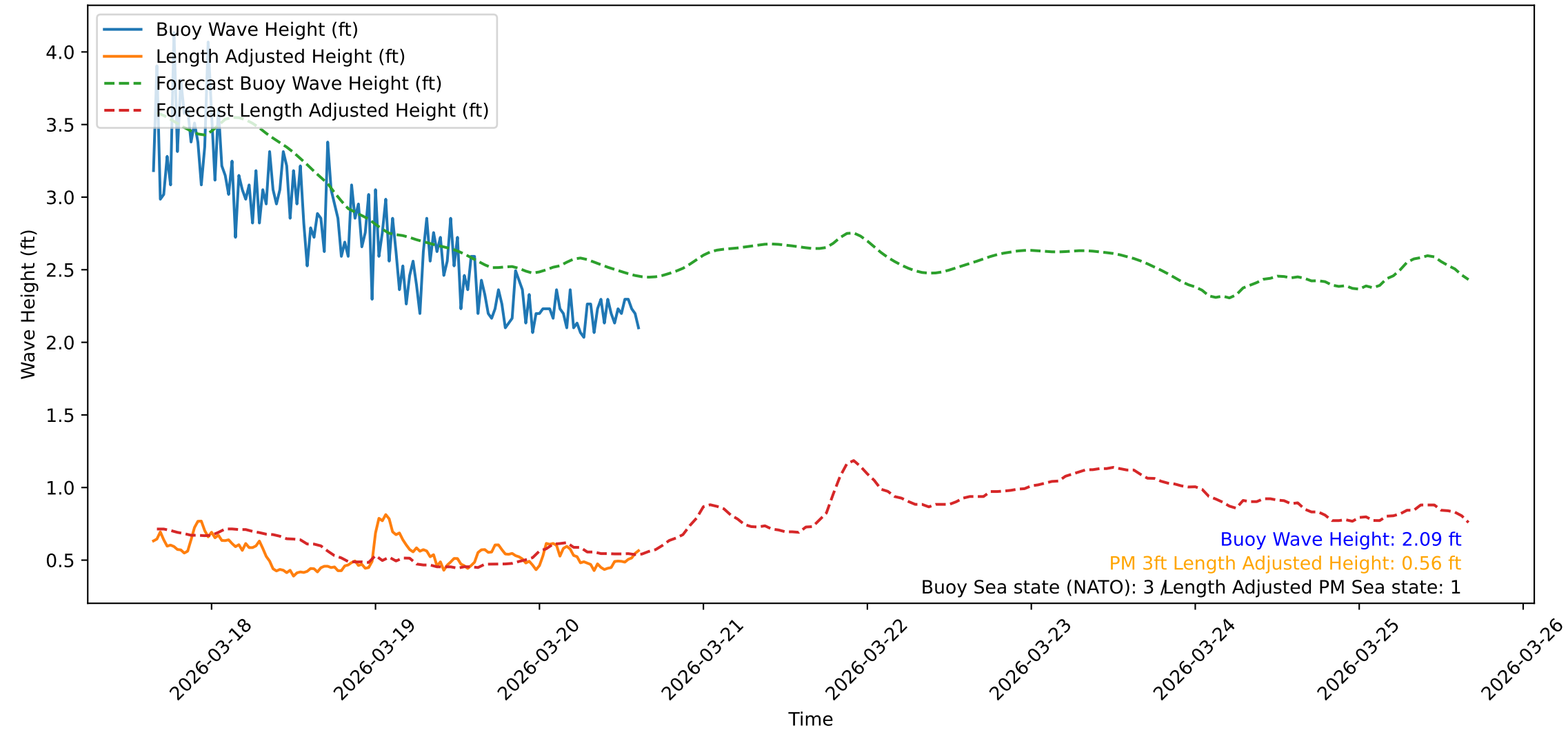
Wave Heights over Time for Green Beach at 2026-03-20 15:31:12
