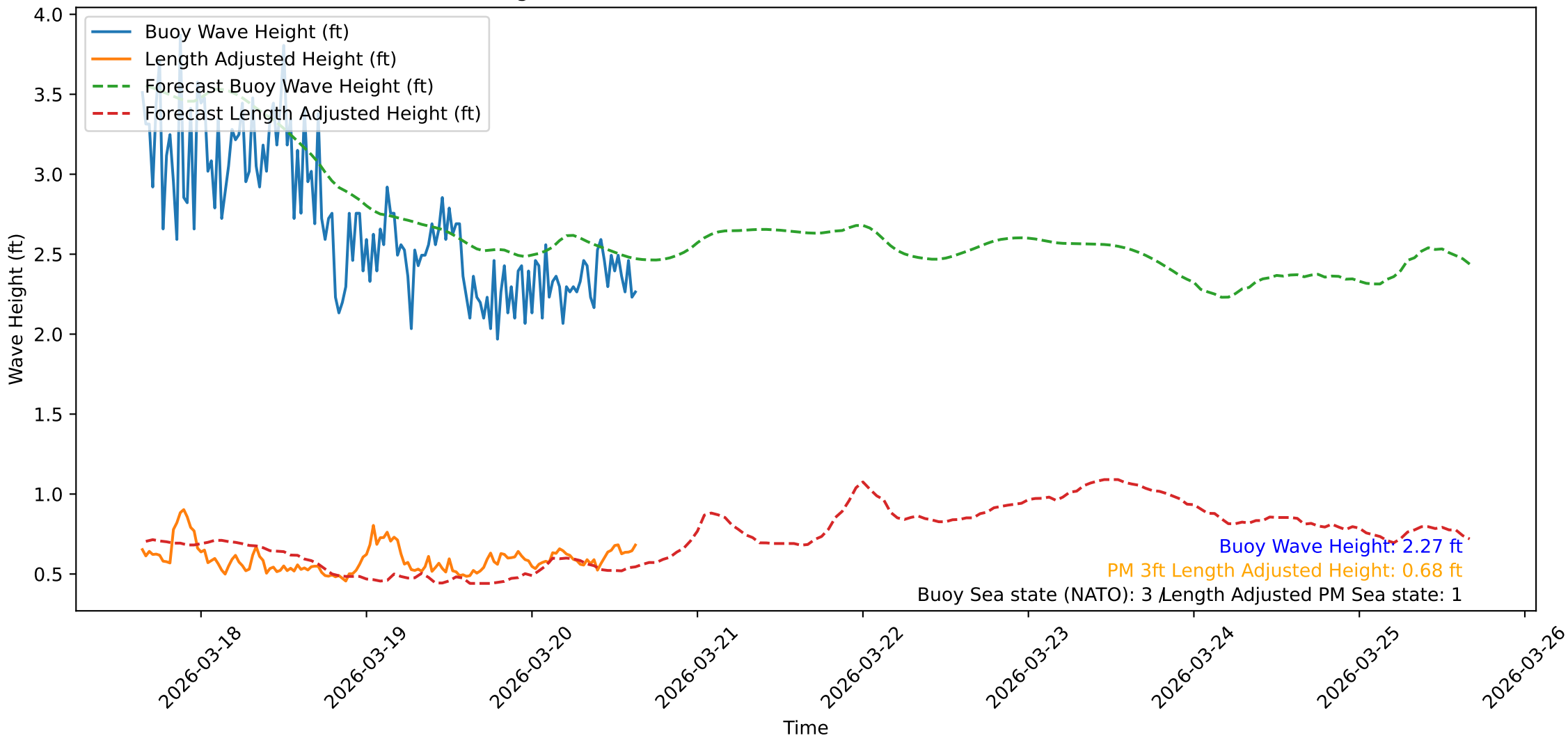
Wave Heights over Time for Oceanside Harbor at 2026-03-20 15:30:32
