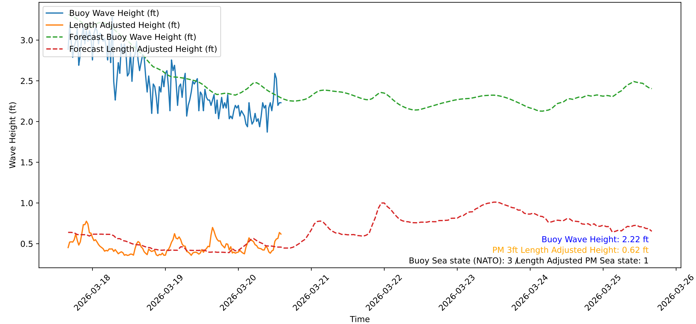
Wave Heights over Time for Red Beach at 2026-03-20 15:30:49
