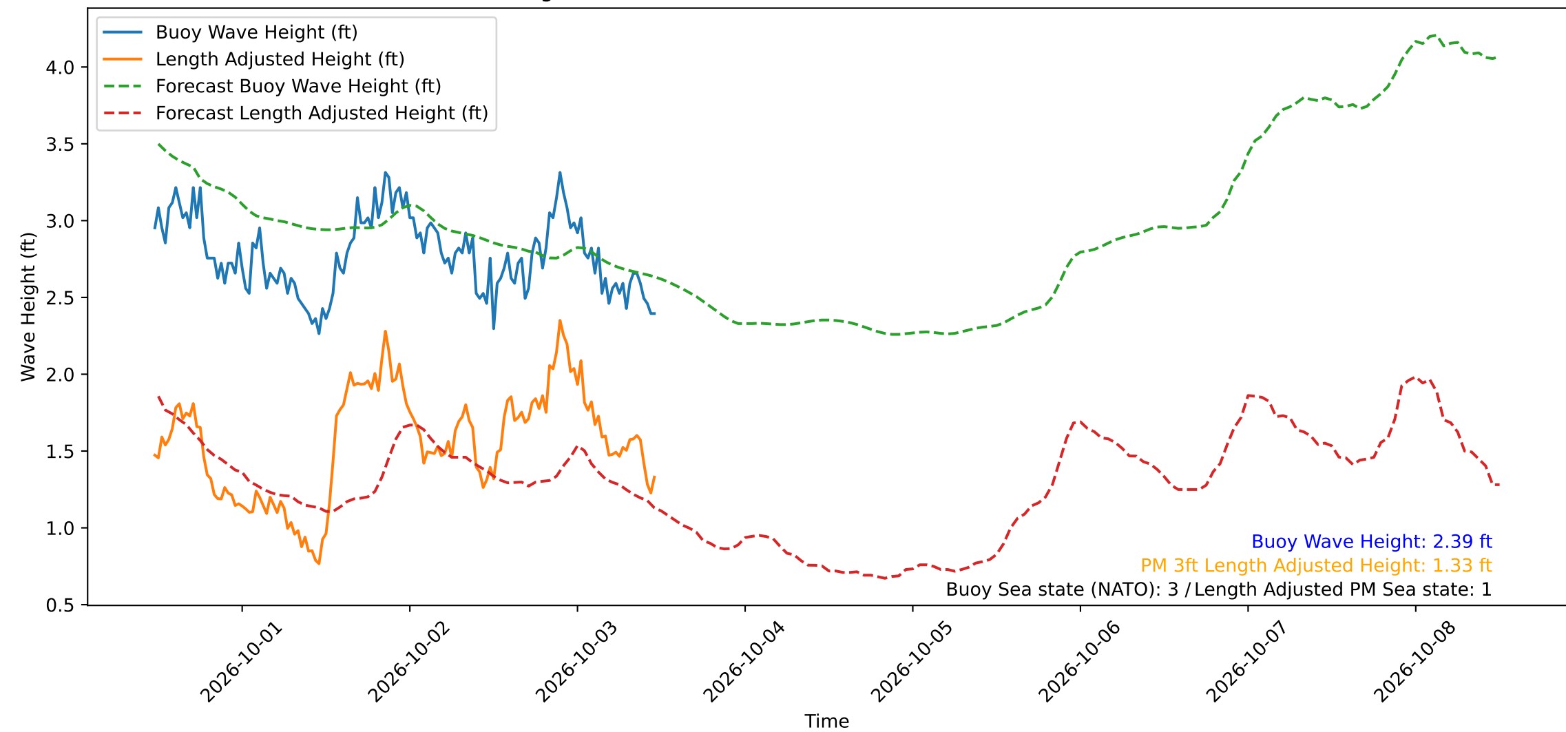
Wave Heights over Time for Oceanside Harbor at 2026-10-03 11:30:30
