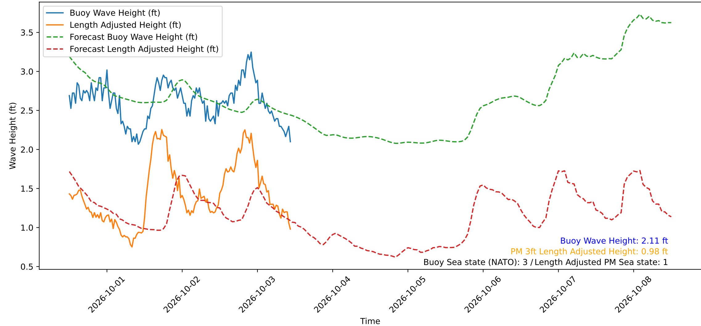
Wave Heights over Time for Red Beach at 2026-10-03 11:30:49
