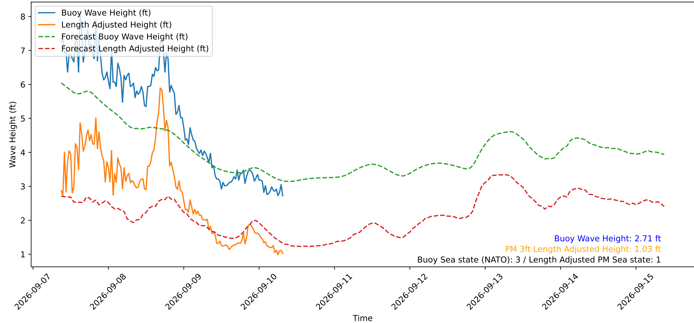
Wave Heights over Time for Green Beach at 2026-09-10 08:31:11
