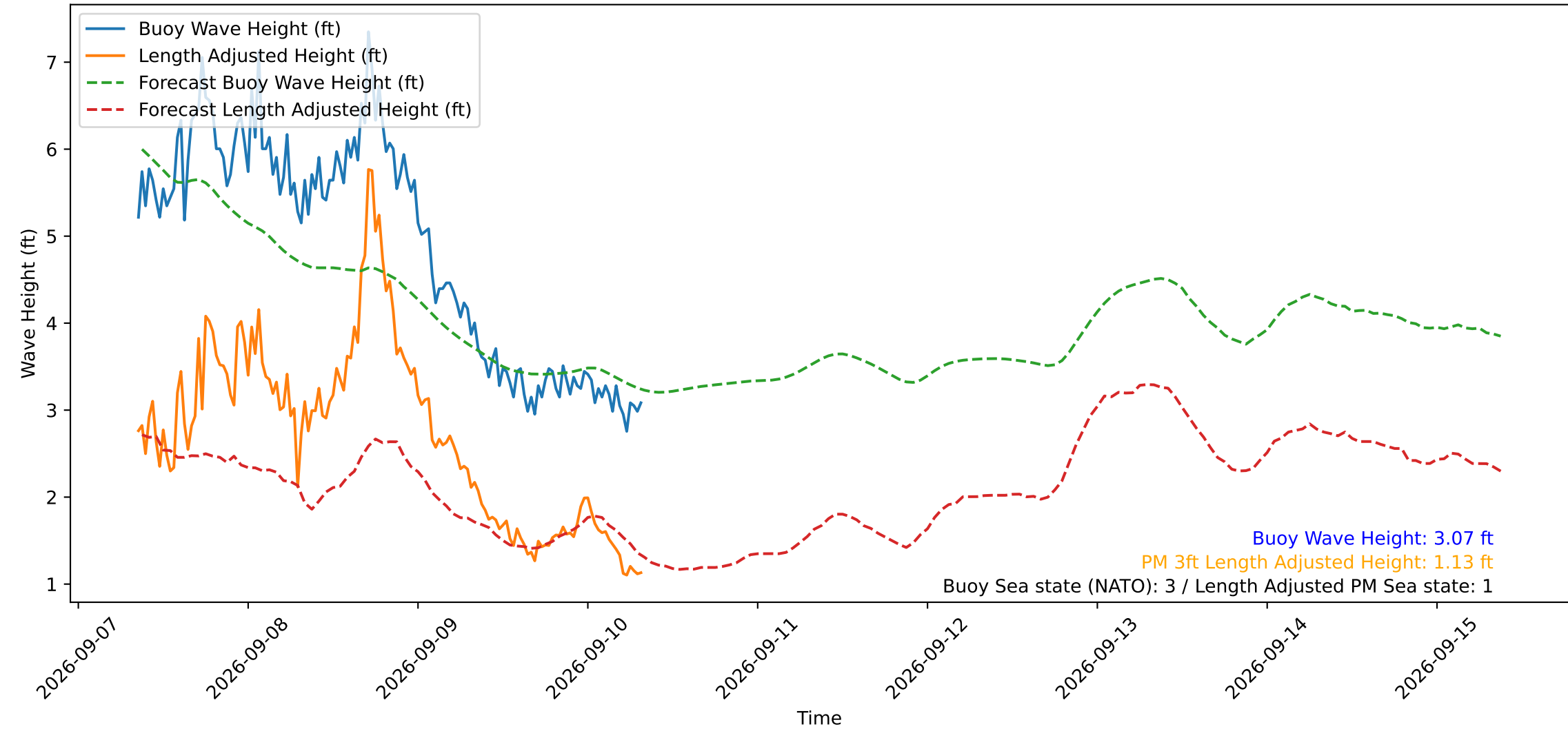
Wave Heights over Time for Oceanside Harbor at 2026-09-10 08:30:29
