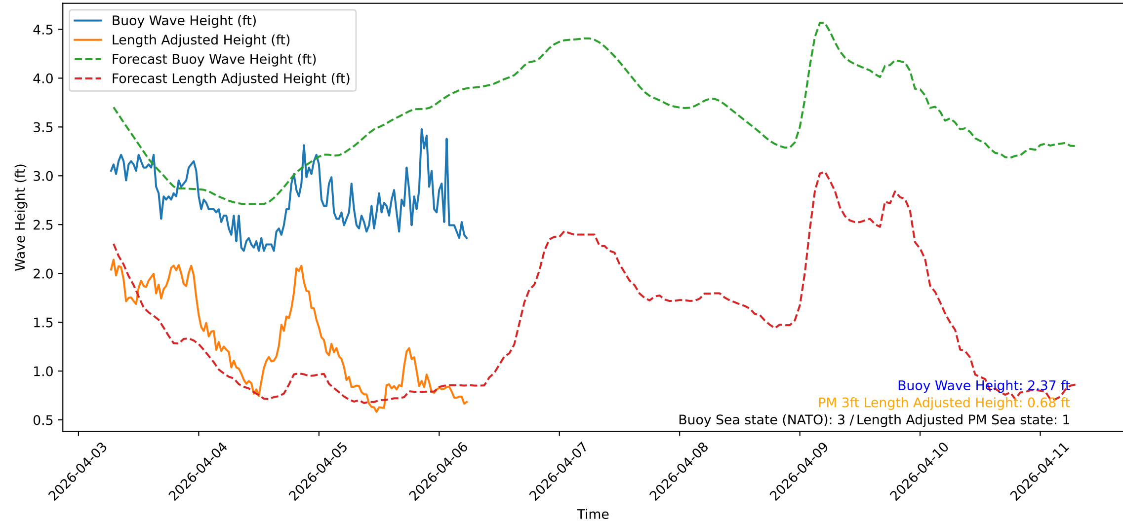
Wave Heights over Time for Green Beach at 2026-04-06 06:31:09
