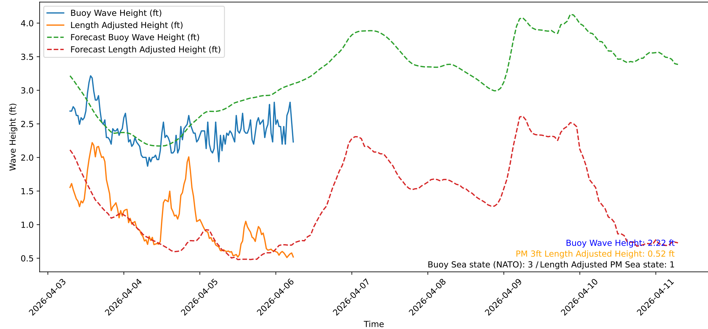
Wave Heights over Time for Red Beach at 2026-04-06 06:30:47
