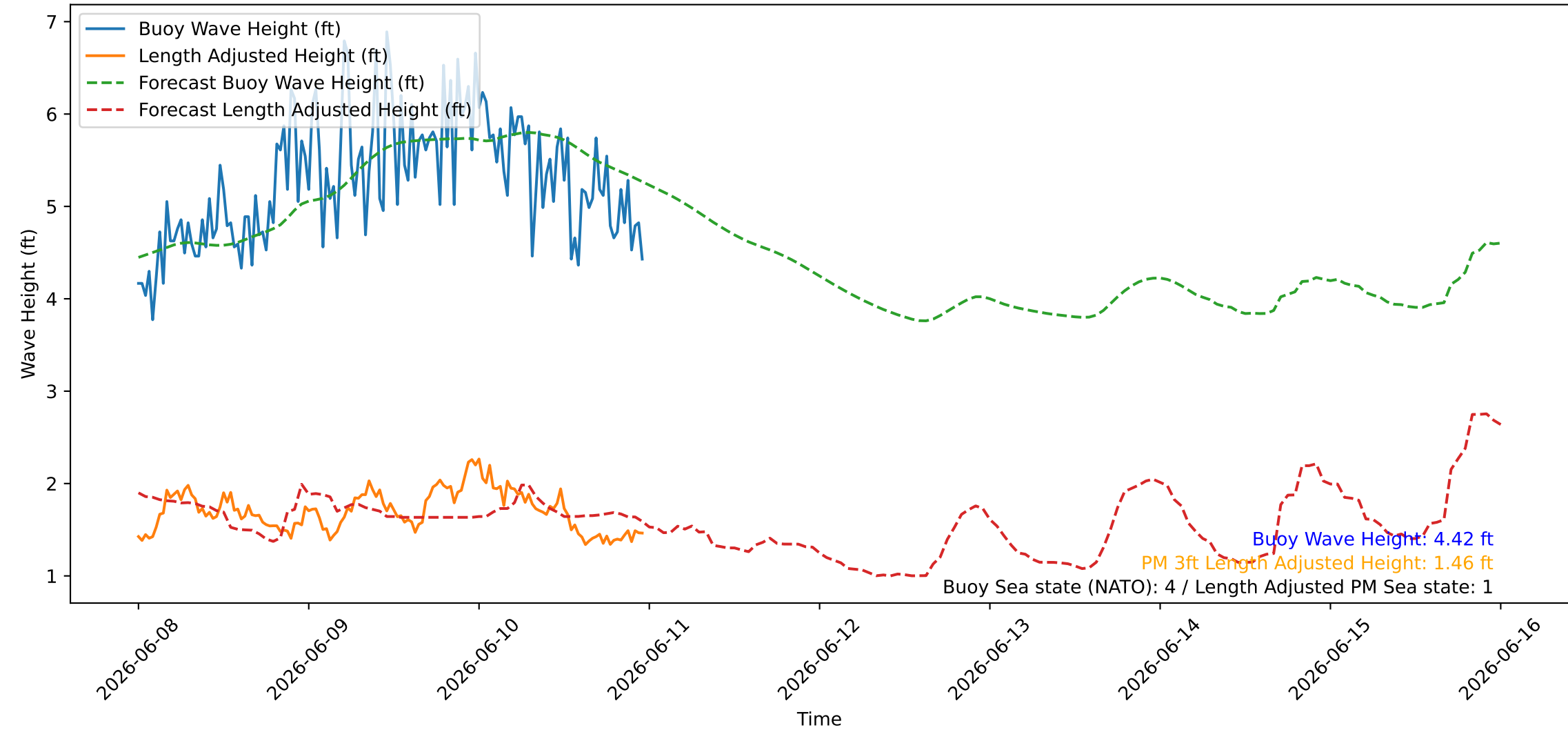
Wave Heights over Time for Green Beach at 2026-06-11 00:01:10
