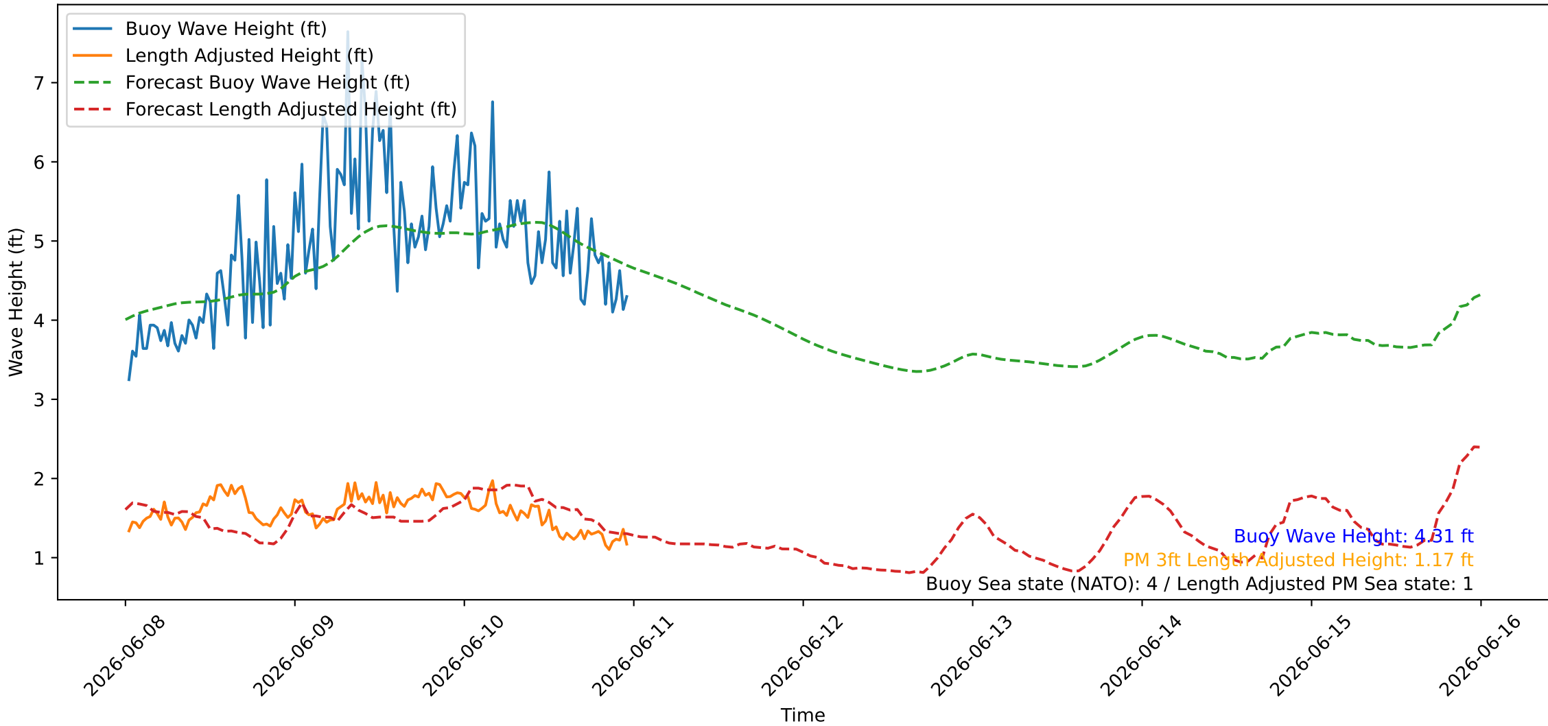
Wave Heights over Time for Red Beach at 2026-06-11 00:00:46
