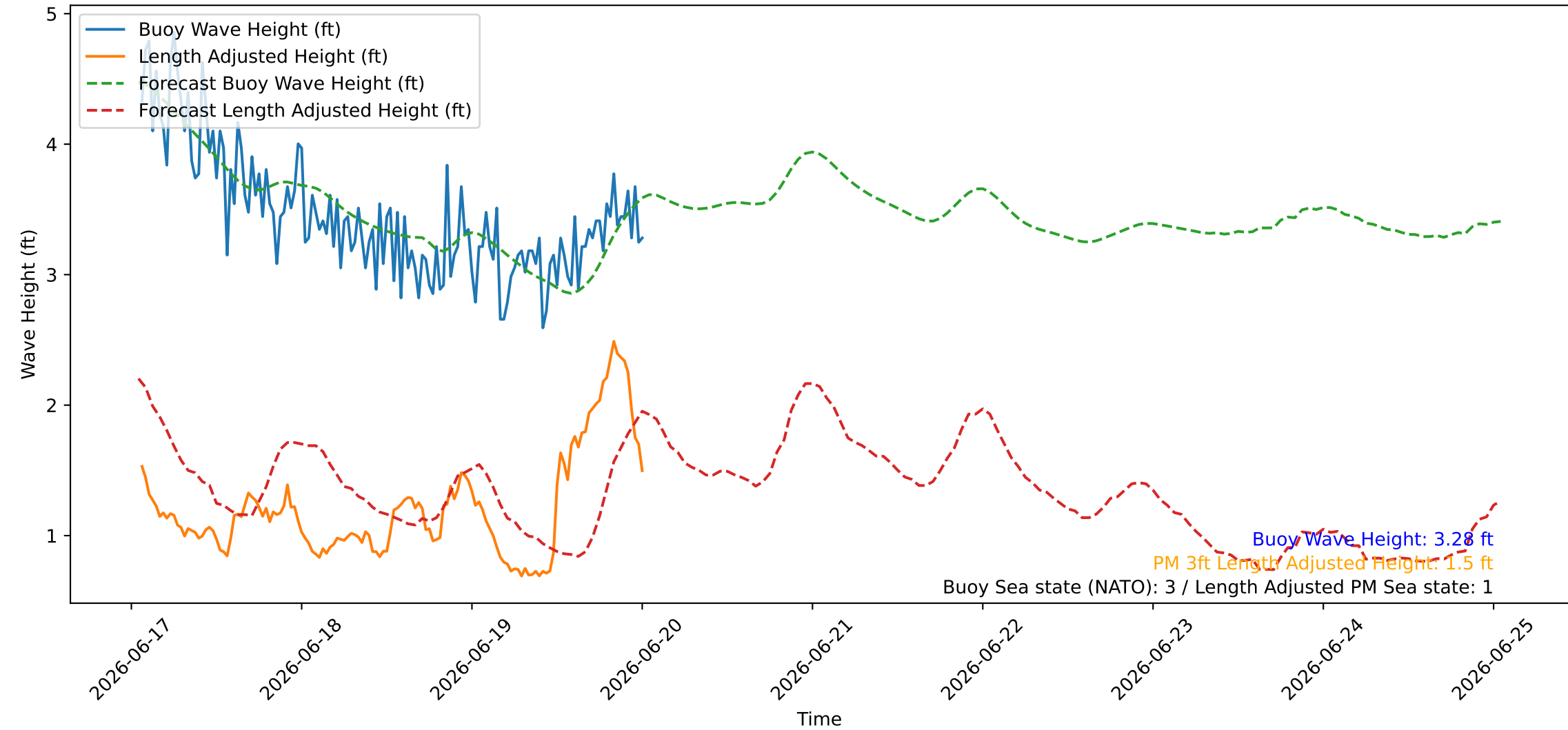
Wave Heights over Time for Red Beach at 2026-06-20 01:00:45
