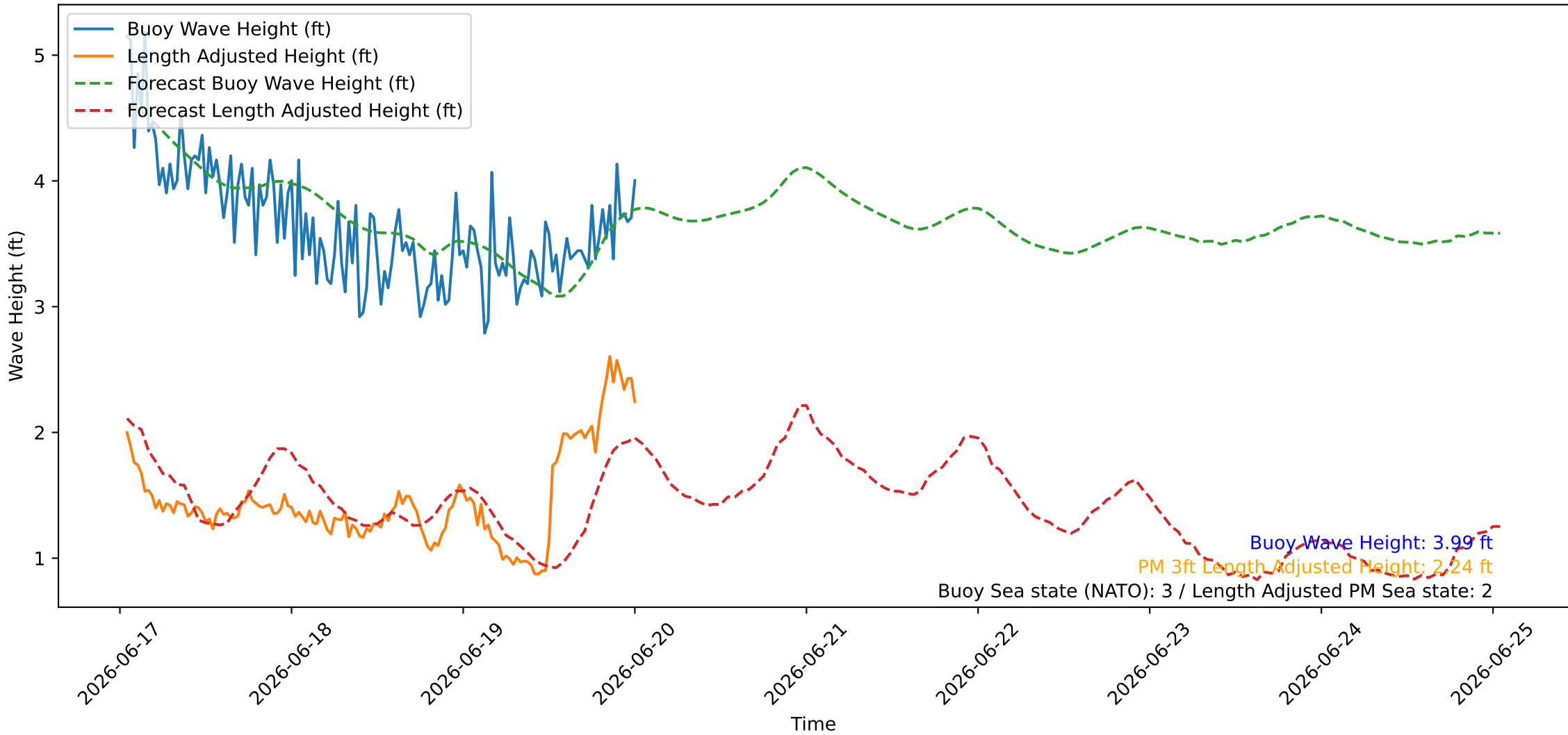
Wave Heights over Time for Oceanside Harbor at 2026-06-20 01:00:26
