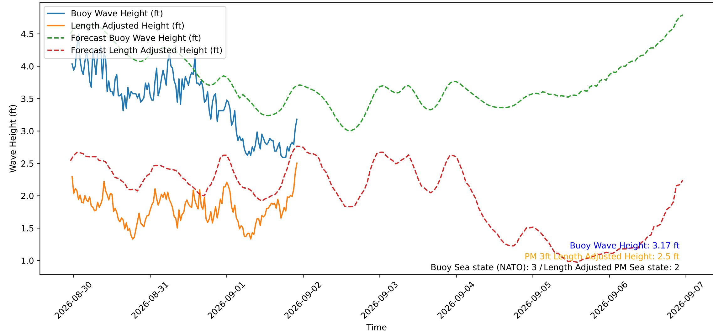
Wave Heights over Time for Red Beach at 2026-09-01 23:00:49
