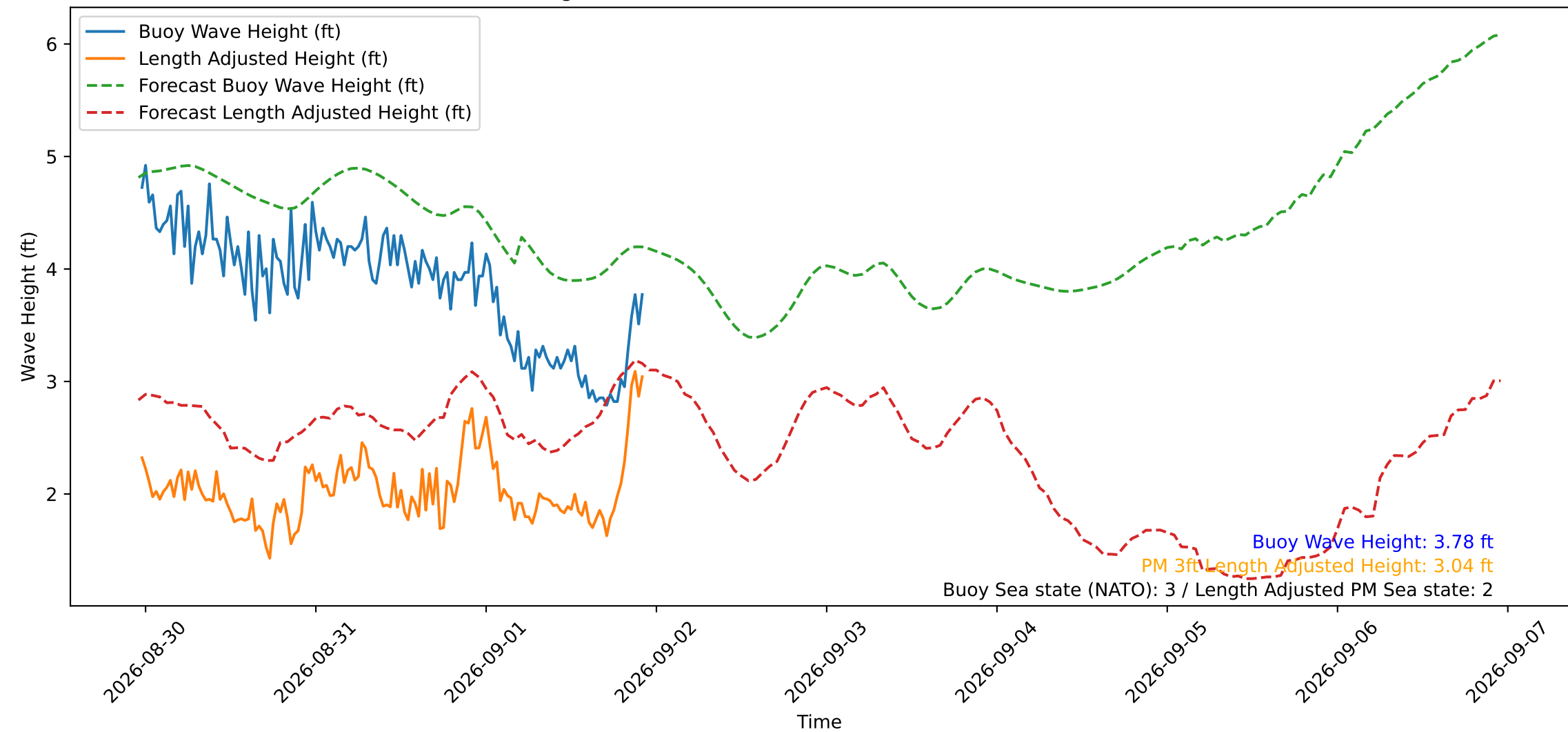
Wave Heights over Time for Green Beach at 2026-09-01 23:01:12
