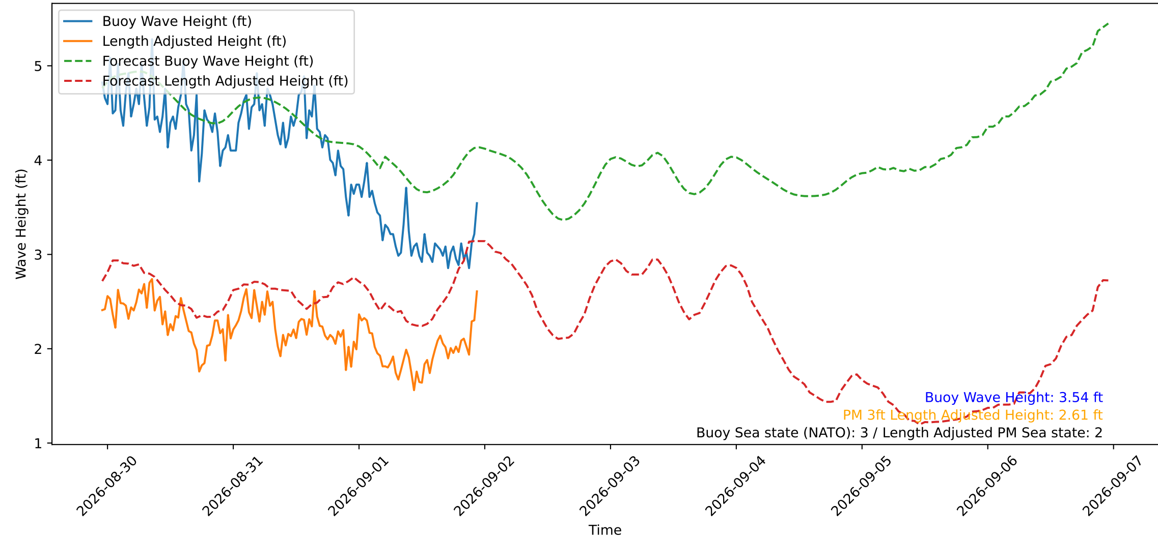
Wave Heights over Time for Oceanside Harbor at 2026-09-01 23:00:30
