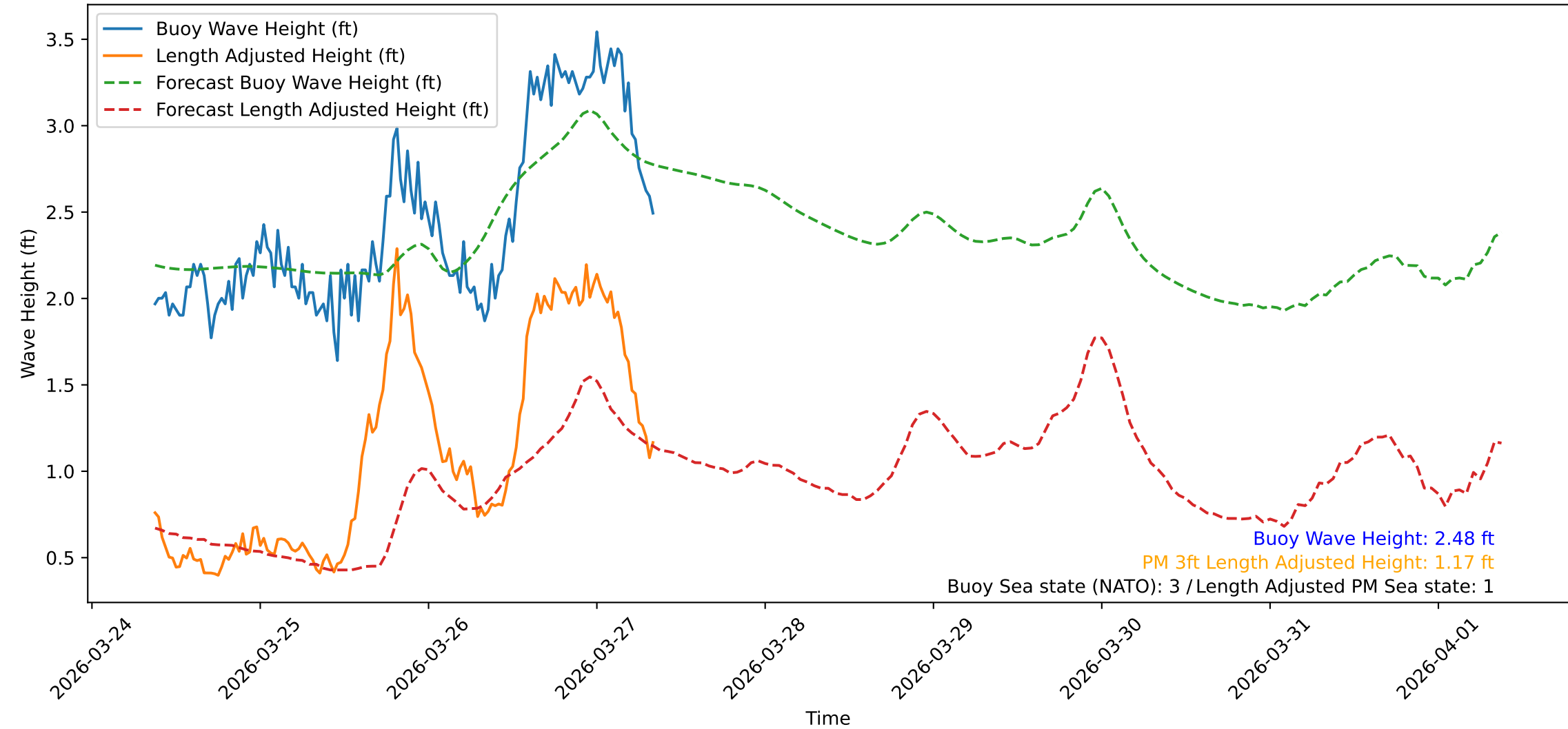
Wave Heights over Time for Green Beach at 2026-03-27 08:51:09
