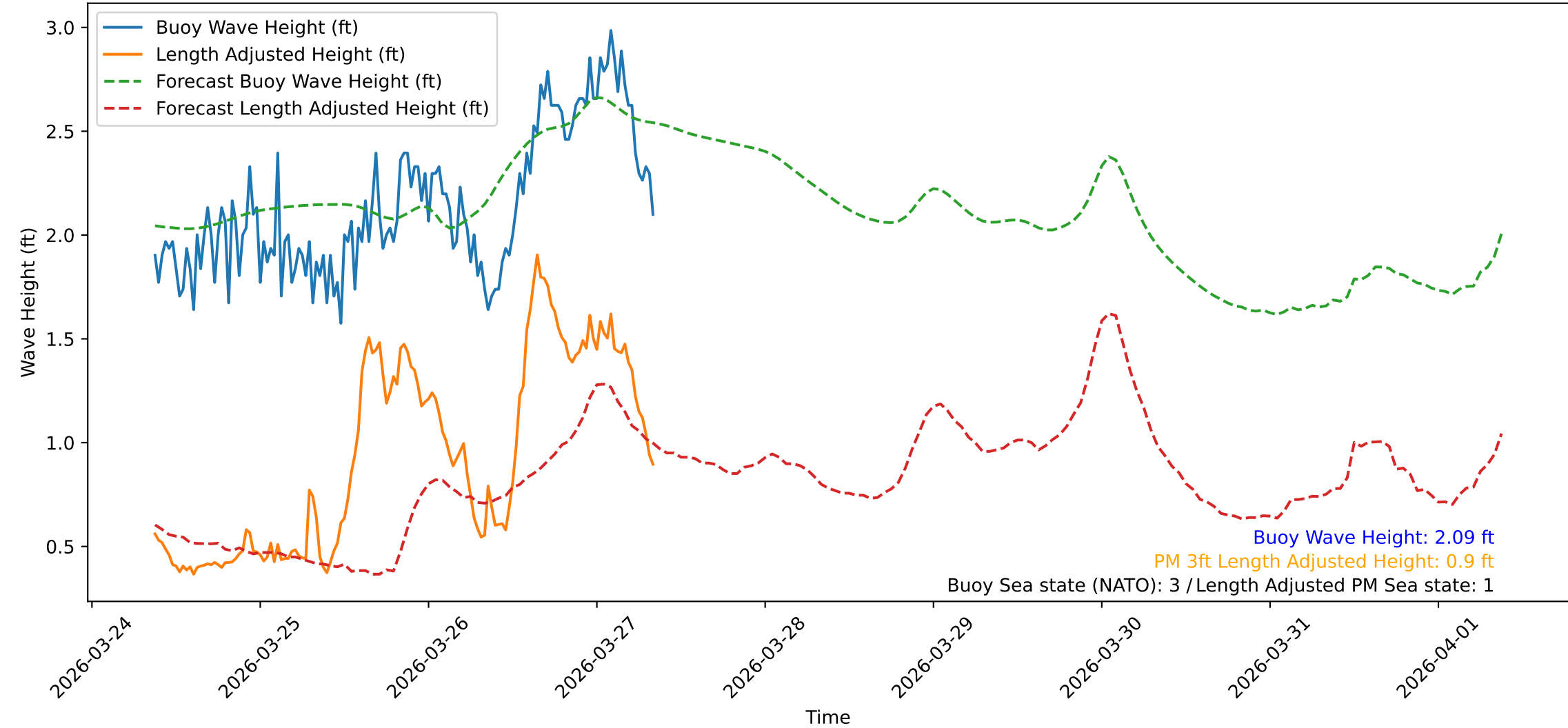
Wave Heights over Time for Red Beach at 2026-03-27 08:50:47
