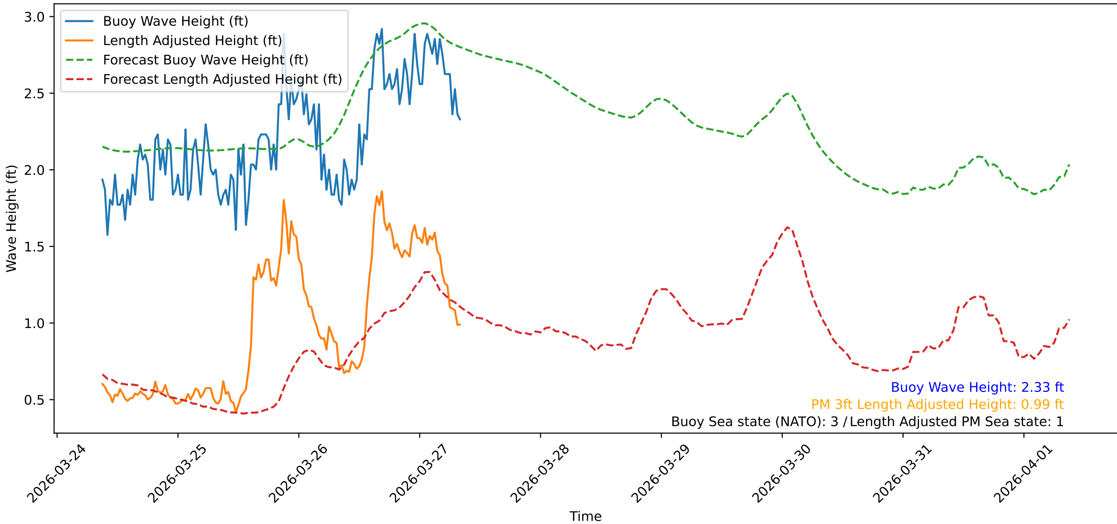
Wave Heights over Time for Oceanside Harbor at 2026-03-27 08:50:31
