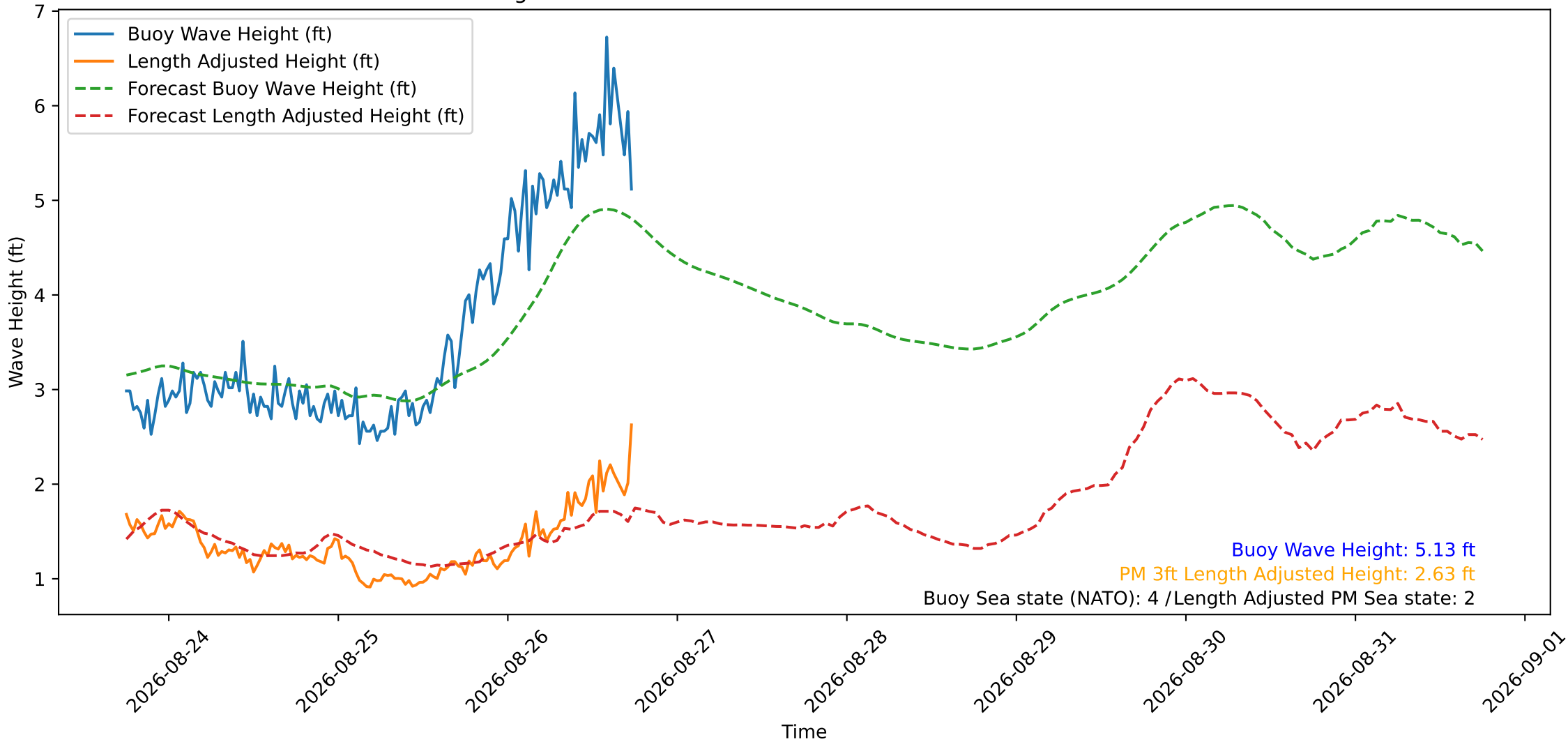
Wave Heights over Time for Oceanside Harbor at 2026-08-26 18:10:30
