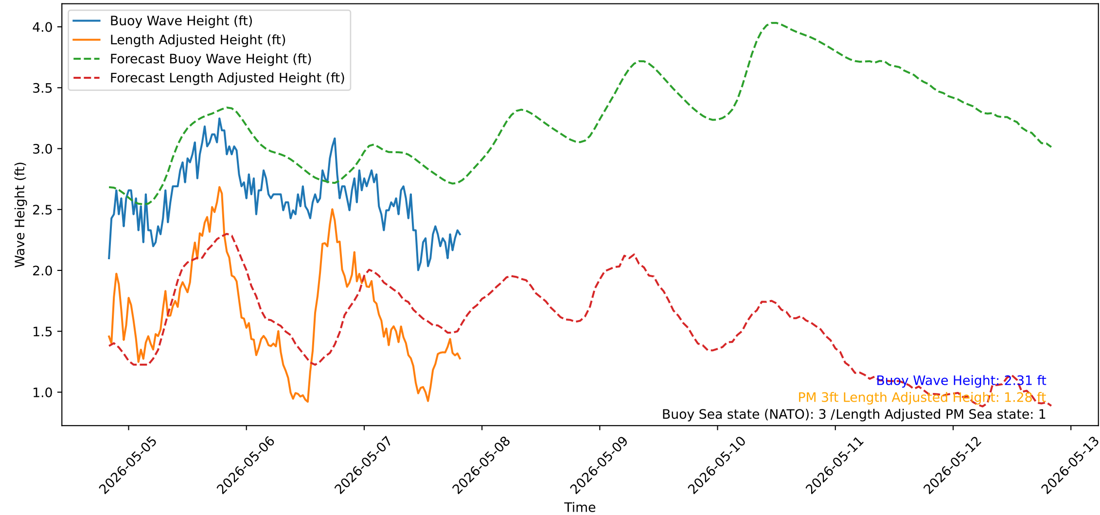
Wave Heights over Time for Oceanside Harbor at 2026-05-07 20:10:32
