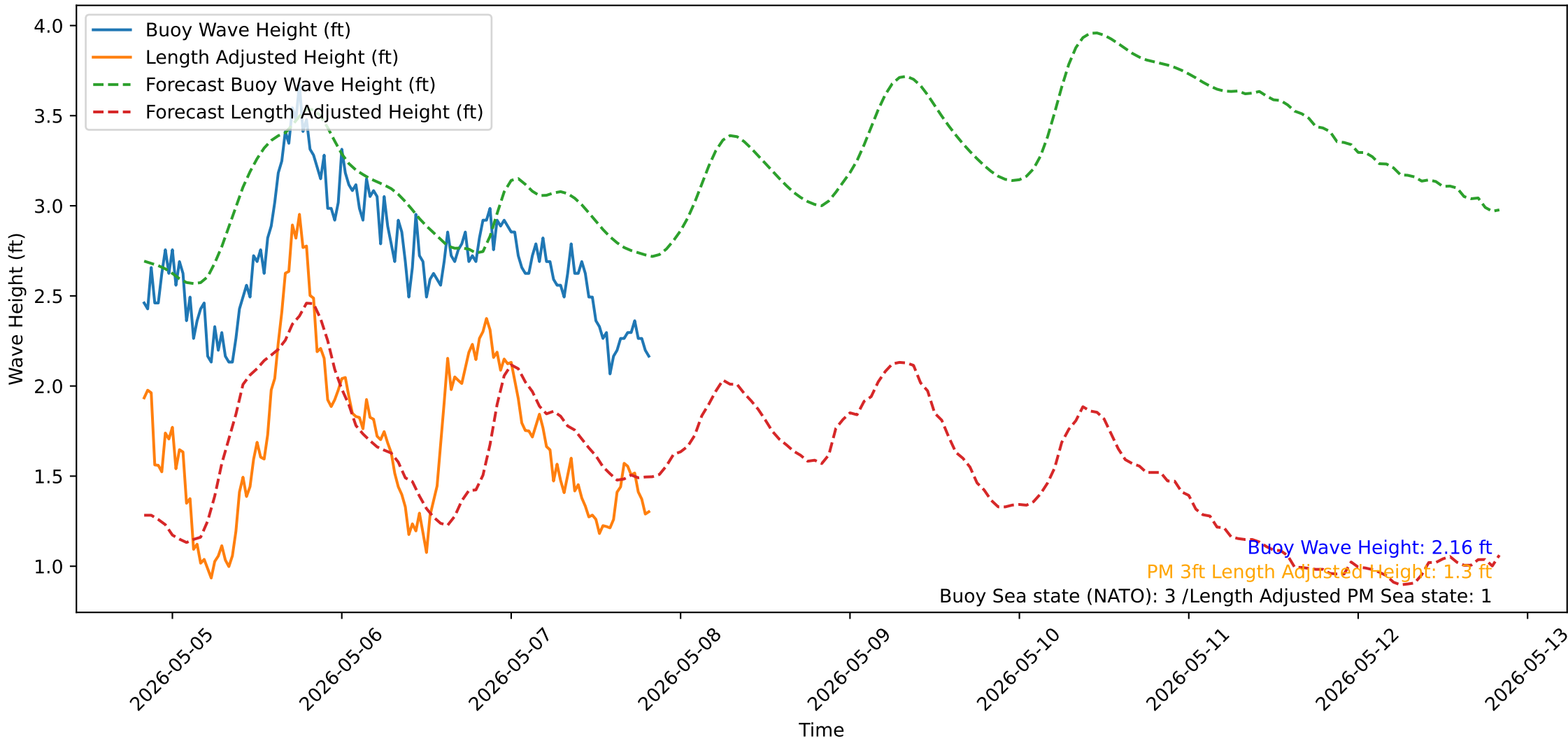
Wave Heights over Time for Green Beach at 2026-05-07 20:11:13
