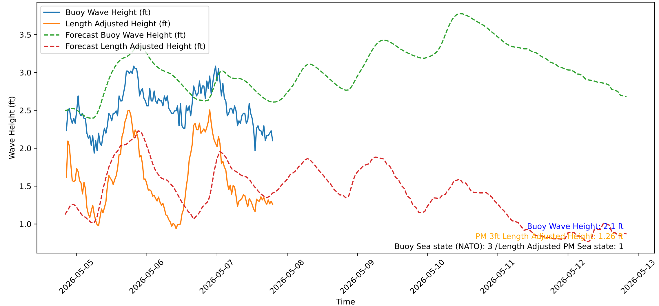
Wave Heights over Time for Red Beach at 2026-05-07 20:10:51
