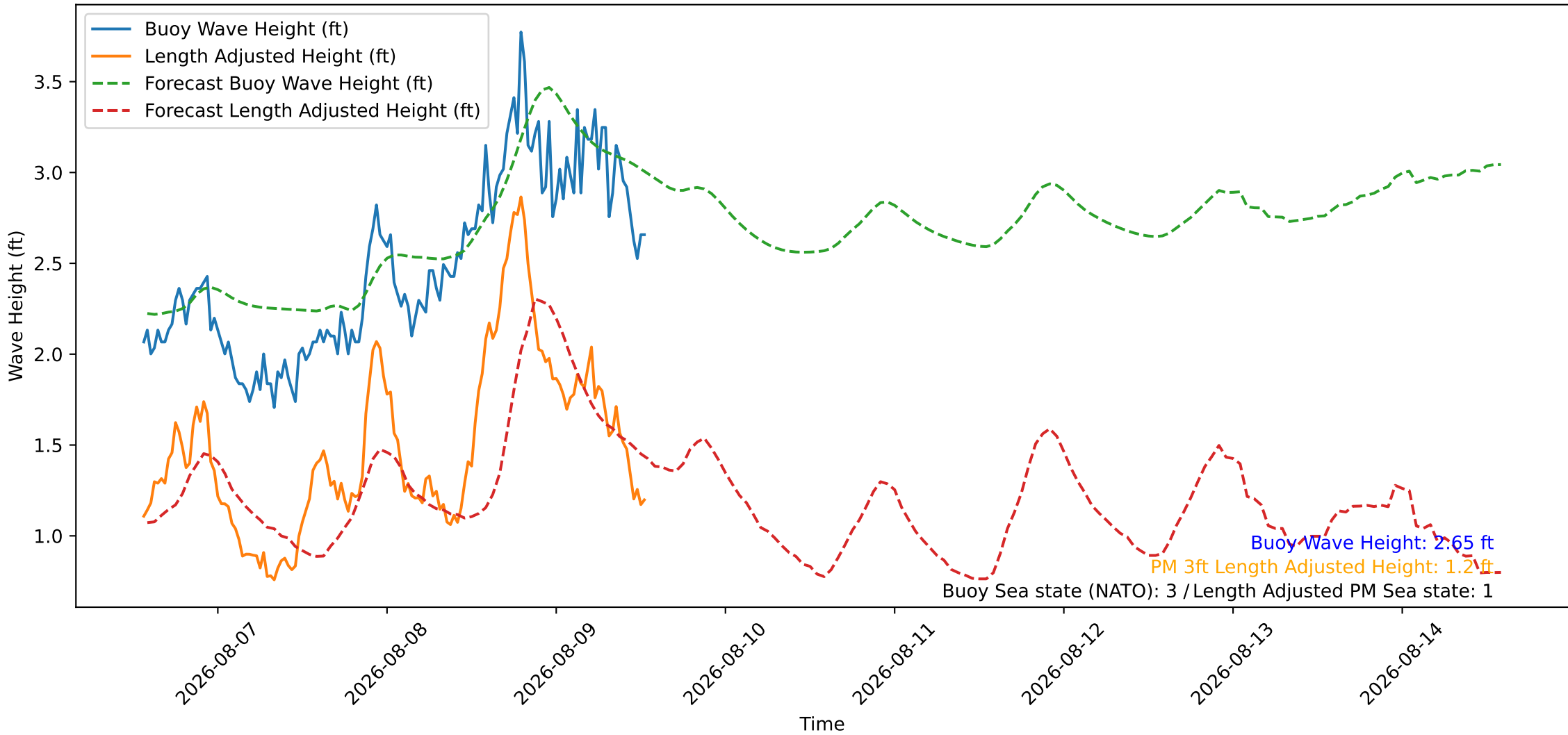
Wave Heights over Time for Green Beach at 2026-08-09 13:31:08
