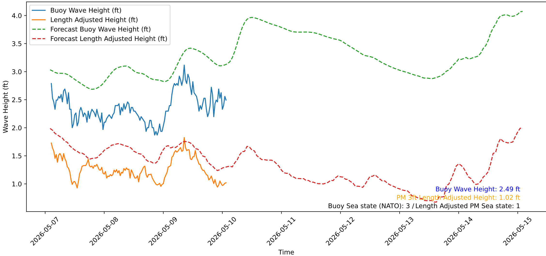
Wave Heights over Time for Oceanside Harbor at 2026-05-10 02:20:32
