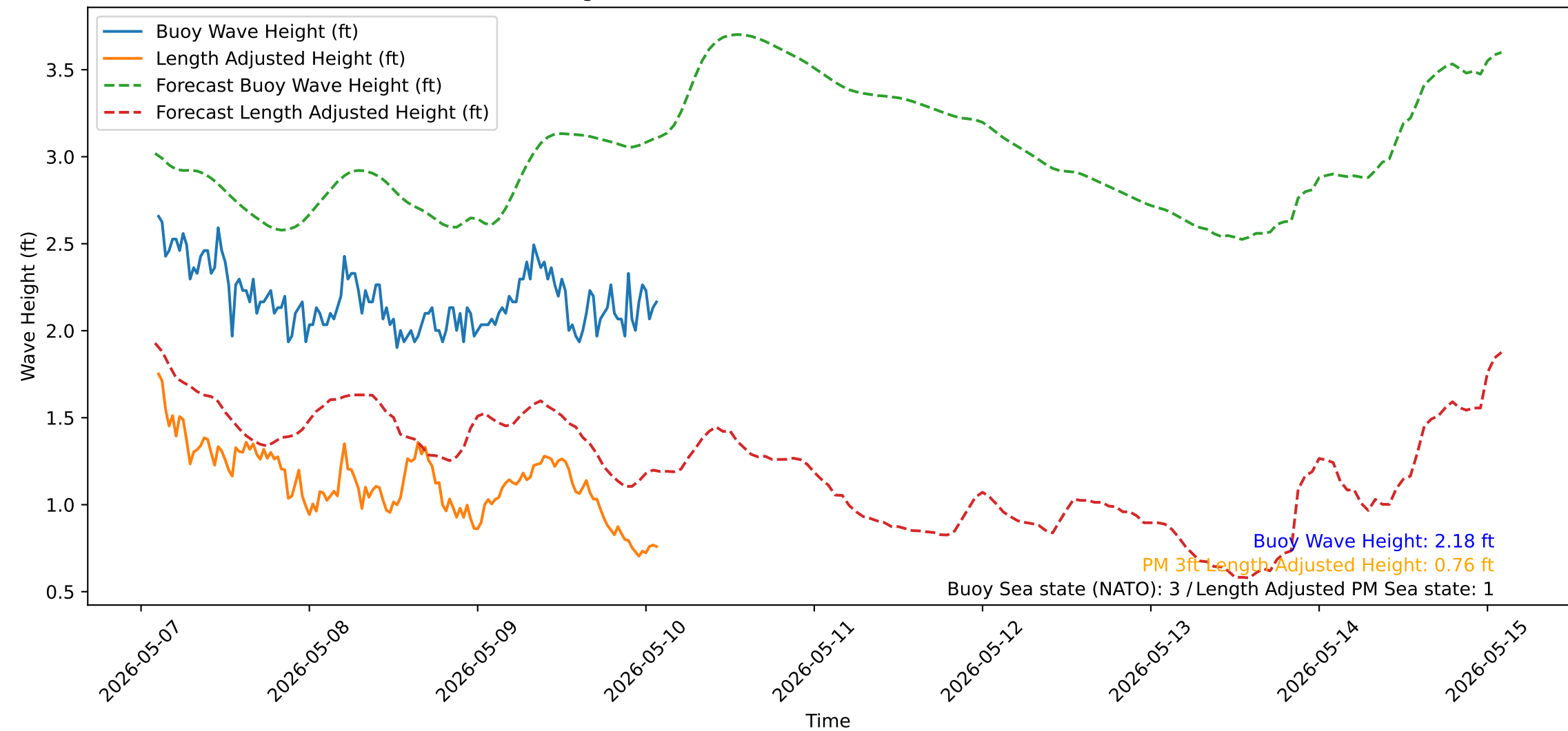
Wave Heights over Time for Red Beach at 2026-05-10 02:20:53
