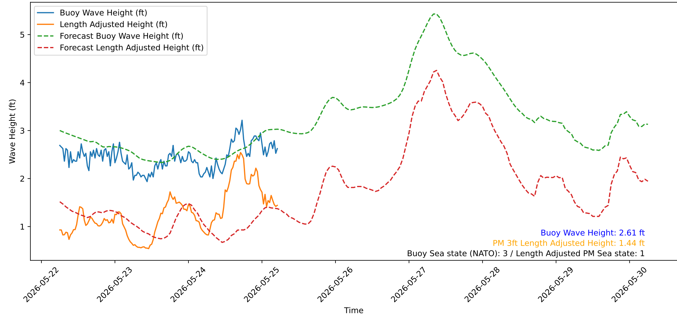
Wave Heights over Time for Red Beach at 2026-05-25 05:50:51
