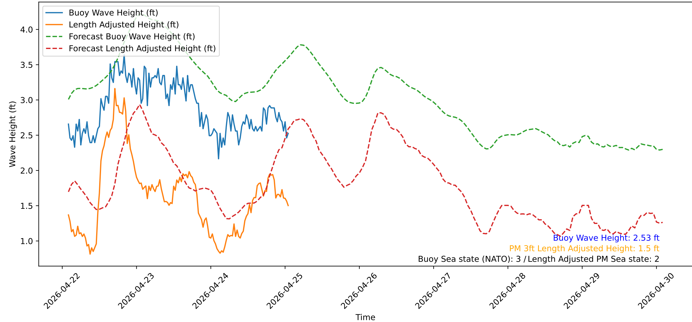
Wave Heights over Time for Red Beach at 2026-04-25 01:50:51
