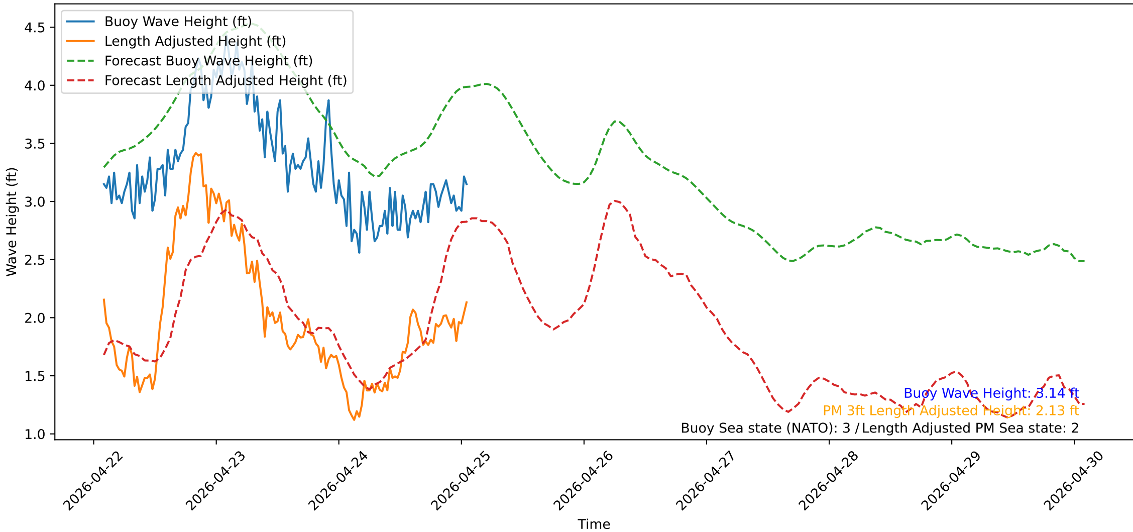
Wave Heights over Time for Oceanside Harbor at 2026-04-25 01:50:31
