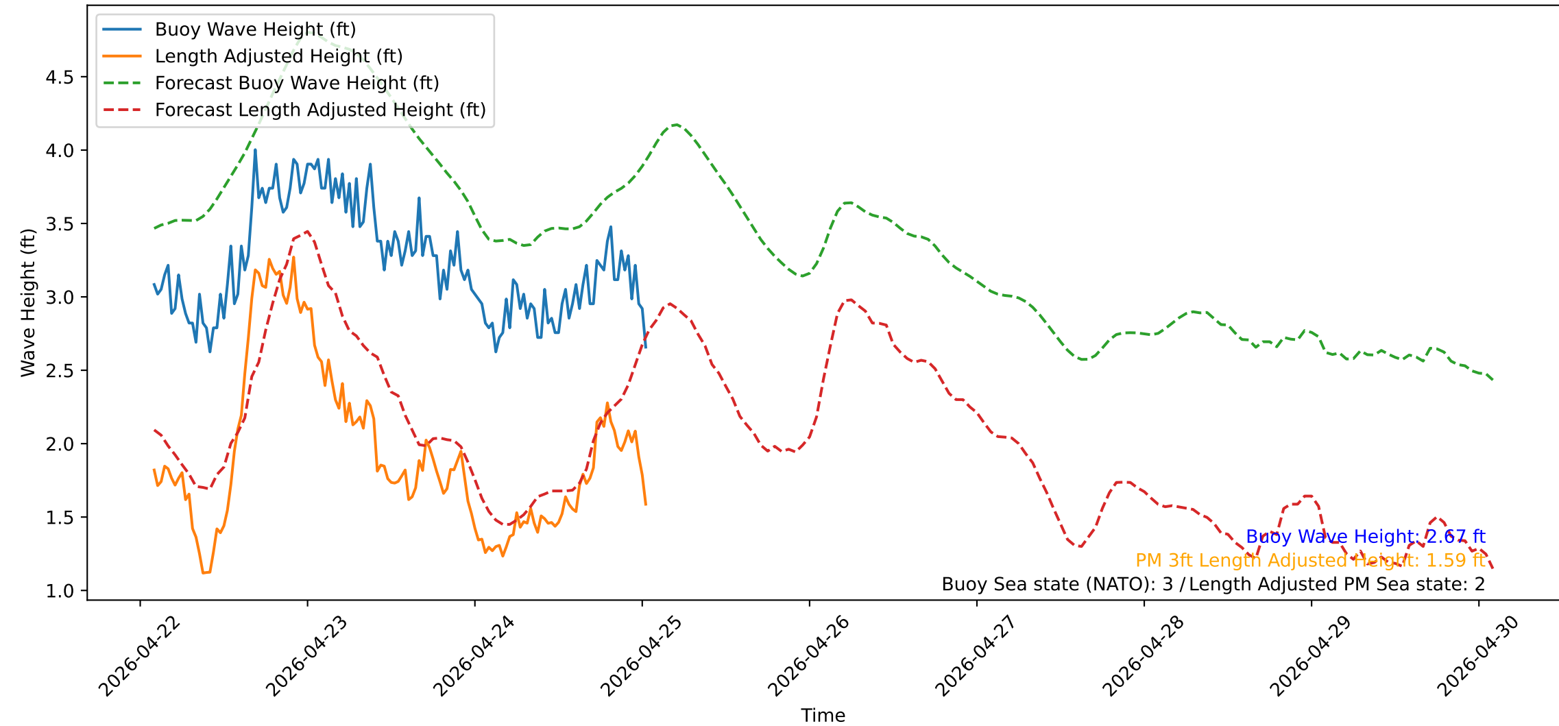
Wave Heights over Time for Green Beach at 2026-04-25 01:51:13
