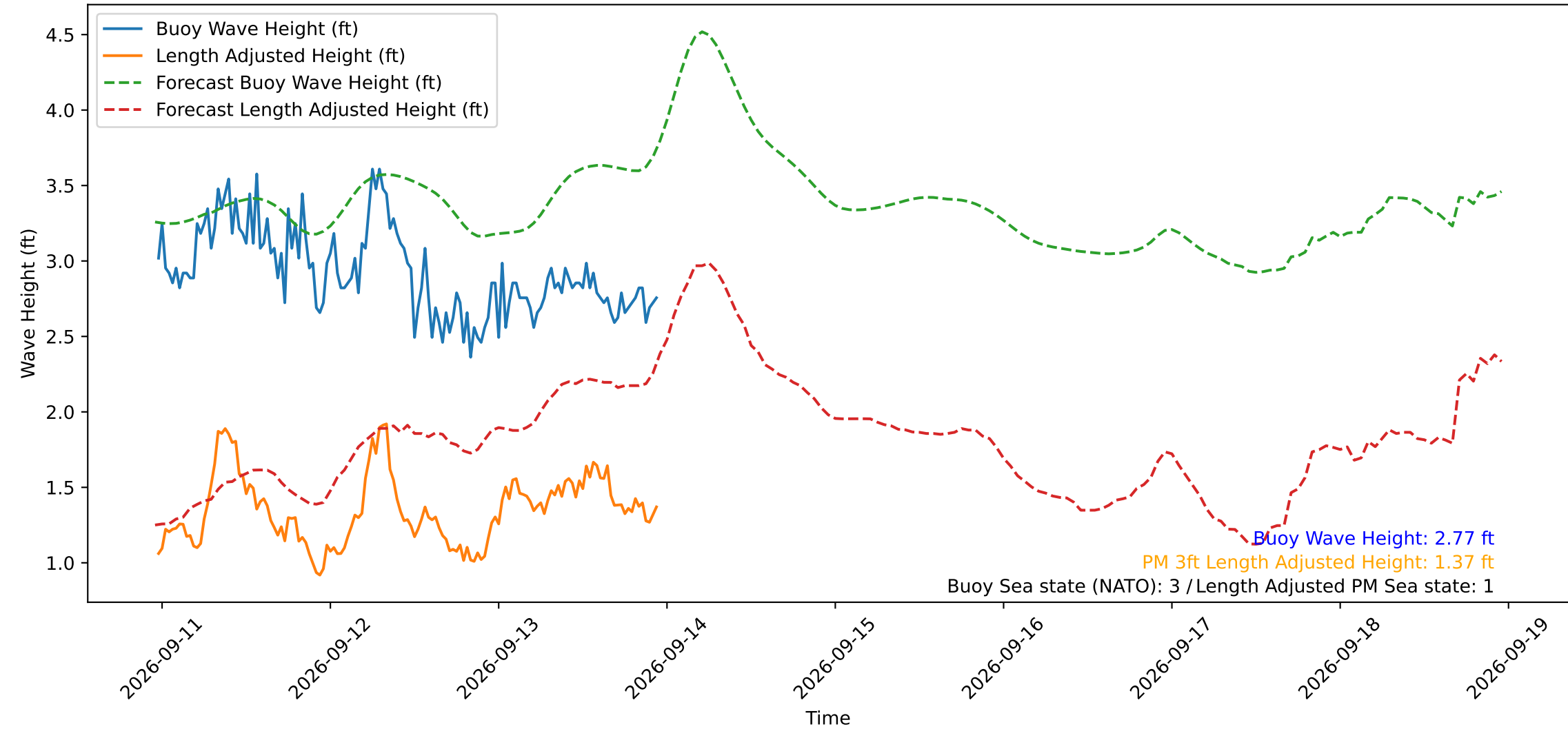
Wave Heights over Time for Green Beach at 2026-09-13 23:11:11
