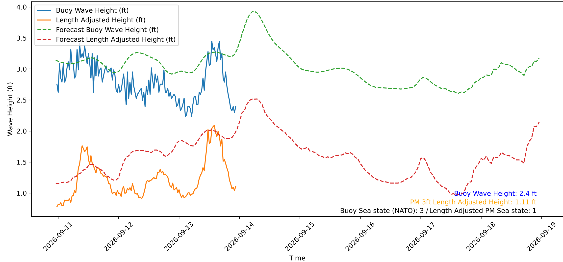
Wave Heights over Time for Red Beach at 2026-09-13 23:10:48
