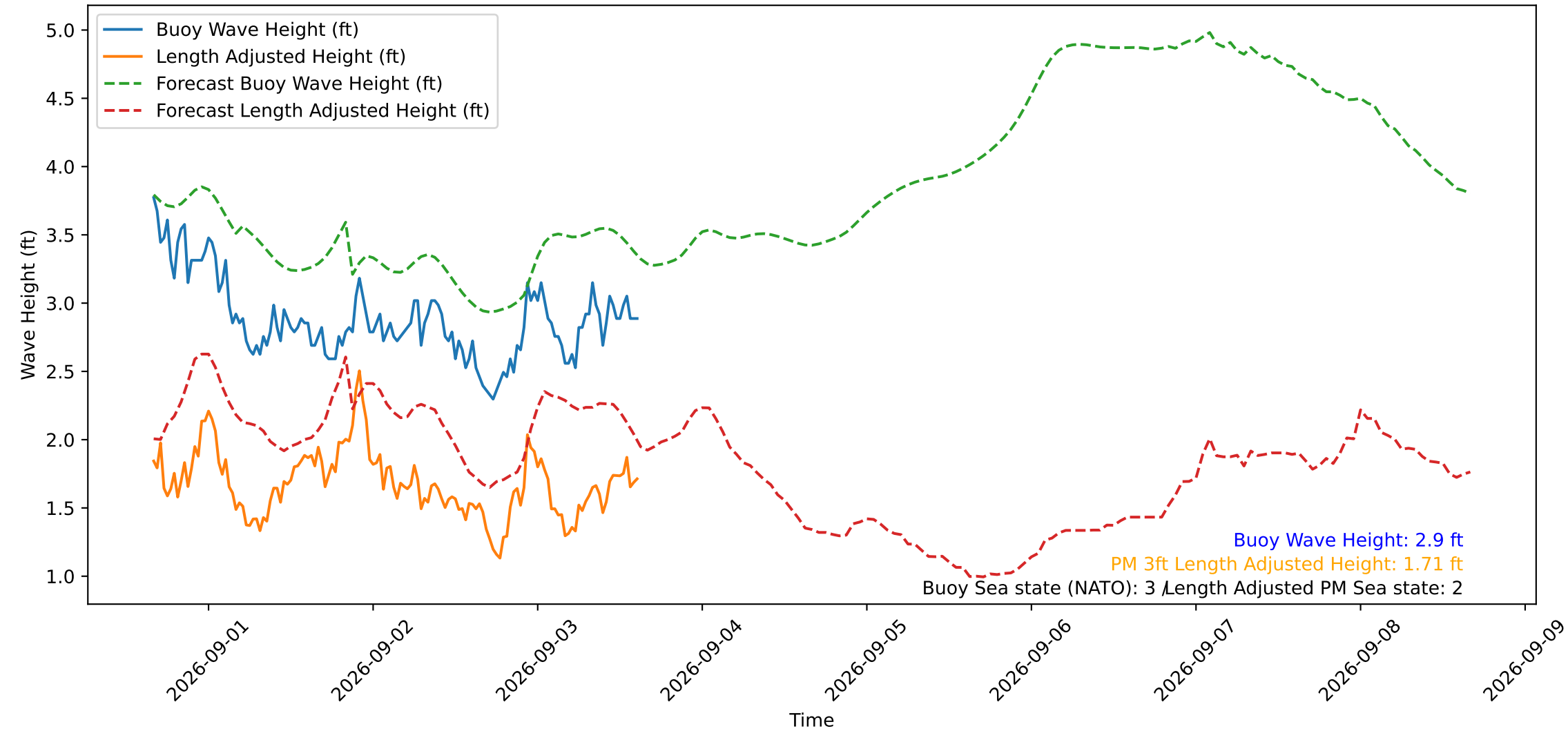
Wave Heights over Time for Red Beach at 2026-09-03 15:30:50
