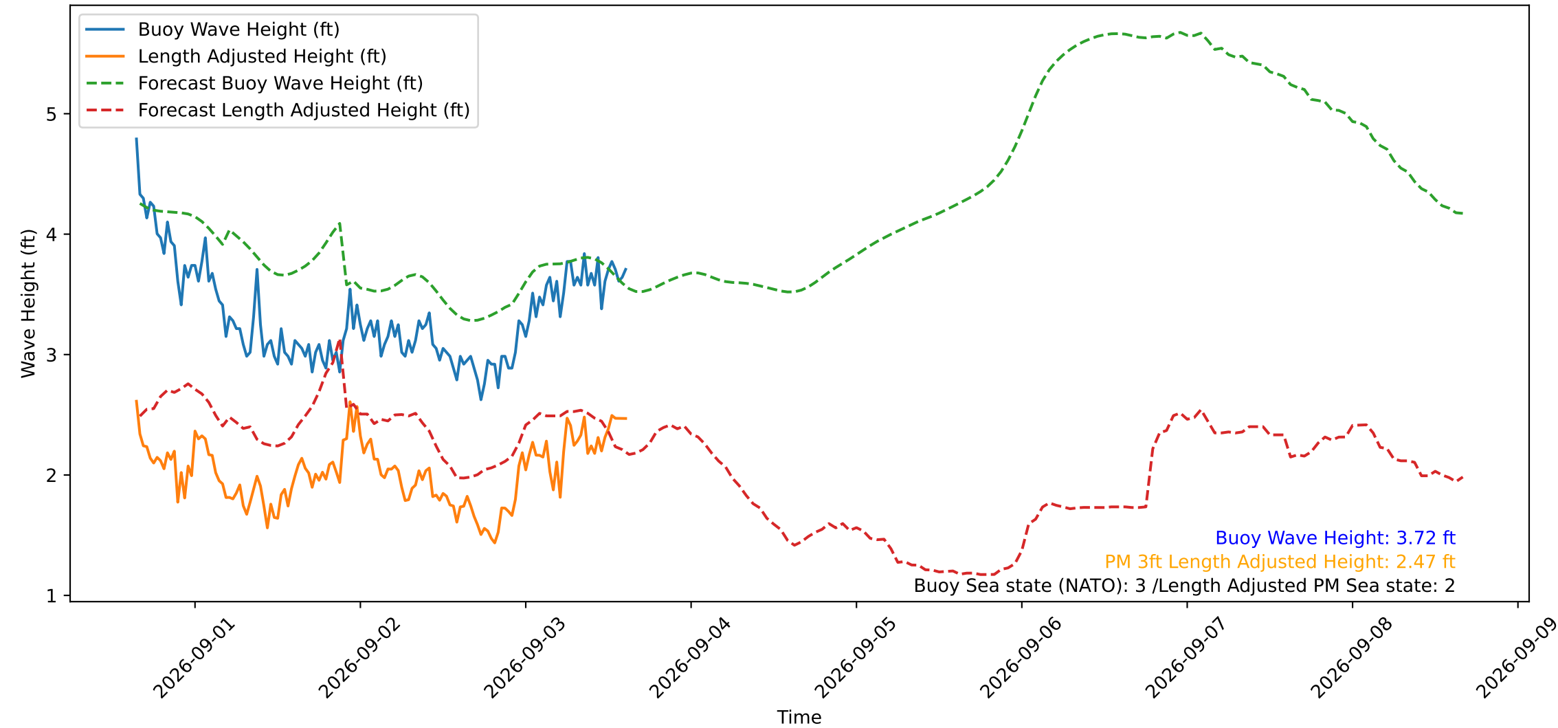
Wave Heights over Time for Oceanside Harbor at 2026-09-03 15:30:30
