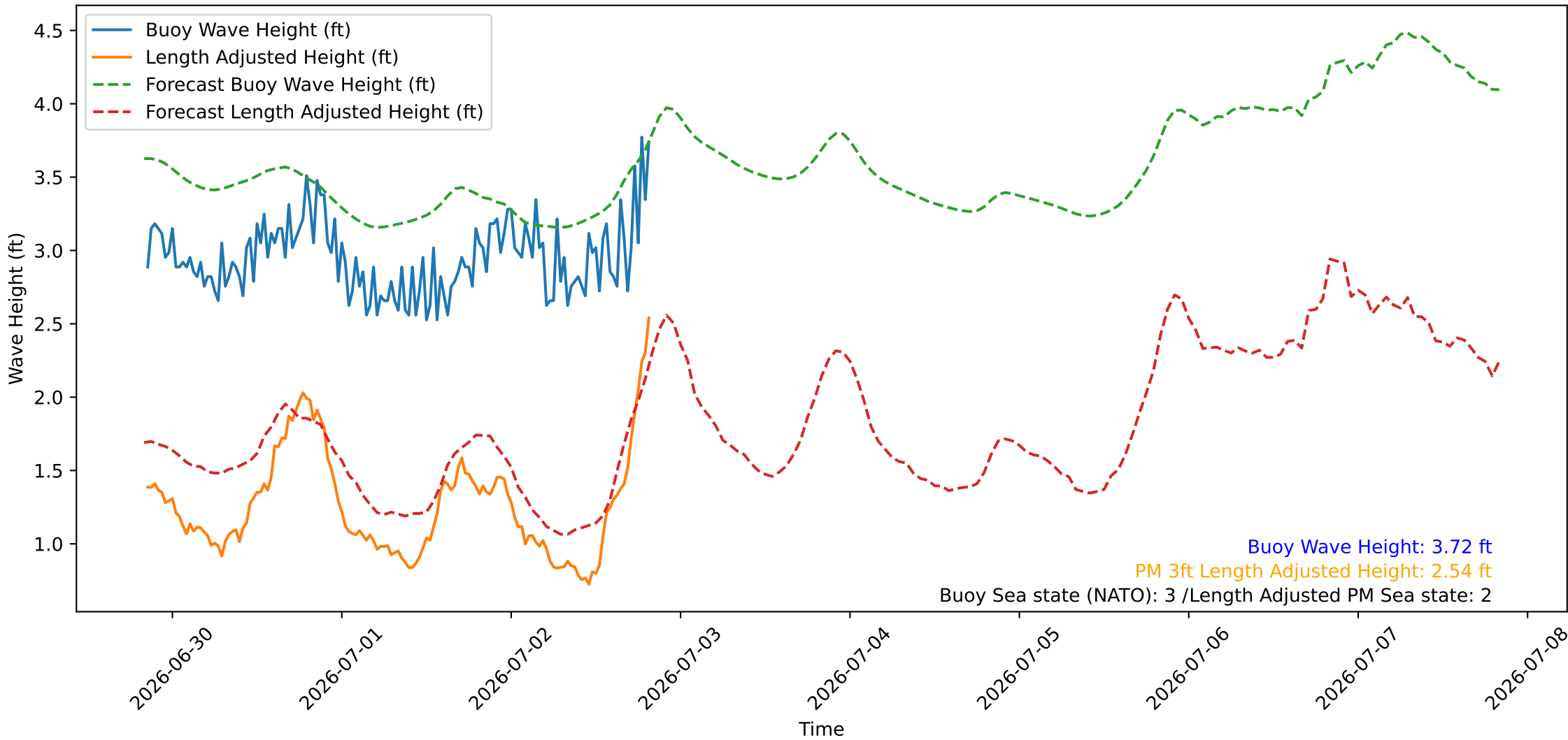
Wave Heights over Time for Green Beach at 2026-07-02 20:21:09
