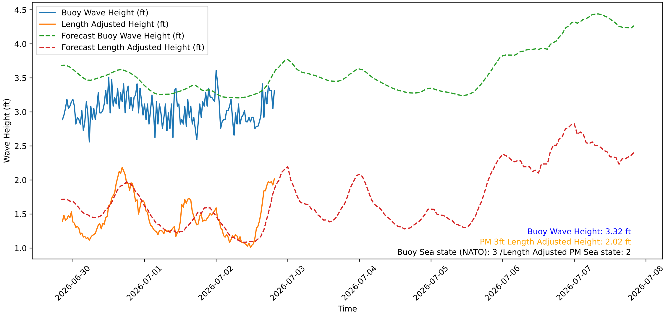
Wave Heights over Time for Oceanside Harbor at 2026-07-02 20:20:26
