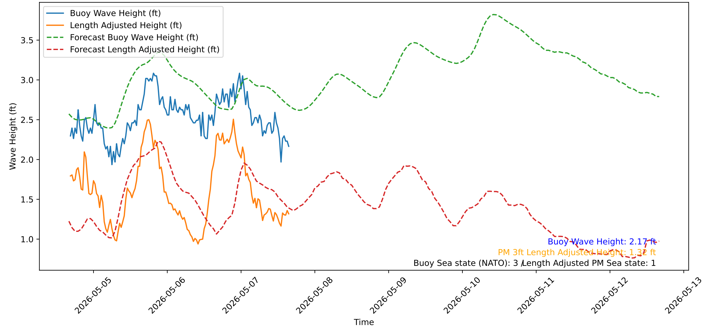
Wave Heights over Time for Red Beach at 2026-05-07 16:10:50
