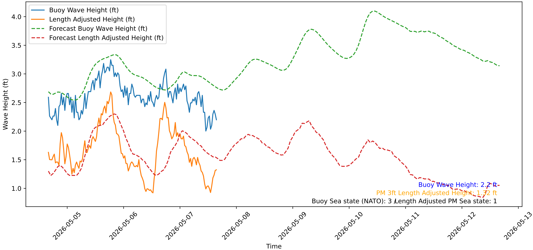
Wave Heights over Time for Oceanside Harbor at 2026-05-07 16:10:31
