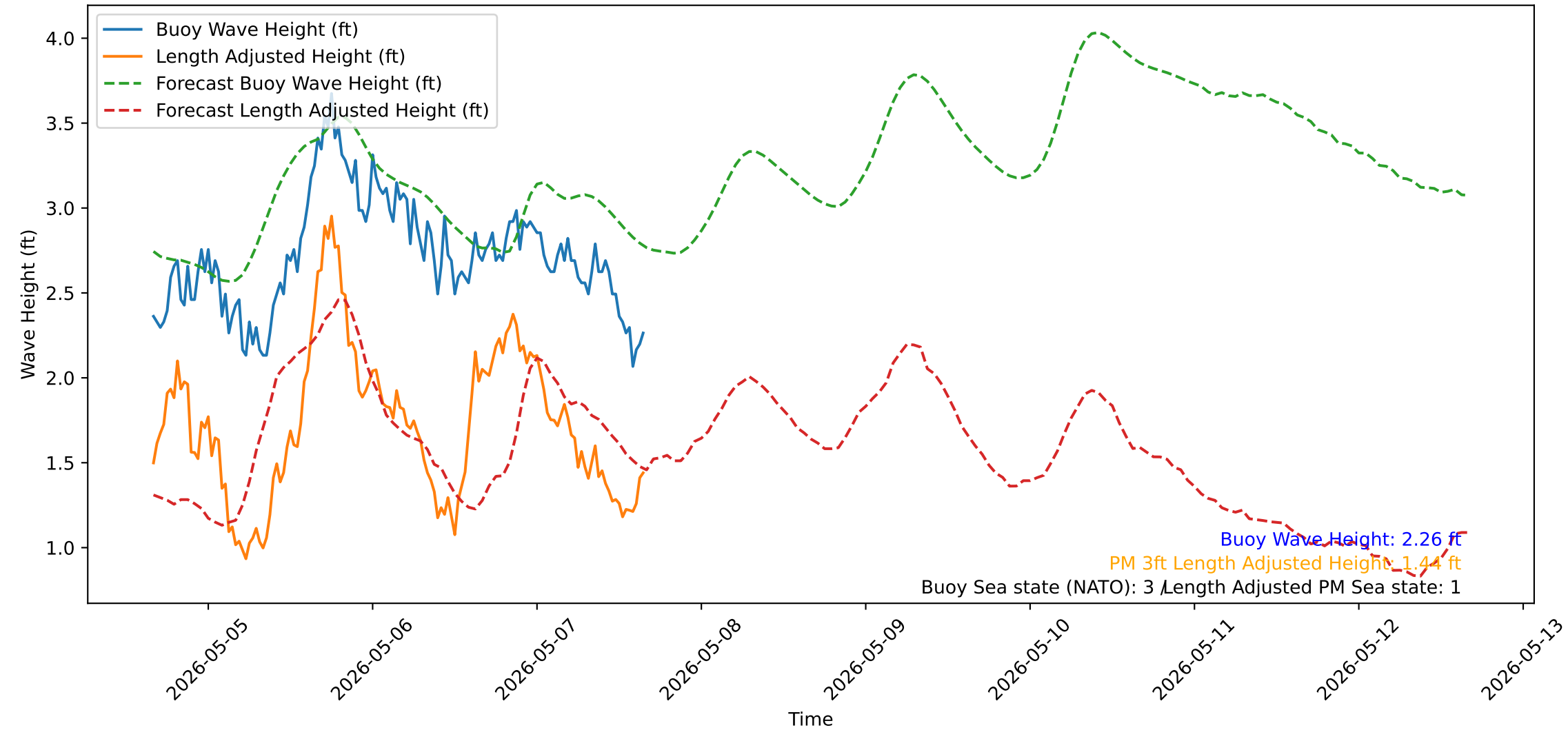
Wave Heights over Time for Green Beach at 2026-05-07 16:11:12
