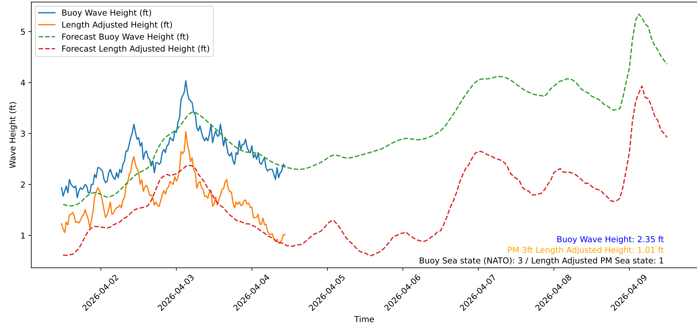
Wave Heights over Time for Oceanside Harbor at 2026-04-04 11:30:32
