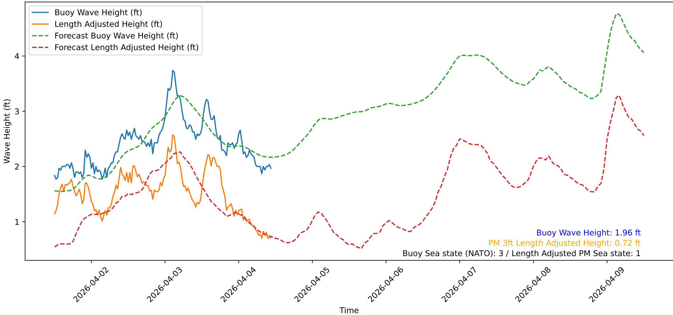
Wave Heights over Time for Red Beach at 2026-04-04 11:30:47
