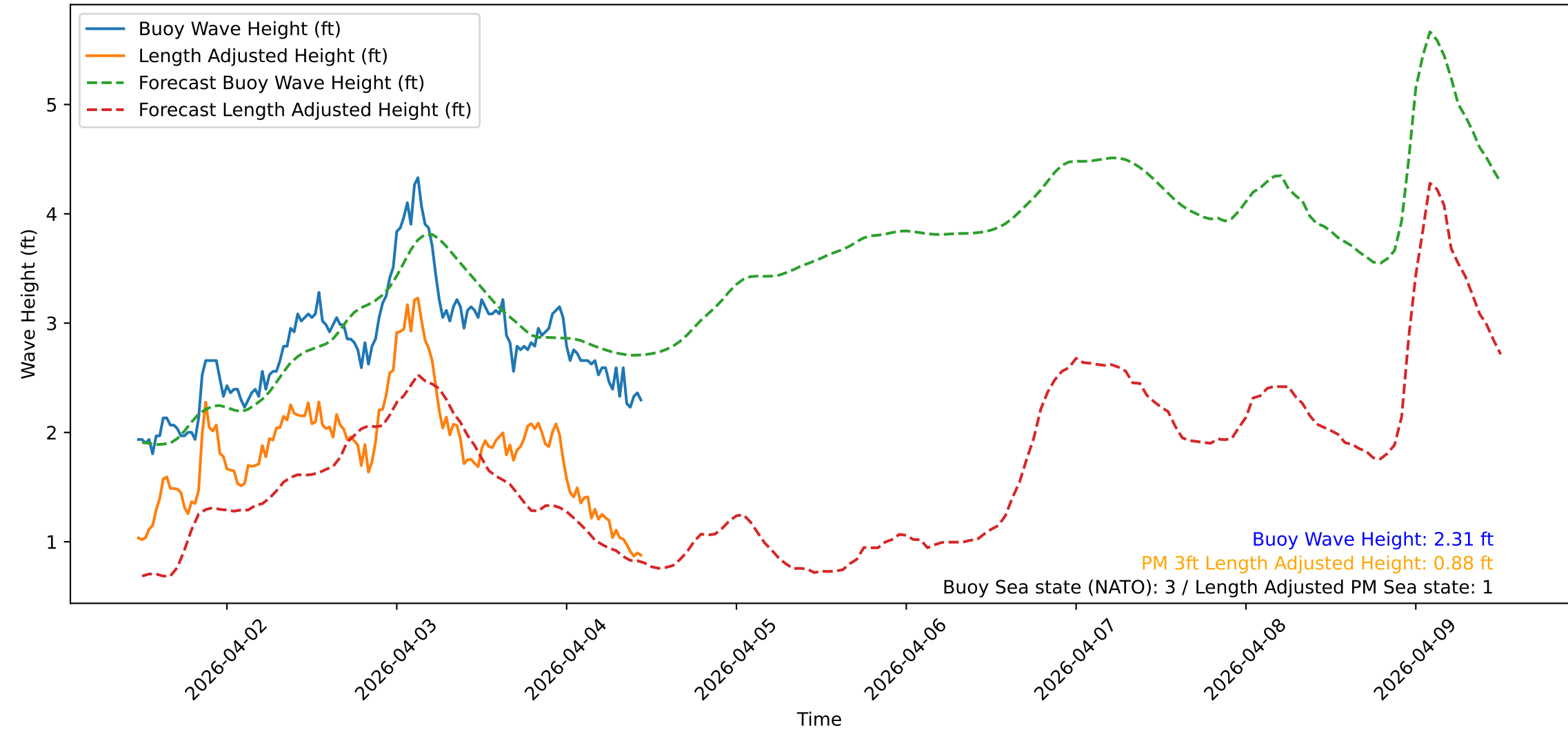
Wave Heights over Time for Green Beach at 2026-04-04 11:31:10
